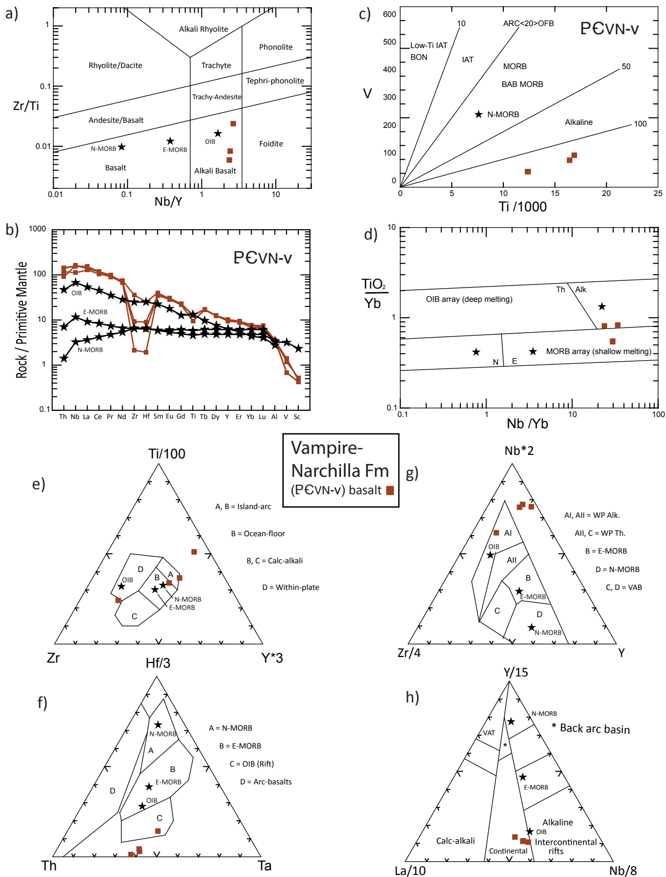
Figure 53. Geochemical and tectonic discriminate diagrams for volcanic rocks of the Vampire-Narchilla Formation: (a) Zr/TiO 2 -Nb/Y diagram of Winchester and Floyd (1977), as modified by Pearce (1996); (b) Primitive mantle-normalized multi-element diagram; (c) Ti/V diagram of Shervais (1982); (d) TiO 2 /Yb-Nb/Yb diagram of Pearce (2008); (e) Zr-Ti-Y diagram of Pearce and Cann (1973) for tholeiitic basalt; (f) Th-Hf-Ta diagram of Wood (1980); (g) Zr-Nb-Y diagram of the Meschede (1986); (h) La-Y-Nb diagram of Cabanis and Lecolle (1989) for basalt.
