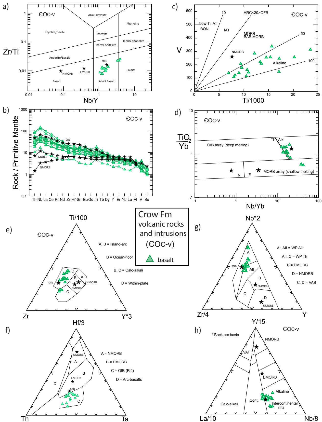
Figure 54. Geochemical and tectonic discriminate diagrams for volcanic and intrusive rocks of the Crow Formation: (a) Zr/TiO 2 -Nb/Y diagram of Winchester and Floyd (1977), as modified by Pearce (1996); (b) Primitive mantle-normalized multi-element diagram; (c) Ti/V diagram of Shervais (1982); (d) TiO 2 /Yb-Nb/Y diagram of Pearce (2008); (e) Zr-Ti-Y diagram of Pearce and Cann (1973) for tholeiitic basalt; (f) Th-Hf-Ta diagram of Wood (1980); (g) Zr-Nb-Y diagram of the Meschede (1986); (h) La-Y-Nb diagram of Cabanis and Lecolle (1989) for basalt.
