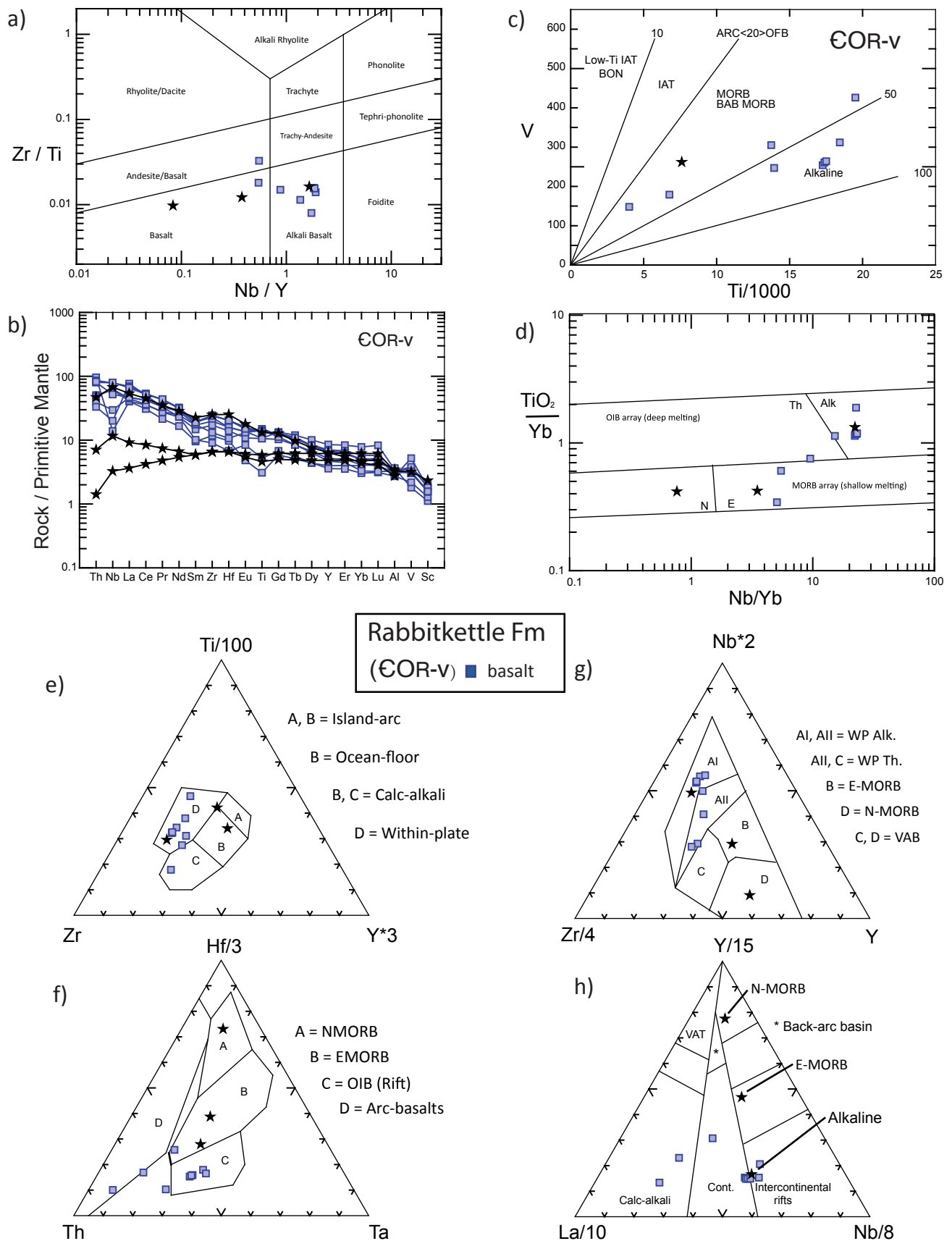
Figure 55. Geochemical and tectonic discriminate diagrams for volcanic rocks of the Rabbitkettle Formation:
