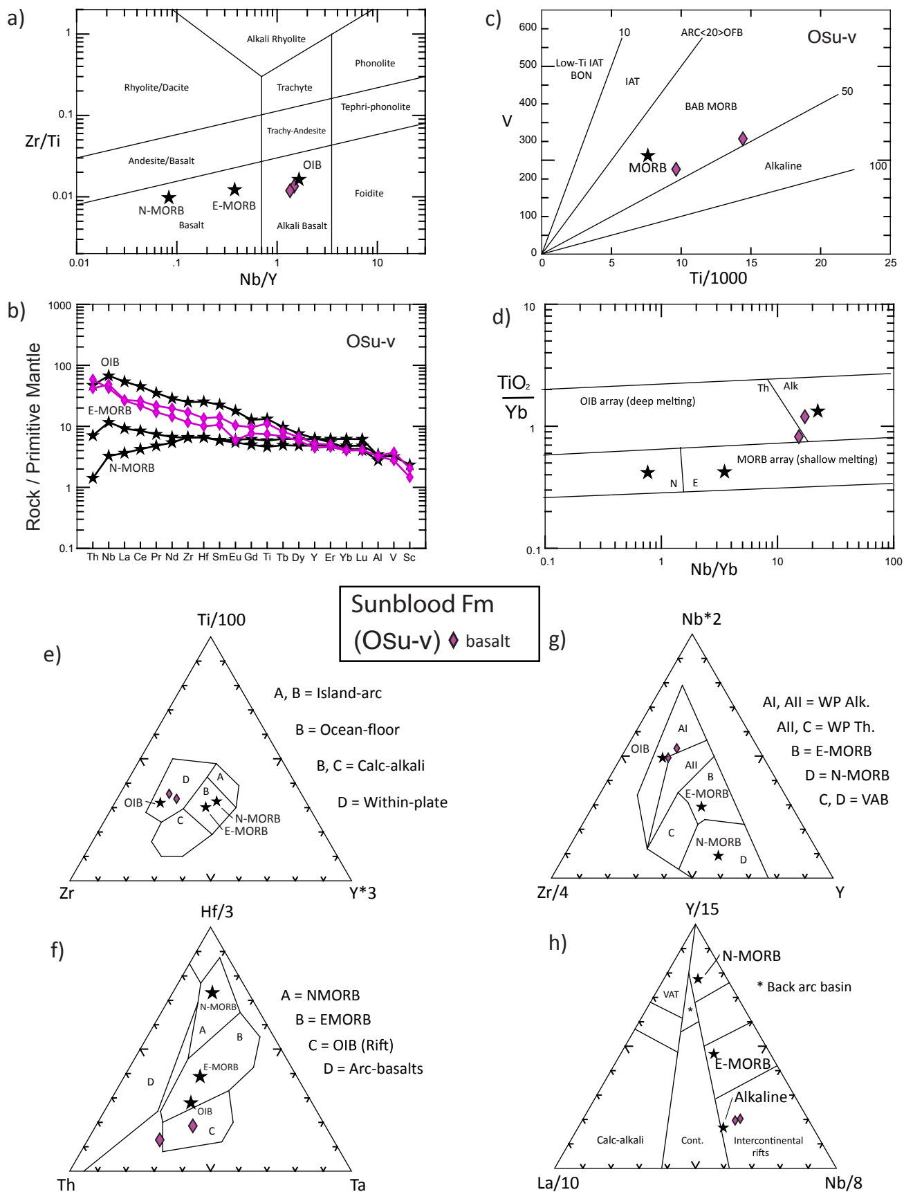
Figure XX. Geochemical and tectonic discriminate diagrams for volcanic rocks of the Sunblood Formation: (a) Zr/TiO 2 -Nb/Y diagram of Winchester and Floyd (1977), as modified by Pierce (1996); (b) Primitive mantle-normalized multi-element diagram; (c) Ti/V diagram of Shervais (1982); (d) TiO 2 /Yb-Nb/Y diagram of Pierce (2008); (e) Zr-Ti-Y diagram of Pierce and Cann (1973) for tholeiitic basalt; (f) Th-Hf-Ta diagram of Wood (1980); (g) Zr-Nb-Y diagram of the Meschede (1986); (h) La-Y-Nb diagram of Cabanis and Lecolle (1989) for basalt.
