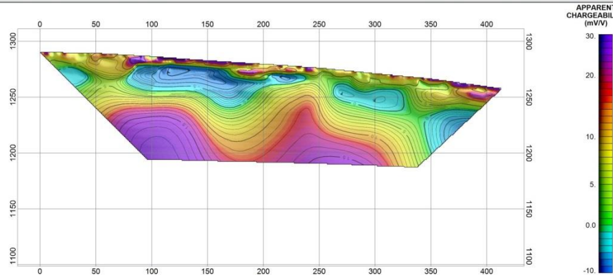
Inverted Chargeability
