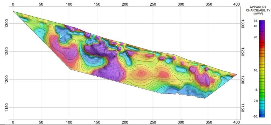
Inverted Chargeability
