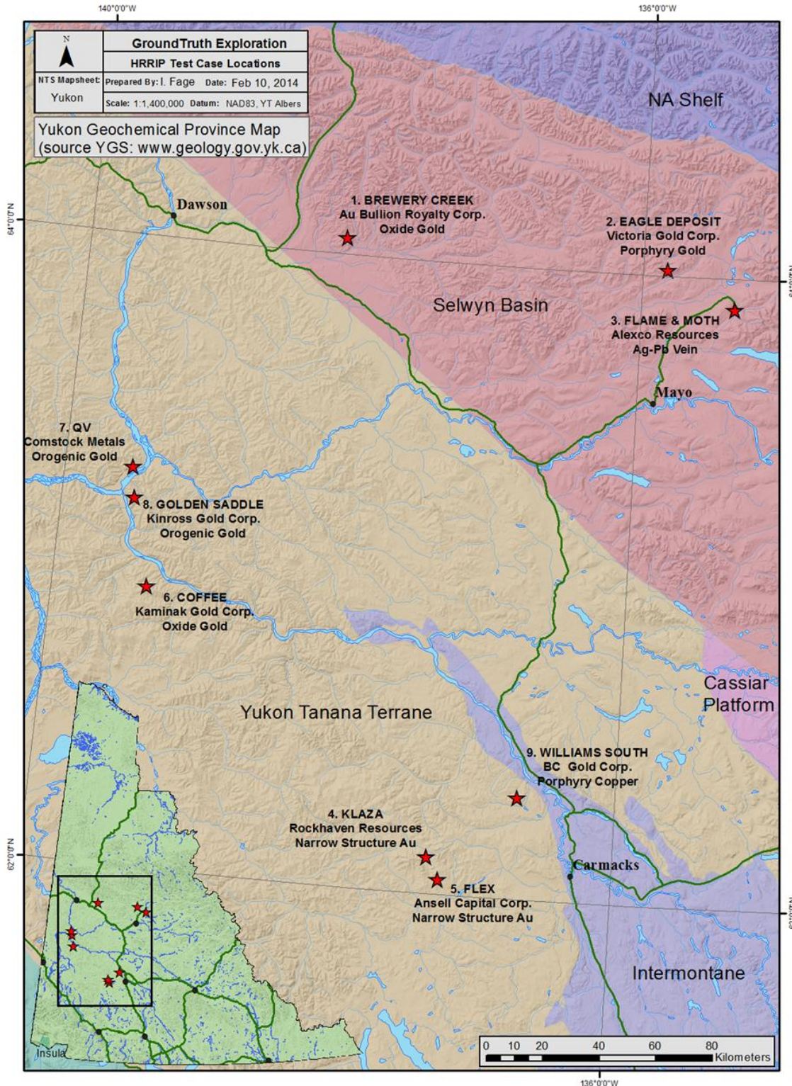
Figure 7. Locations of the 9 case studies overlain on the Yukon terrane map.
