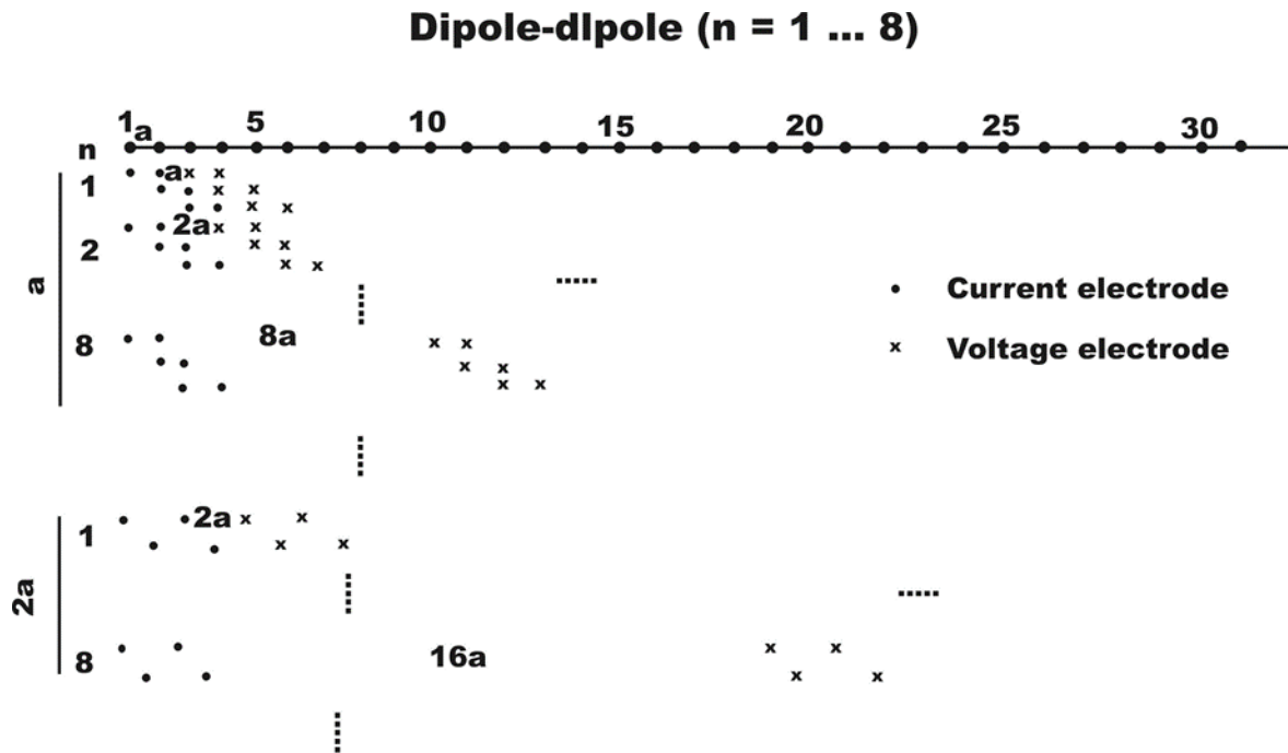
Figure 5. Example of current and voltage electrode locations for dipole array.
