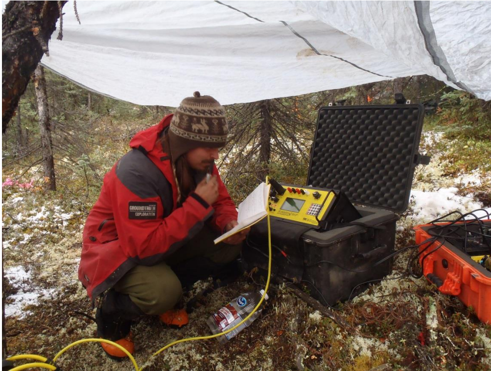
Figure CS9-2. Chad Cote operating Supersting on CS-9, Williams South project.
