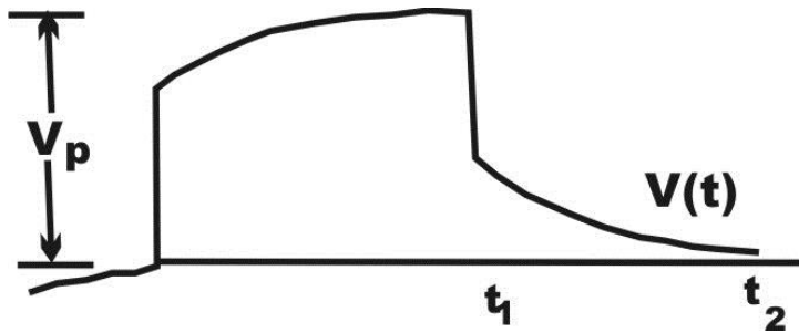
Figure 9. Schematic of IP decay parameters (from Sumner, 1976).
