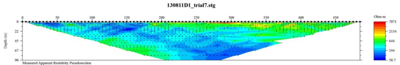
Figure 6. Example of a resistivity pseudosection for a dipole-dipole array.
