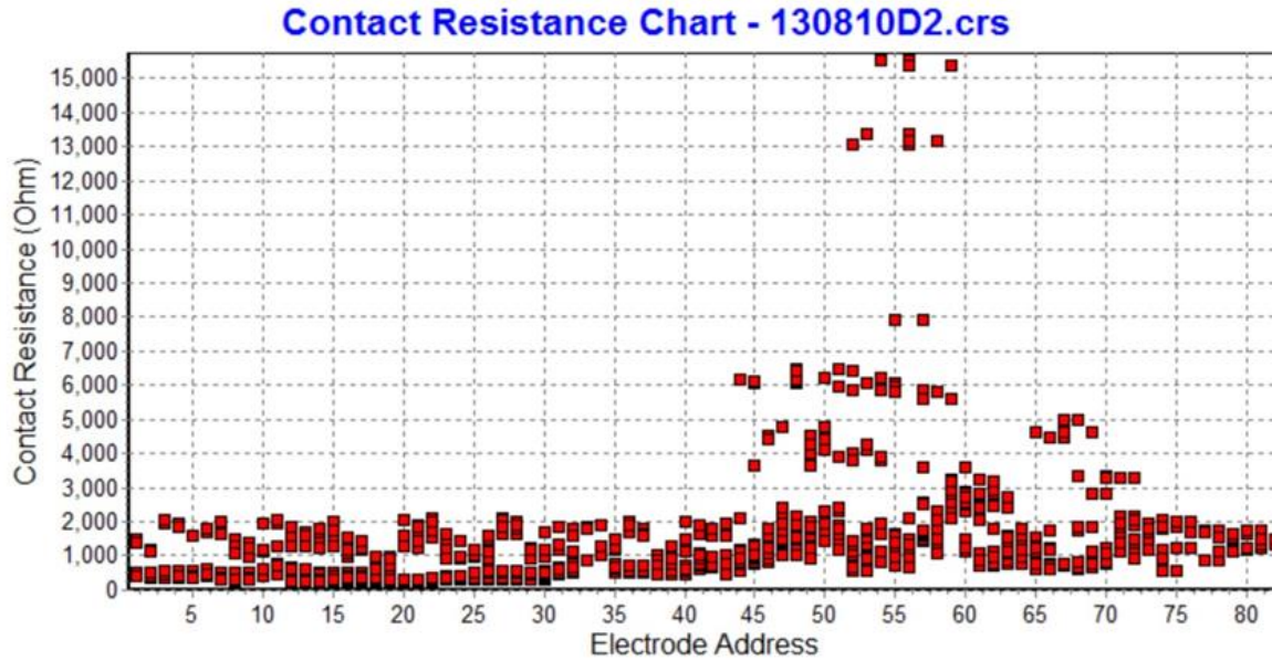
Figure 3. Example of contact resistance for an 84 electrode system.
