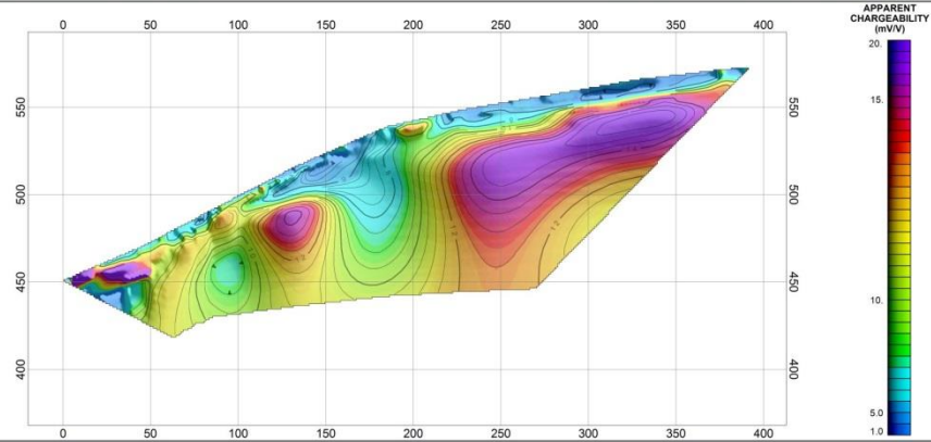
Inverted Chargeability
