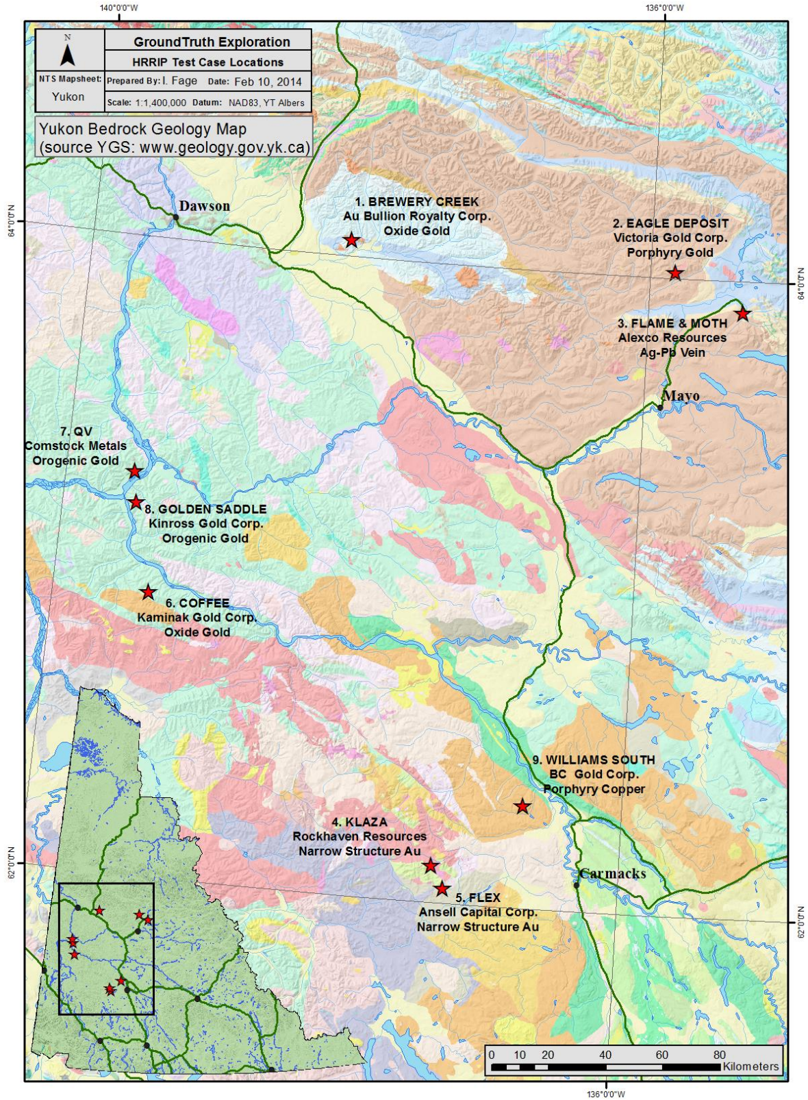
Figure 8. Locations of the 9 case studies overlain on the Yukon regional geology map.
