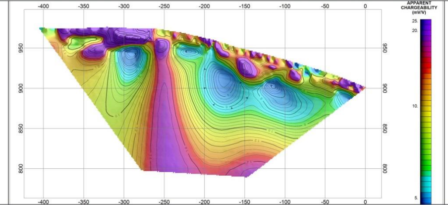
Inverted Chargeability
