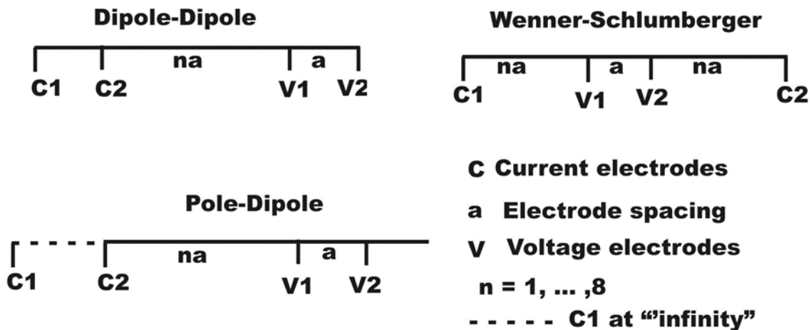
Figure 1. Common electrode arrays.
