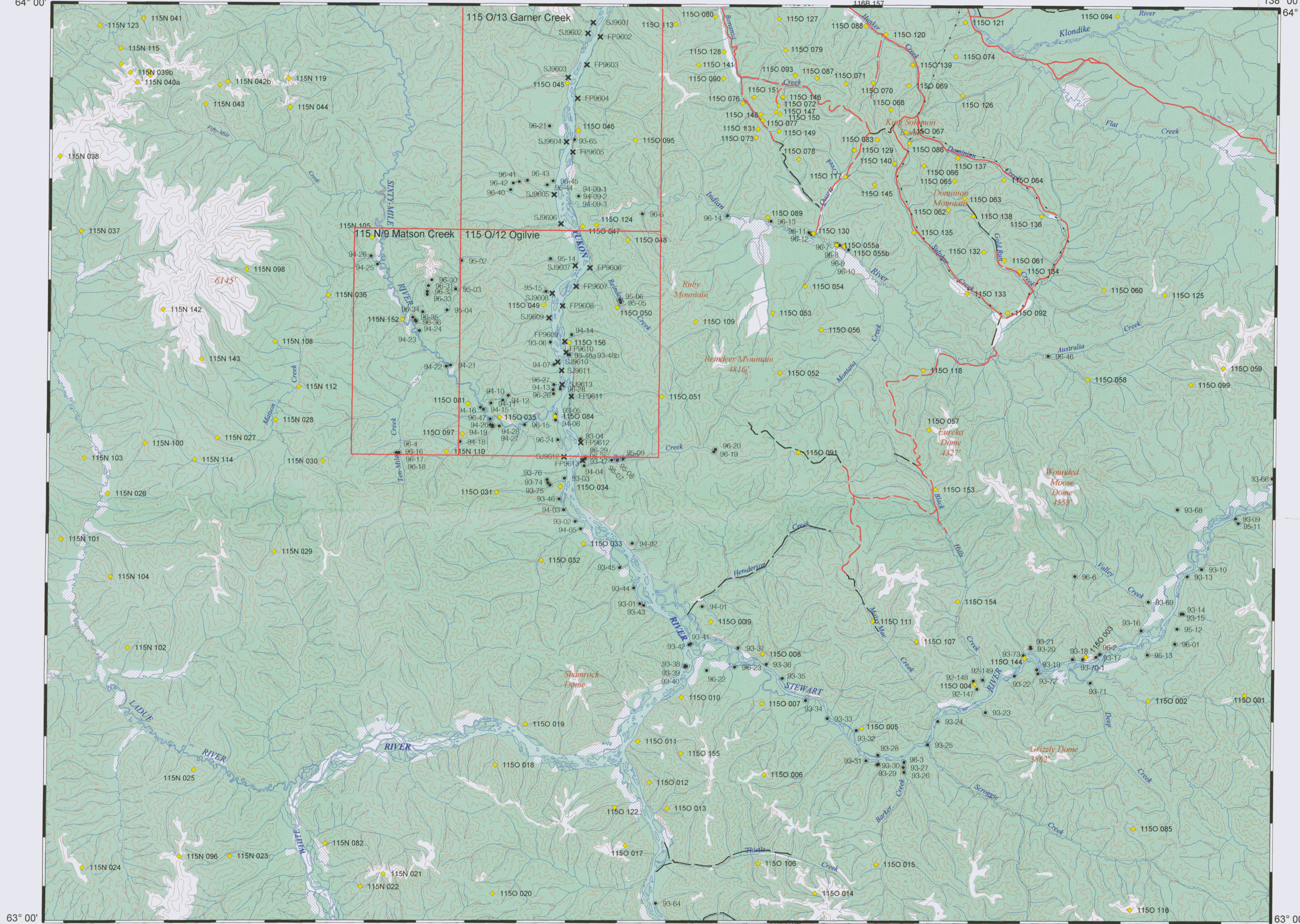
Figure 2. Stewart River Placer Project compilation map. This map accompanies Open File 1998-1: Morison, S.R., Mougeot, C. and Walton, L., 1998. Surficial geology and sedimentology of Garner, Ogilvie and Matson Creek map areas, western Yukon Territory (115 O/13, 115 O/12 and 115 N/9- east half), Exploration and Geological Services Division, Yukon Region, Indian and Northern Affairs Canada, 87p.
