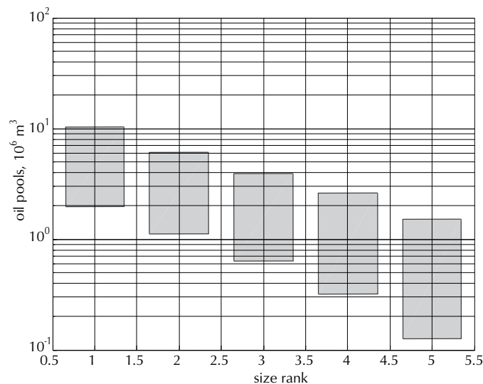
Figure 32. Predicted accumulation size by rank. The predicted pool sizes are obtained using order statistics and conditioning the accumulation-size distribution against the number of expected pools, as shown in Table 25.
