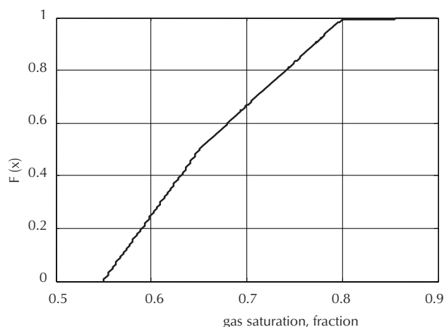
Figure 26. Example play parameter input distributions for select accumulation size equation input variables, specifically the accumulation area of closure, net pay, reservoir porosity and hydrocarbon saturation, for Play 1, in the Cretaceous sandstones. Complete sets of input play parameters are presented in Tables 4, 8, 12, 16, 20, 24, 28, 32, 36, 40, 44, 48, 52, 56, and 60, which are reported at the 100th, 50th, 1st and 0 percentiles of the input play parameter distributions. F(x) = cumulative frequency
