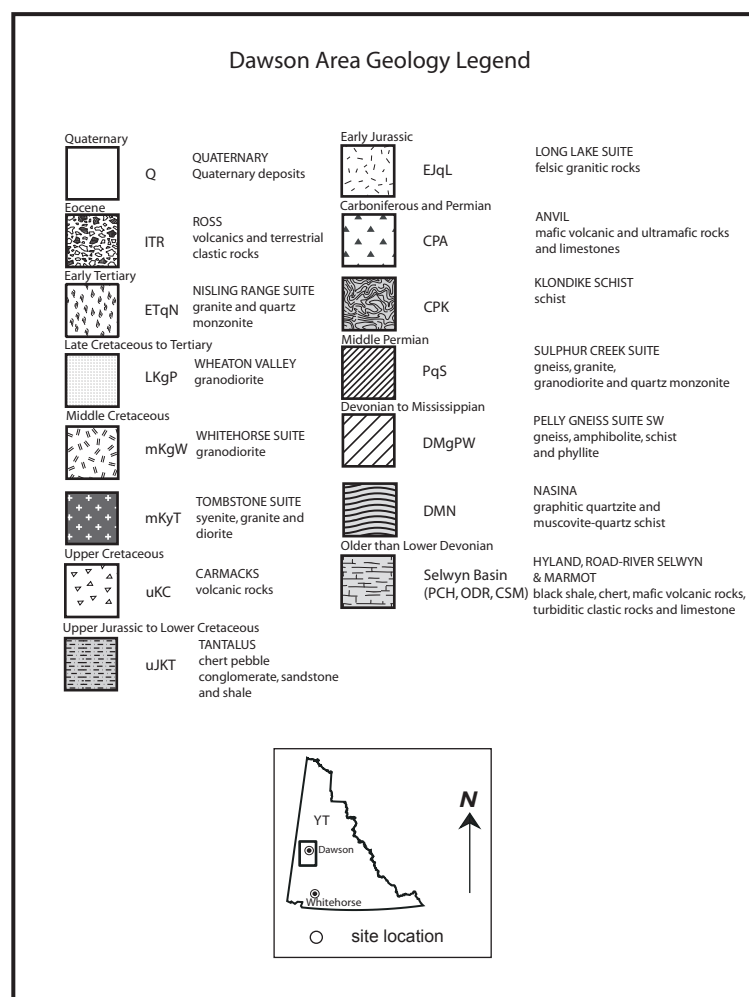
Figure 4a. Legend for Dawson area geology map at right, with study sites indicated, (Gordey and Makepeace, 2003).
