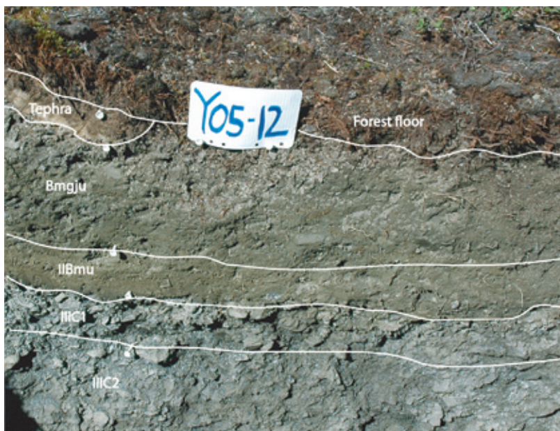
Figure 28. Soil profile at Clip 2 on the Clip property, with horizons indicated.
