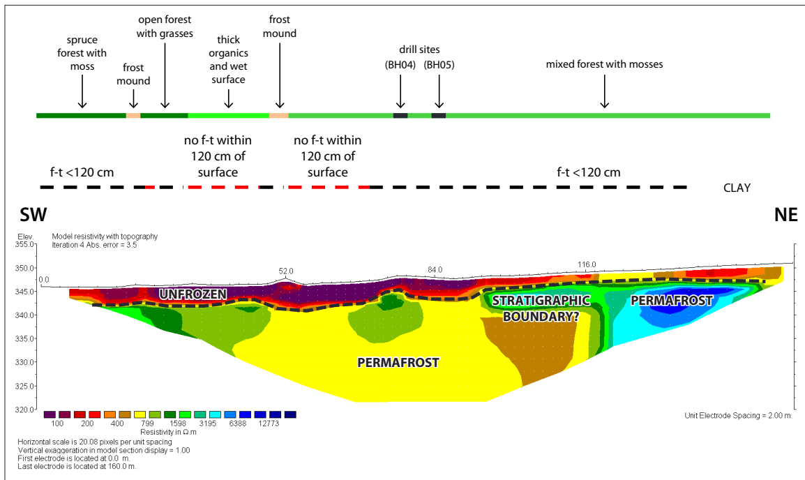
Figure 62. ERT profile DC_ERT06, which is 160 m long and runs southwest to northeast approximately 100 m west and 15 m upslope of DC_ERT05 (see Figure 60 for location). The profile has a maximum penetration depth of ~25 m. Likely areas of permafrost are outlined by black dashed lines; f-t = frost table.
