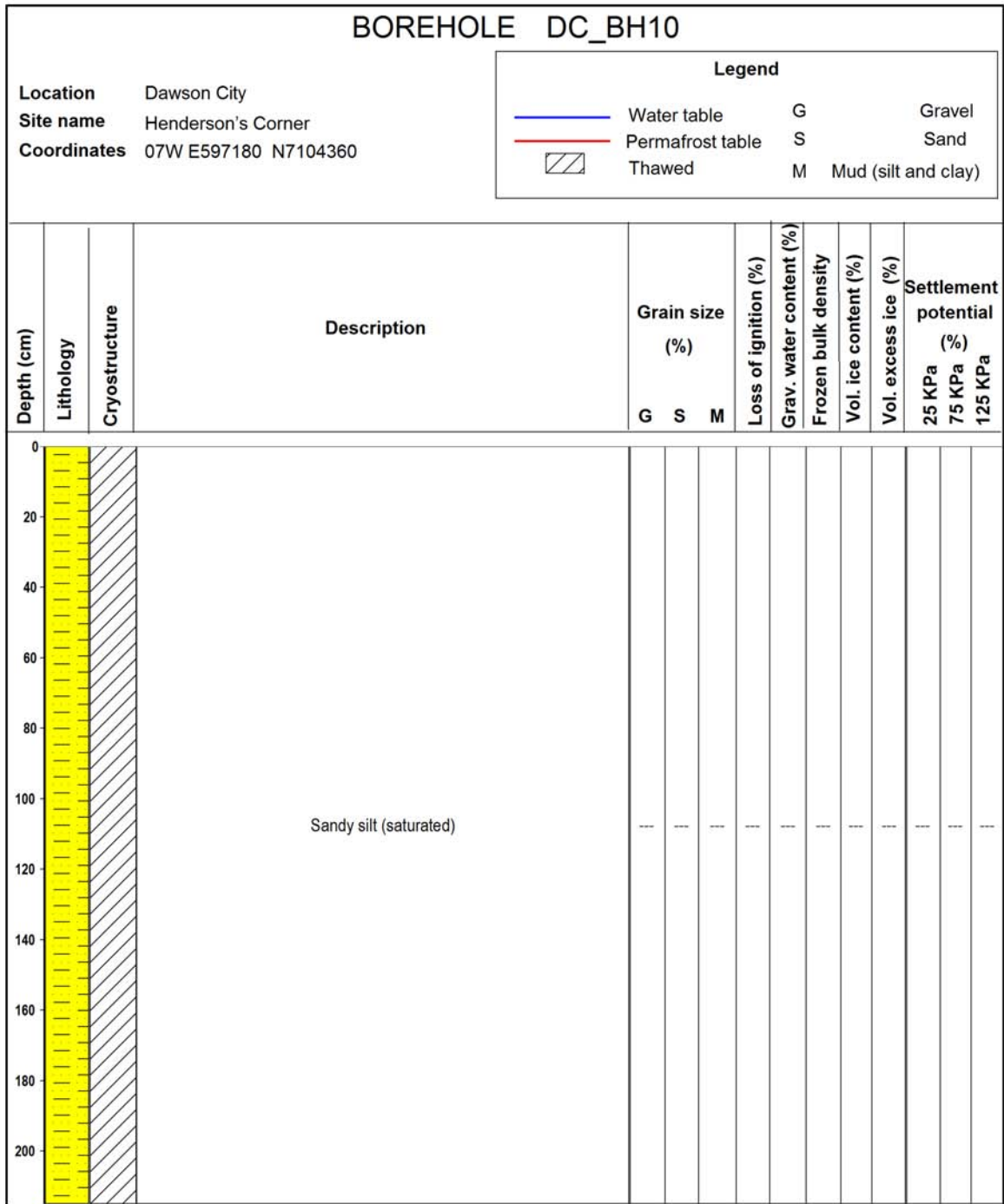
Figure B10. Borehole log for borehole DC_BH10, from the Henderson's Corner case study site (see Figure 68 in the main body of this report for location).
