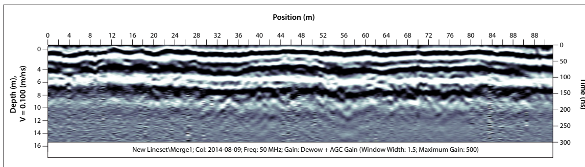
Figure 53. GPR profile DC_GPR01 from the West Dawson case study site, showing a strong, undulating layer from 0-1 m depth, which may correspond to the top of the permafrost table.
