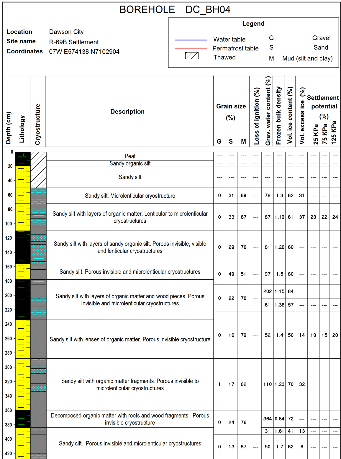
Figure B4. Borehole log for borehole DC_BH04, from the R-69B case study site (see Figure 60 in the main body of this report for location).
