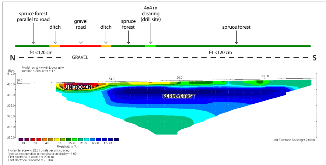
Figure 51. ERT profile DC_ERT01b is 160 m long and runs north to south, and parallel to DC_ERT1a (see Figure 50 for location). The profile has a maximum penetration depth of ~25 m. Likely areas of permafrost are outlined by black dashed lines; f-t = frost table.
