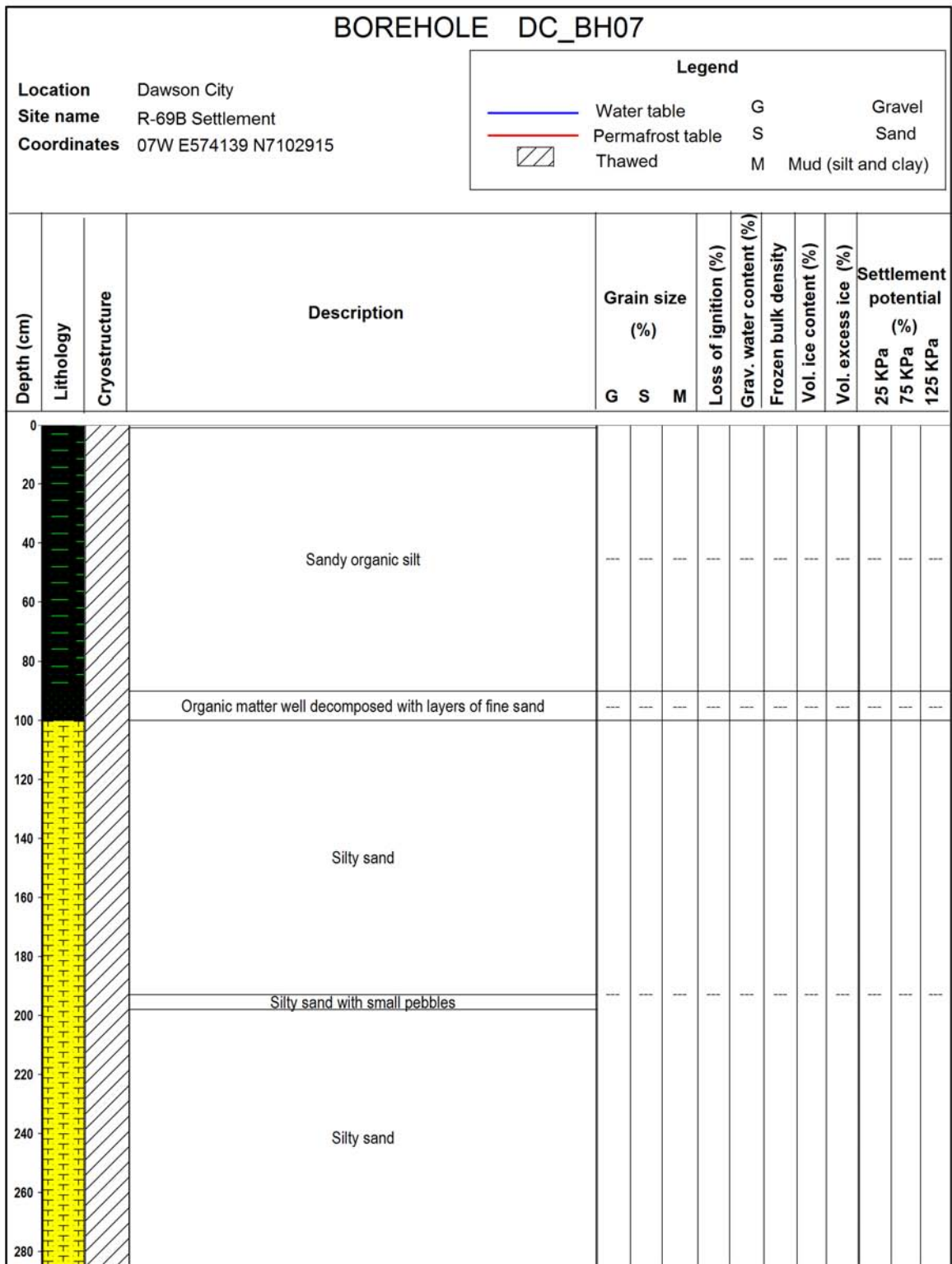
Figure B7. Borehole log for borehole DC_BH07, from the R-69B case study site (see Figure 60 in the main body of this report for location).
