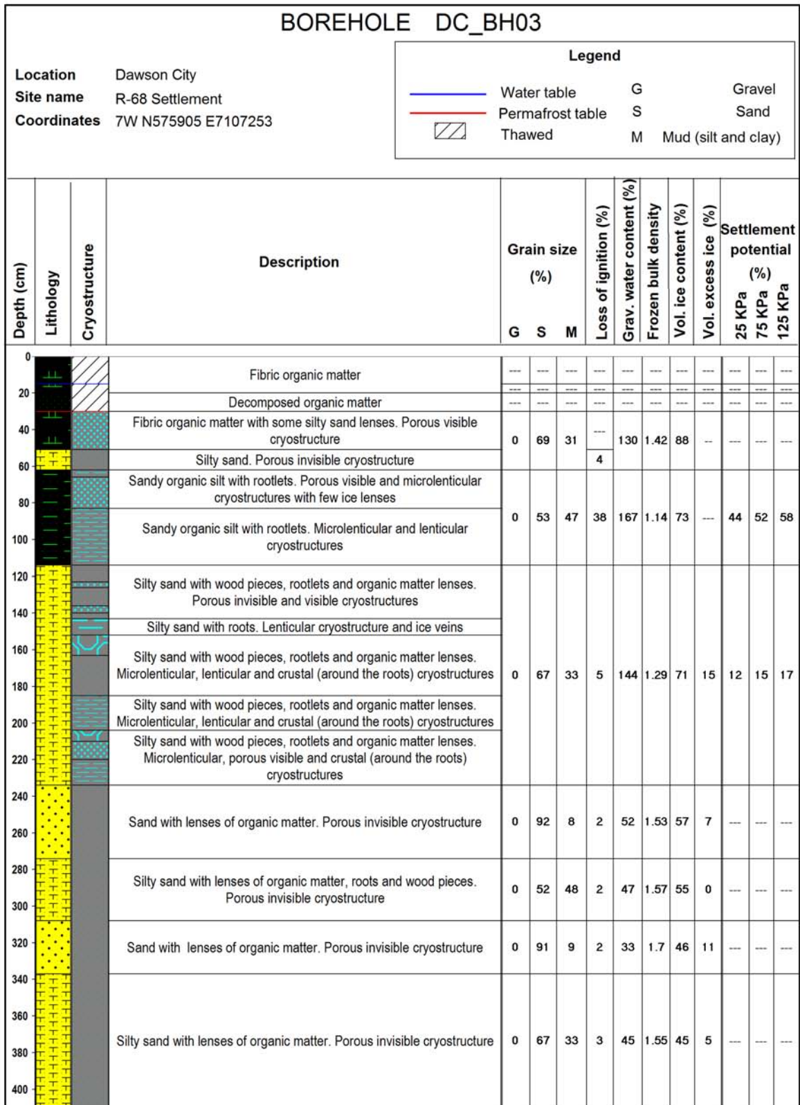
Figure B3. Borehole log for borehole DC_BH03, from the R-68B case study site (see Figure 56 in the main body of this report for location).
