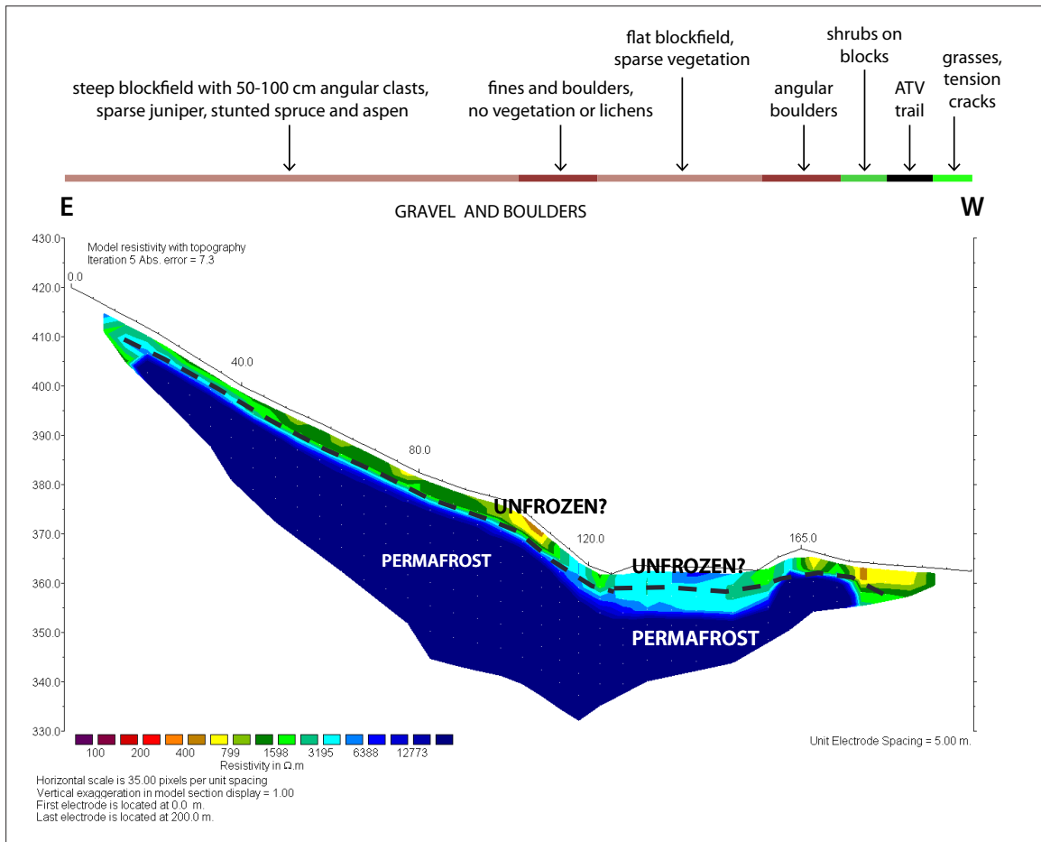
Figure 44. ERT profile for the Moosehide Slide (200 m long) was run down the lobate mass at the foot of the steep, unstable headwall of the slide. The profile has a maximum penetration depth of about 30 m. Likely areas of permafrost are outlined by black dashed lines.
