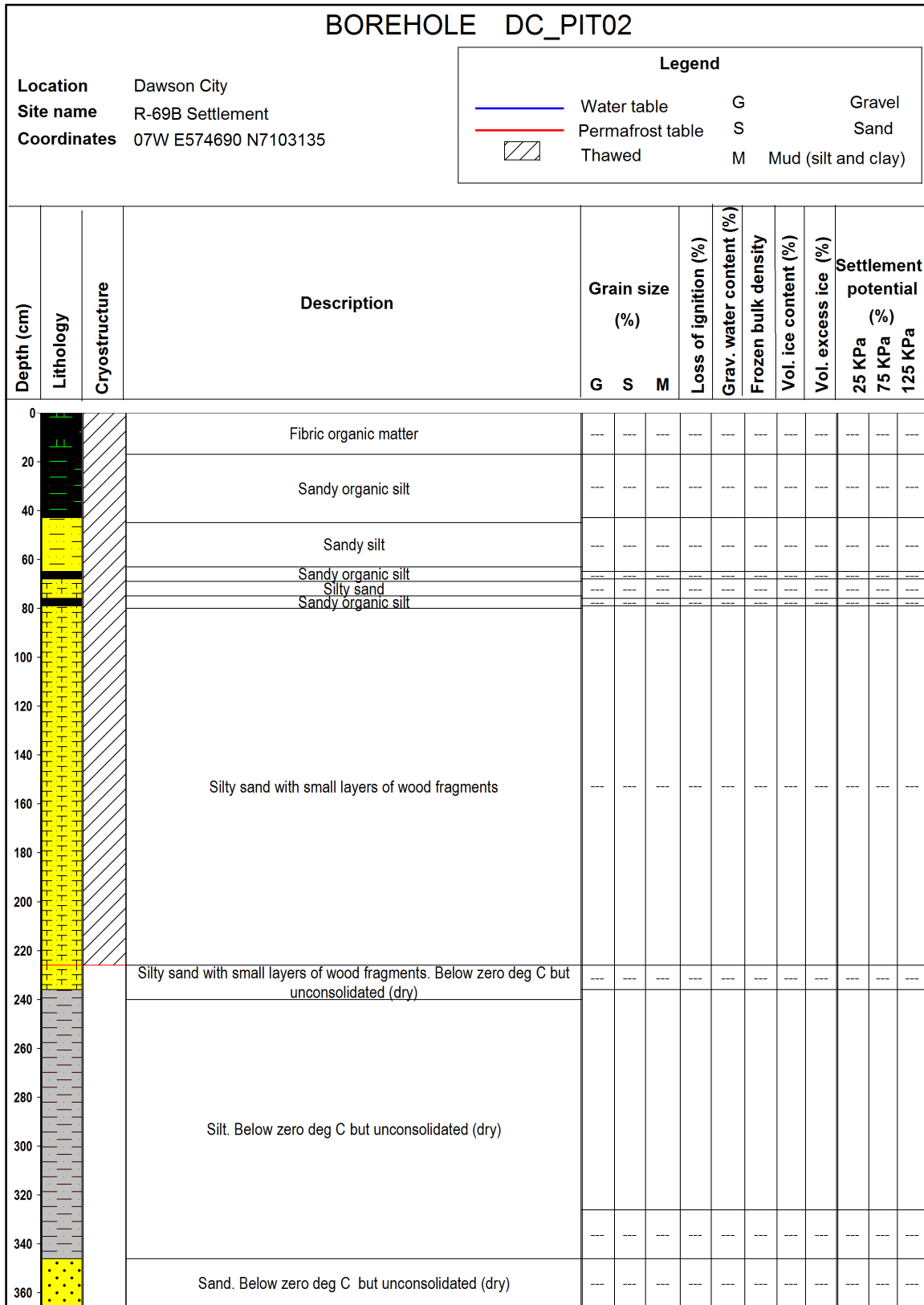
Figure B12. Log for soil pit DC_PIT02, from the R-69B case study site (see Figure 60 in the main body of this report for location).
