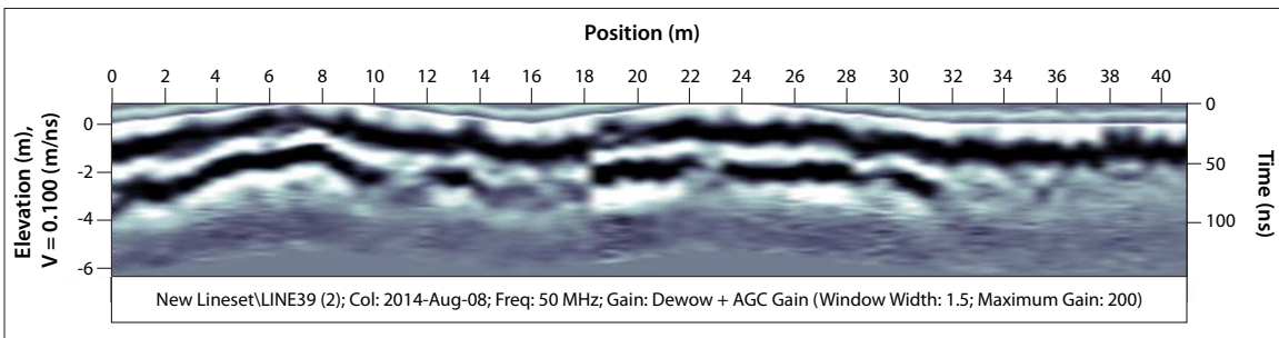
Figure 65. GPR profile DC_GPR05 from the R-69B case study site, showing a strong reflection near surface (between 0.2 and 0.5 m), likely corresponding to the top of the permafrost table.
