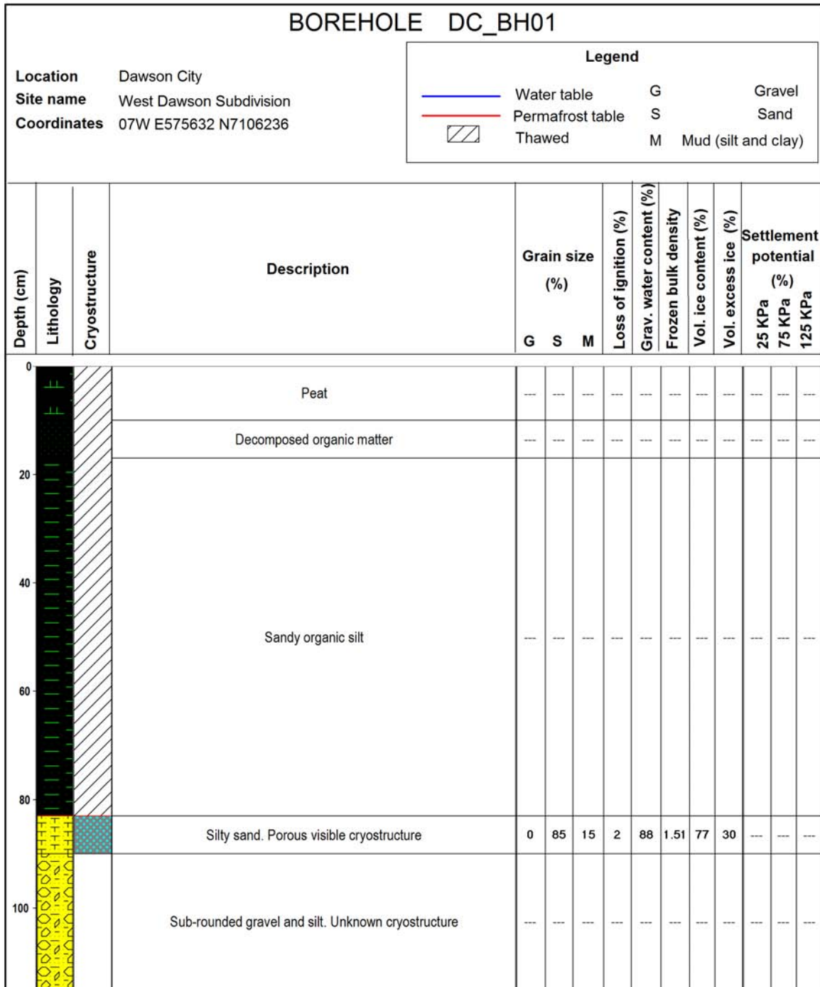
Figure B1. Borehole log for borehole DC_BH01, from the West Dawson case study site (see Figure 50 in the main body of this report for location).
