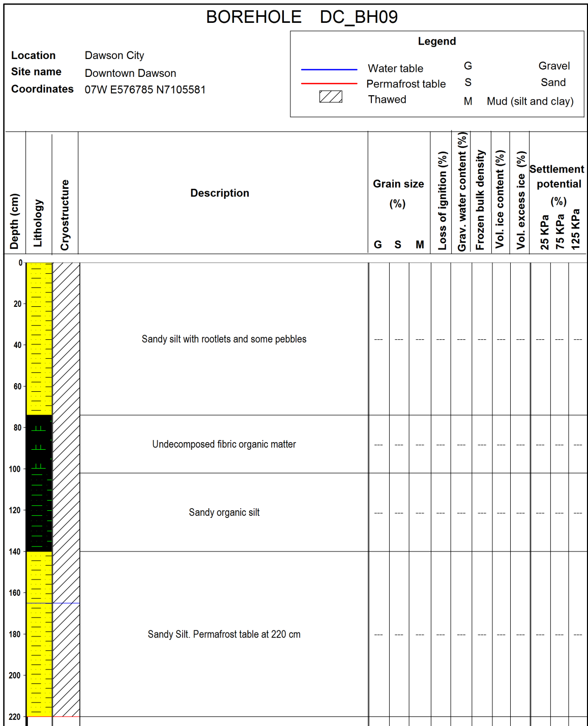
Figure B9. Borehole log for borehole DC_BH09, from the downtown Dawson case study site (see Figure 66 in the main body of this report for location).
