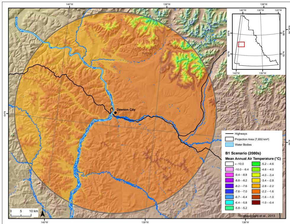
Figure D8. Mean annual air temperature for the Dawson area for 2080, projected using the B1 scenario.
