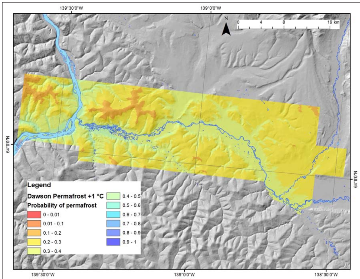
Figure 69. Projected permafrost probability for the Dawson region under an increase in mean annual air temperature of 1°C.
