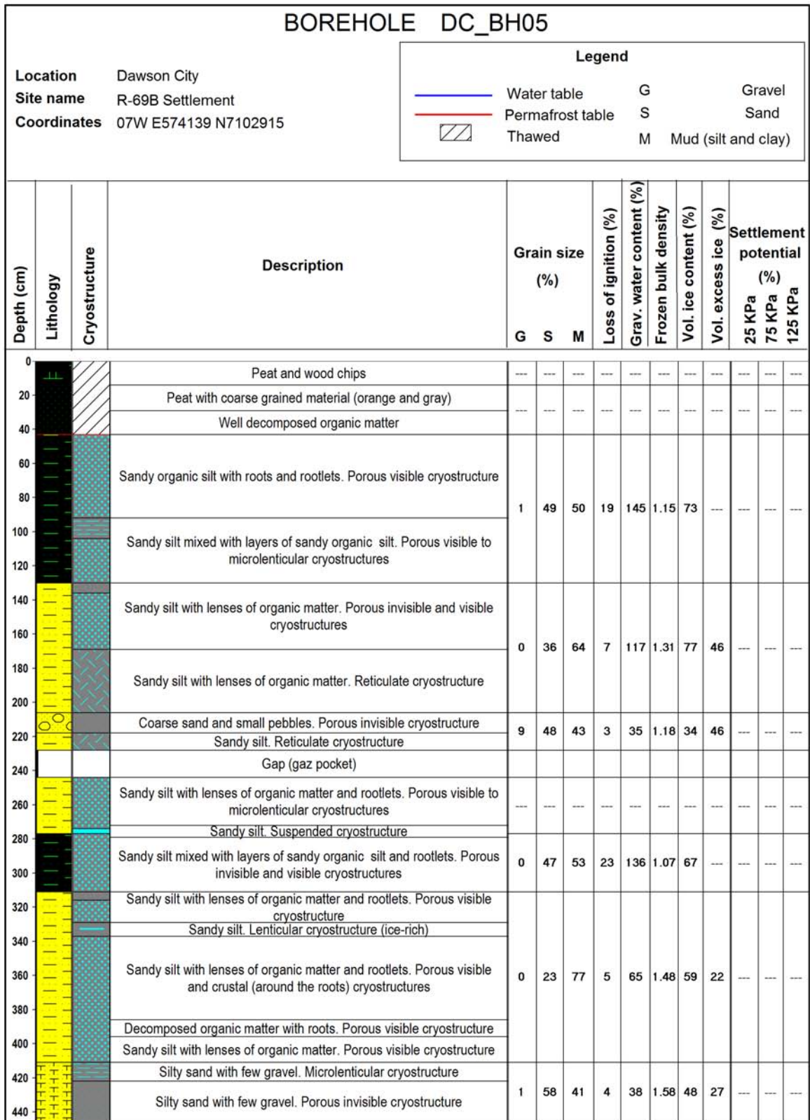
Figure B5. Borehole log for borehole DC_BH05, from the R-69B case study site (see Figure 60 in the main body of this report for location).
