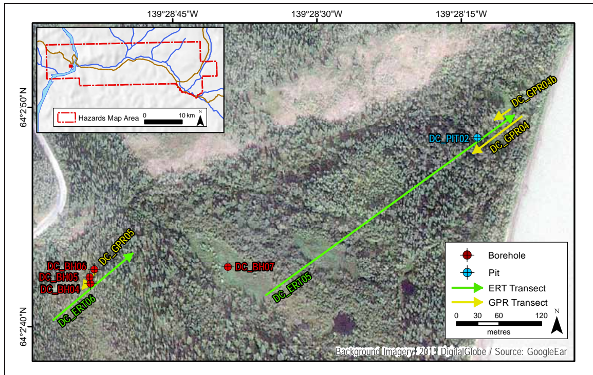
Figure 60. Map illustrating locations of detailed site investigations for the R-69B case study site. Refer to Figure 49 for case study location.
