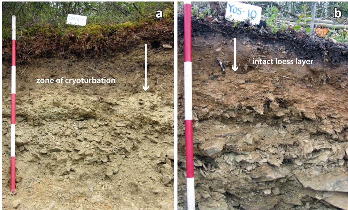
Figure 31. (a) A north-facing hillslope with a well-mixed soil profile; and (b) a south-facing hillslope with the loess layer intact. Coloured bands on rod are 25 cm.
