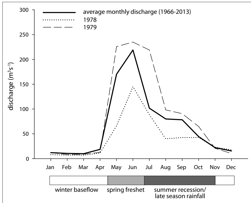
Figure 6. Average monthly discharge hydrograph for the Klondike River above Bonanza Creek (heavy solid line). Also shown are hydrographs for the years 1978 (dotted line) and 1979 (long-dashed line), demonstrating low and high measured peak discharge, respectively (Water Survey of Canada, 2015).
