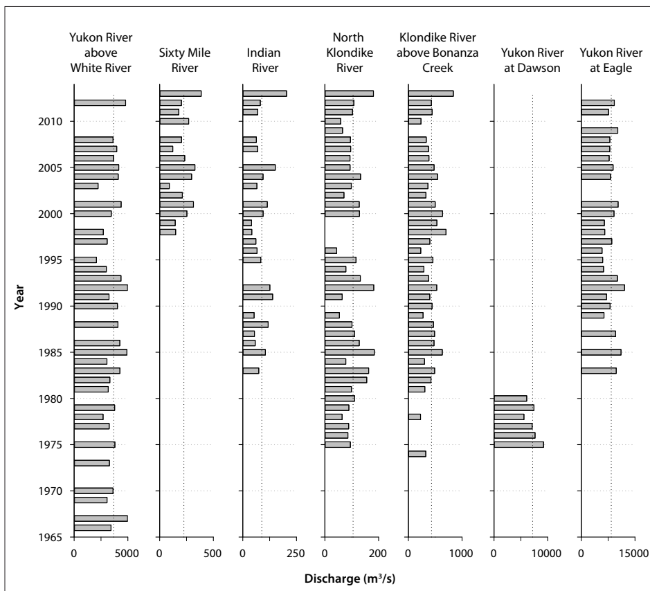
Figure 9. Peak discharge at WSC stations with multi-year records, arranged generally upstream (left) to downstream (right). Vertical, long-dashed lines indicate average peak discharge for each station for its period of record (Water Survey of Canada, 2015).
