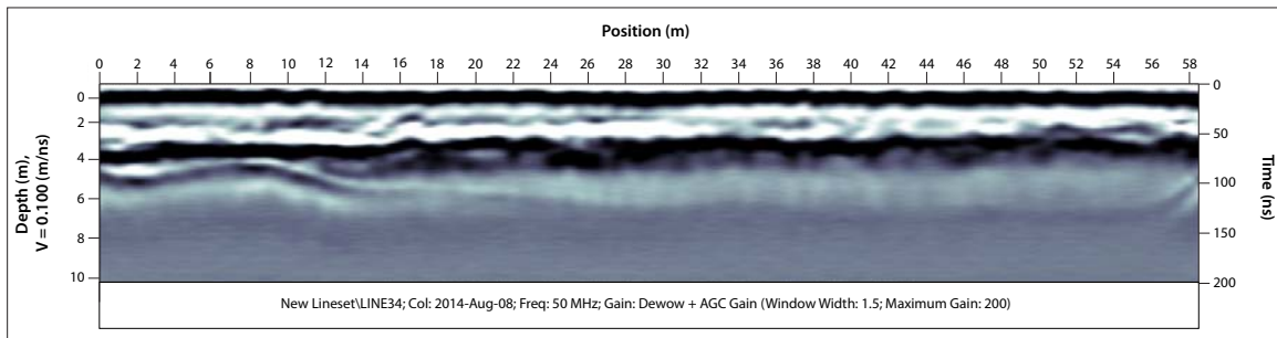
Figure 57. GPR profile DC_GPR03 from the C-3B case study site, showing a weak, undulating reflection at a depth of ~2 m, possibly corresponding to a gravelly layer.
