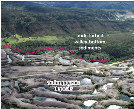
Figure 36. Aerial view of anthropogenic deposits (e.g., dredge tailings) and vegetated, undisturbed sediments in the Klondike River valley.
