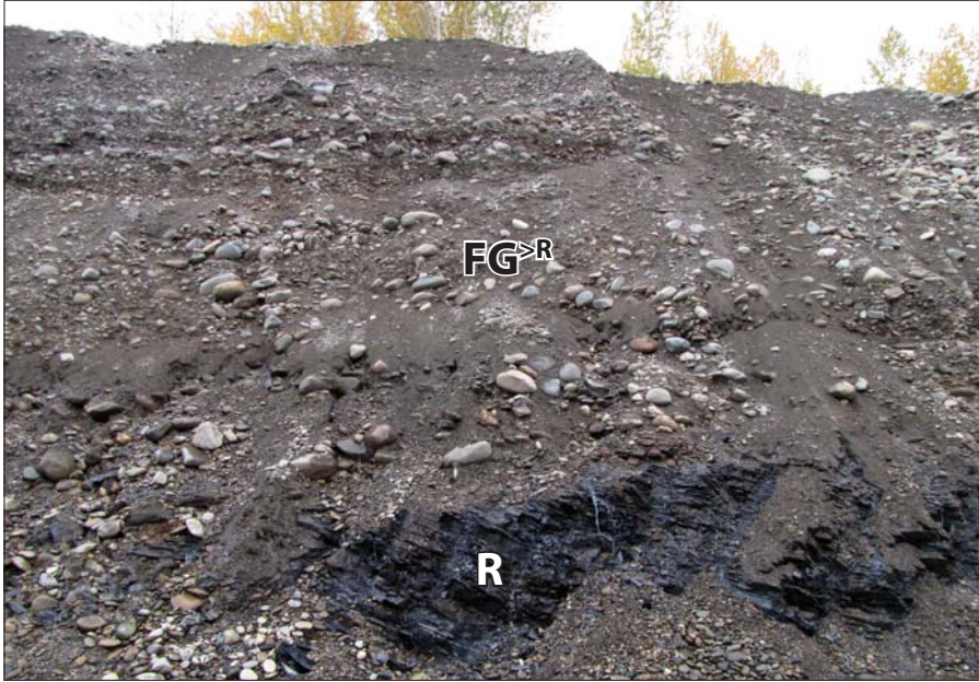
Figure 26. Pre-Reid glaciofluvial gravel ( FG^R ) deposited on bedrock (R) in the Klondike Valley and overlain by modern fluvial deposits.
