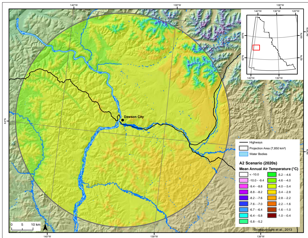
Figure D4. Mean annual air temperature for the Dawson area for 2020, projected using the A2 scenario.
