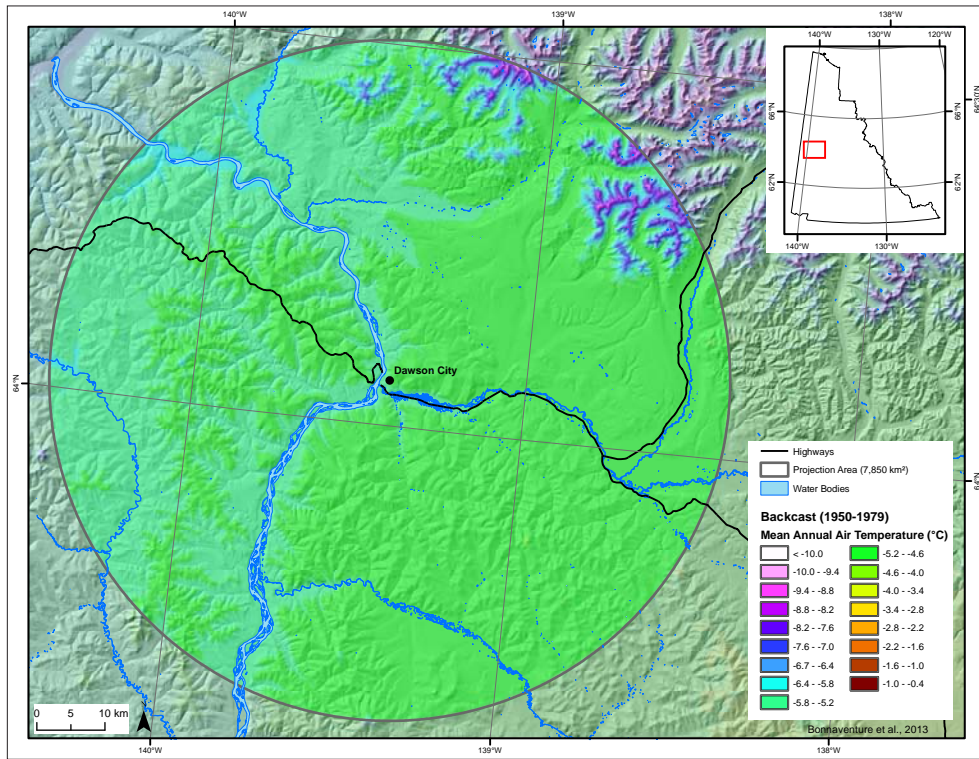
Figure D1. Mean annual air temperature for the Dawson area, backcasted for the 1950-1979 period.
