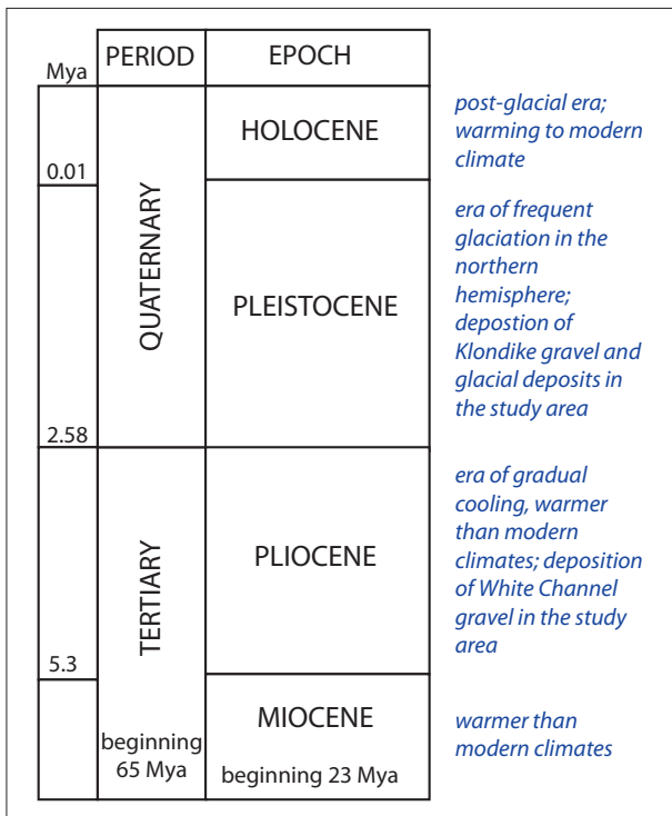
Figure 15. A simplified geologic timescale including those periods of rapid landscape evolution that occurred in the study area. Mya = millions years ago.
