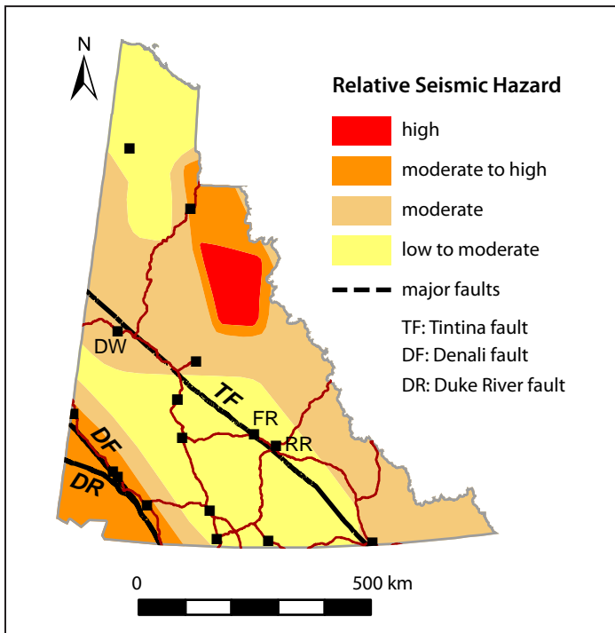
Figure 40. Simplified version of the National Building Code of Canada’s 2010 seismic hazard map (for spectral acceleration at a 0.2 second period (5 cycles per second)), illustrating the relative likelihood of experiencing earthquakes strong enough to potentially damage some, but not all, single family (one and two-story) dwellings (Natural Resources Canada, 2013). Dawson (DW) is located in the moderate hazard zone, where there is a 5-15% chance that significant damage will occur every 50 years. FR = Faro; RR = Ross River
