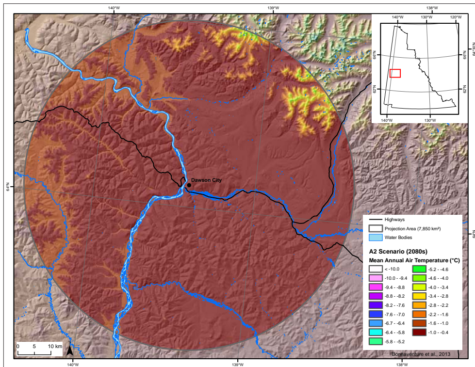
Figure D10. Mean annual air temperature for the Dawson area for 2080, projected using the A2 scenario.
