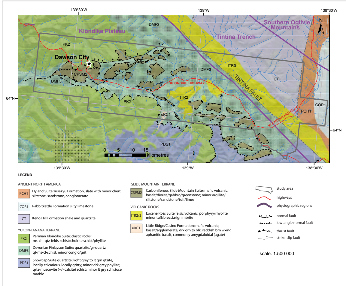
Figure 17. Simplified geology map of the study area including physiographic regions, faults, and simplified descriptions of the rocks of Slide Mountain and Yukon-Tanana terranes; ancient North America; and intrusive volcanics. From Colpron (2014).
