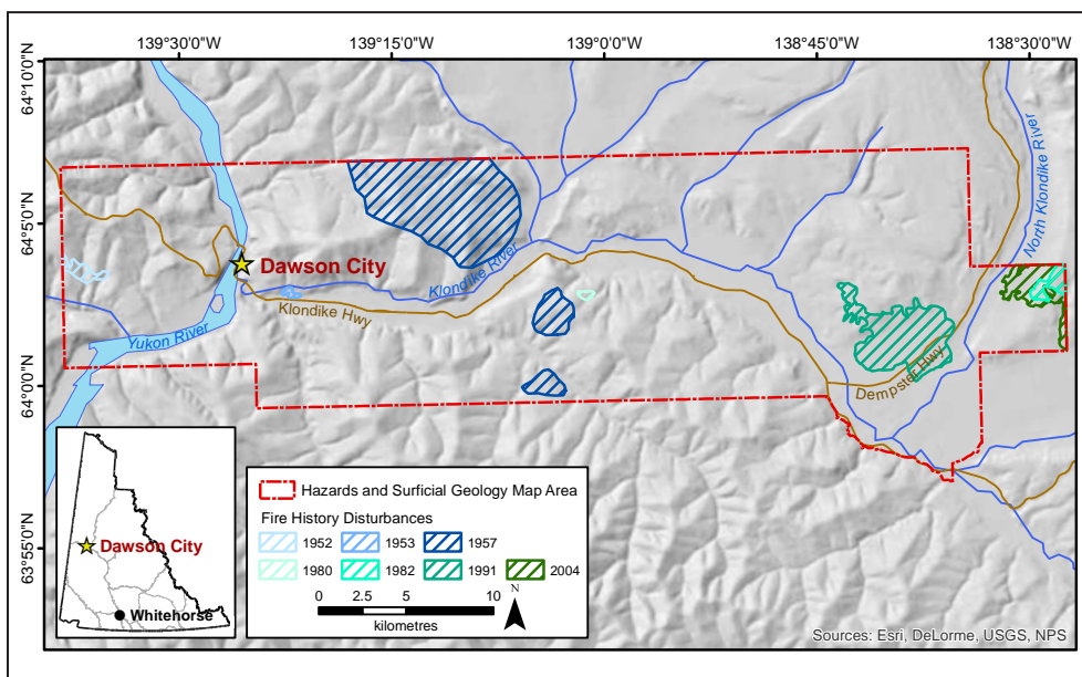
Figure 13. Fire history for the Dawson region, denoting the extents of notable fires in the study area. Fire history records provided by Government of Yukon.
