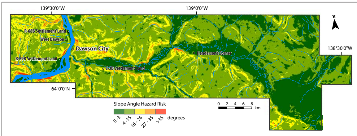
Figure 74. Hazard risk associated with slope angle in the Dawson region.
