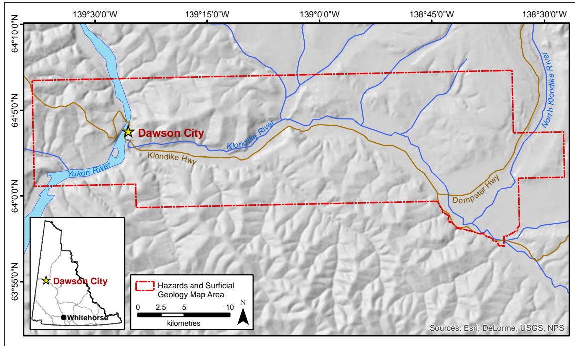
Figure 1. Location of study area, illustrating the surficial geology and hazards map footprints.
