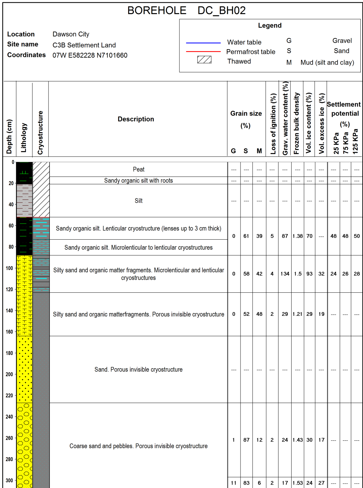
Figure B2. Borehole log for borehole DC_BH02, from the C-3B case study site (see Figure 54 in the main body of this report for location).
