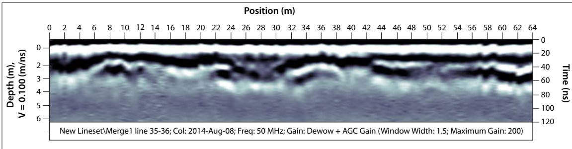
Figure 63. GPR profile DC_GPR04 from the R-69B case study site, showing a strong reflection at a depth of between 1 and 2.5 m, which may correspond to the top of the permafrost table.
