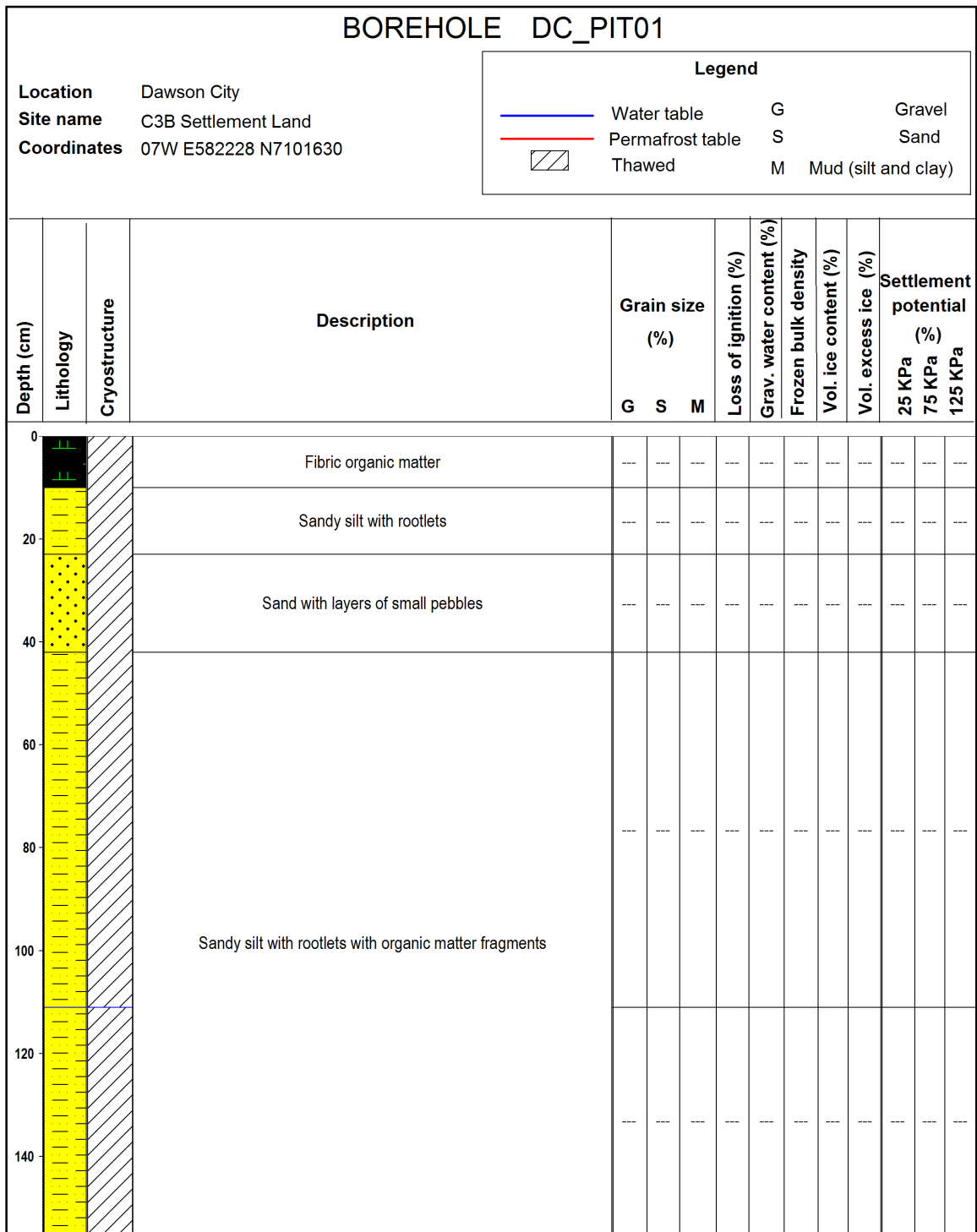
Figure B11. Log for soil pit DC_PIT01, from the C-3B case study site (see Figure 54 in the main body of this report for location).
