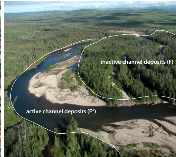
Figure 28. Late-Pleistocene to Holocene fluvial deposits on the Klondike River. Active fluvial deposits ( F^A ) include stream materials that are subject to regular flooding. Inactive fluvial deposits ( F ) include terraces above the floodplain and valley bottom deposits no longer part of the active floodplain.
