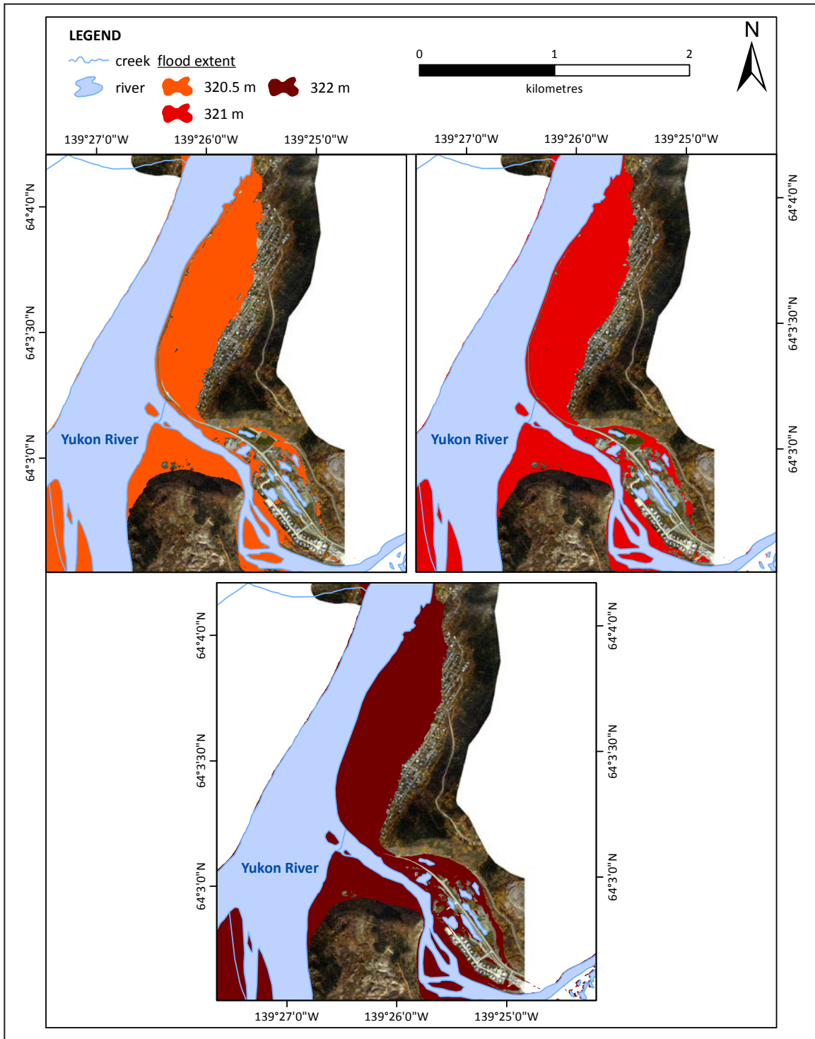
Figure 12b. Modelled flood extents for Dawson City depicting flood extent for individual Yukon River levels (relative to the Canadian Geodetic Datum) including river levels 320.5, 321 and 322 m. Note that the dike is not integrated as a barrier to flooding. Model results are based on LIDAR imagery provided by the Yukon Government. Background image source: ERSI, DigitalGlobe, GeoEye.
