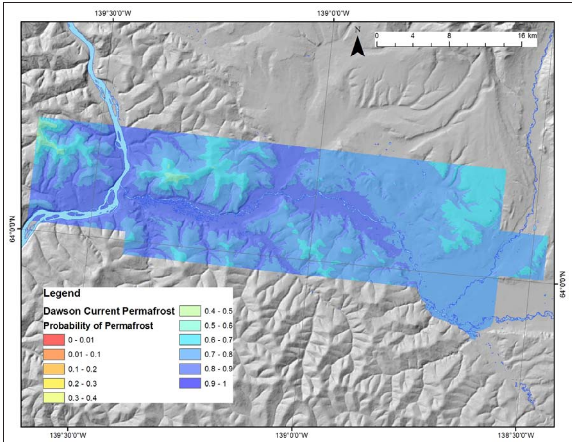
Figure 39. Permafrost probability for the Dawson region under current climate conditions.
