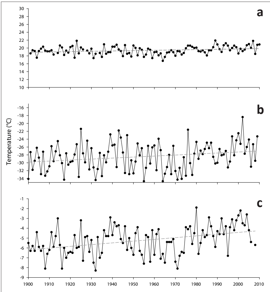
Figure 4. Historical temperature data from Dawson City, based on data amalgamated by Purves (2010), illustrating (a) summer, (b) winter and (c) annual average temperature. The dashed grey line represents a linear regression through the dataset.
