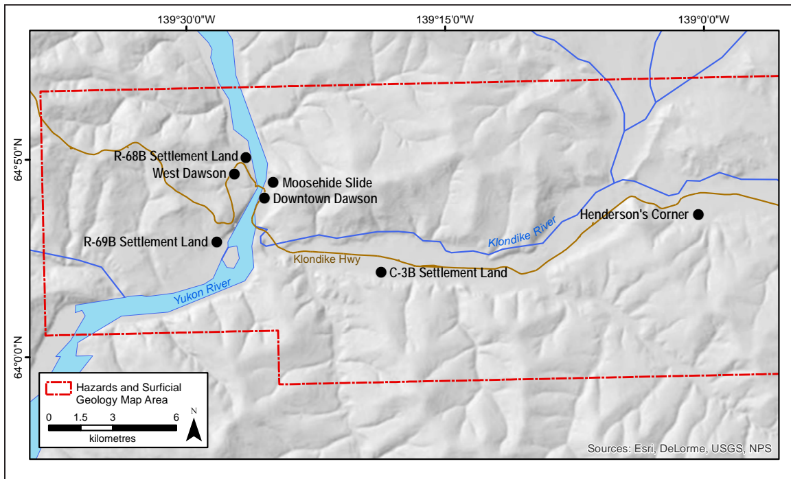
Figure 49. Overview map of all case study site locations for the Dawson area.
