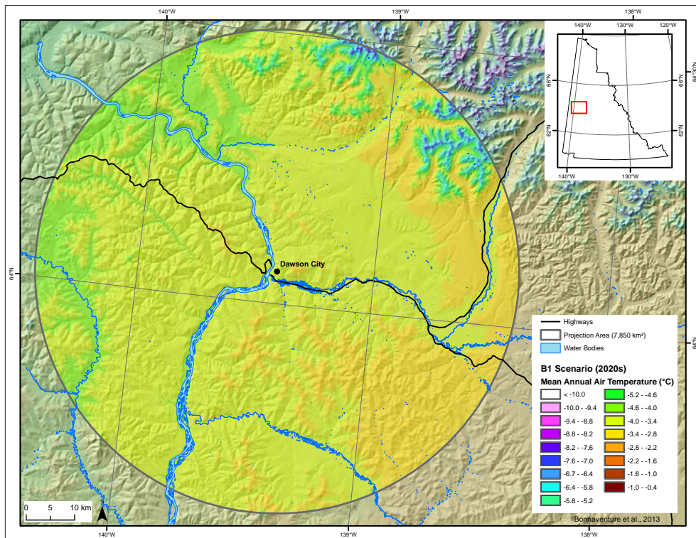
Figure D2. Mean annual air temperature for the Dawson area for 2020, projected using the B1 scenario.
