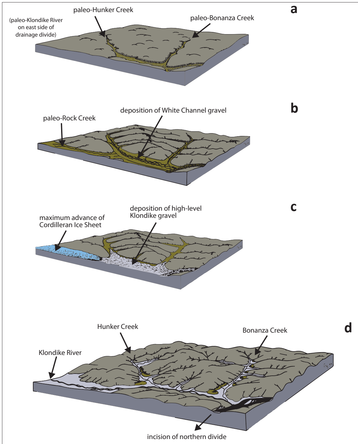
Figure 18. Evolution of the late Tertiary landscape: (a) Accumulation of the White Channel gravel begins in the early Miocene; broad, low-angle drainages of the paleo-Hunker and paleo-Bonanza creeks formed the headwaters of a south-flowing, paleo-Yukon River. (b) Continued aggradation of the White Channel gravel under a cooling climate in the late Tertiary; Rock Creek is a small tributary to the Hunker Creek drainage. (c) During the maximum advance of the Cordilleran Ice Sheet into the study area, ice overtopped the Rock Creek drainage divide, eroded the Klondike Valley, and deposited the high-level, Klondike gravel. (d) Eventual establishment of the northward flow of the Yukon River led to a lowering of base-level and incision of high and intermediate-level terraces; modern drainages are deeply incised and underfit for their broad valley profiles. Figure modified from Lowey (2004; Figure 24).
