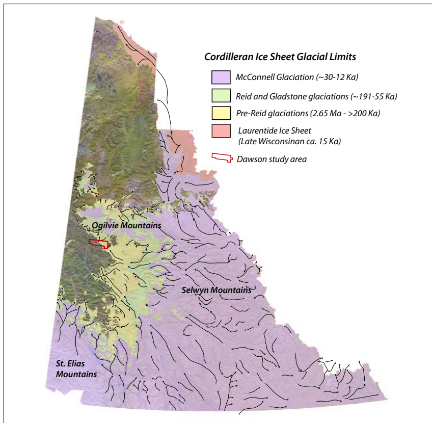
Figure 14. The study area for the Dawson Landscape Hazards Mapping Project is at the furthest extent of Pleistocene ice sheets in western Yukon. Advances of the Cordilleran Ice Sheet in Yukon became less extensive throughout the Pleistocene and the study area is thought to have only been glaciated by the earliest, Pre-Reid advances. Unglaciated areas of Yukon were part of the landmass known as Beringia, which remained unglaciated throughout the Pleistocene. Arrows indicate ice-flow directions. Figure modified from Duk-Rodkin (1996).
