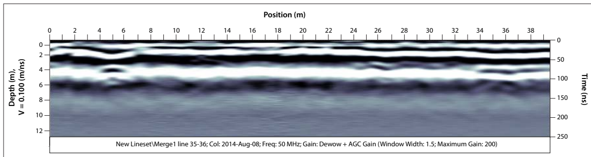
Figure 56. GPR profile DC_GPR02 from the C-3B case study site, showing a reflection at a depth of 0.3-1 m, which may correspond to the top of the permafrost table.
