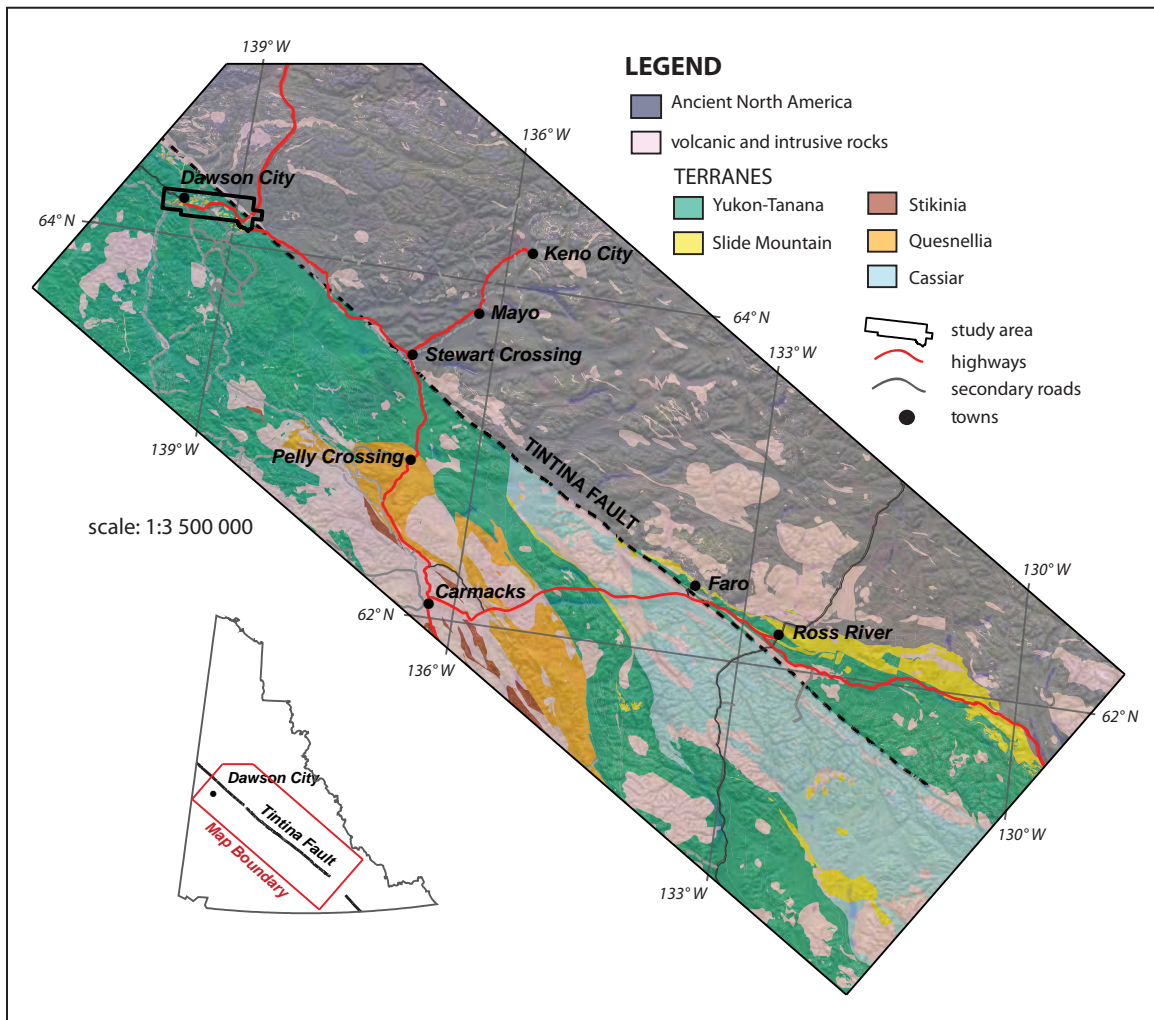
Figure 16. Simplified terrane map of the study area and surrounding regions. The majority of the bedrock in the study area comprise rocks of Yukon-Tanana and Slide Mountain terranes. From Colpron (2014).
