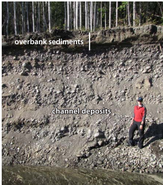
Figure 29. Holocene channel and overbank deposits on the Klondike River.
