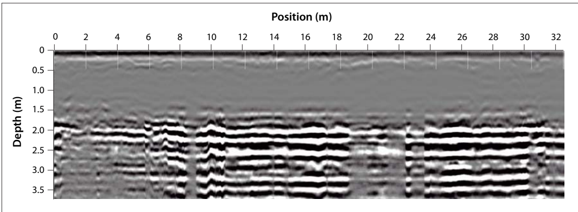
Figure 64. GPR profile DC_GPR04b for the R-69B case study site, showing a strong reflection at a depth of ~2 m.
