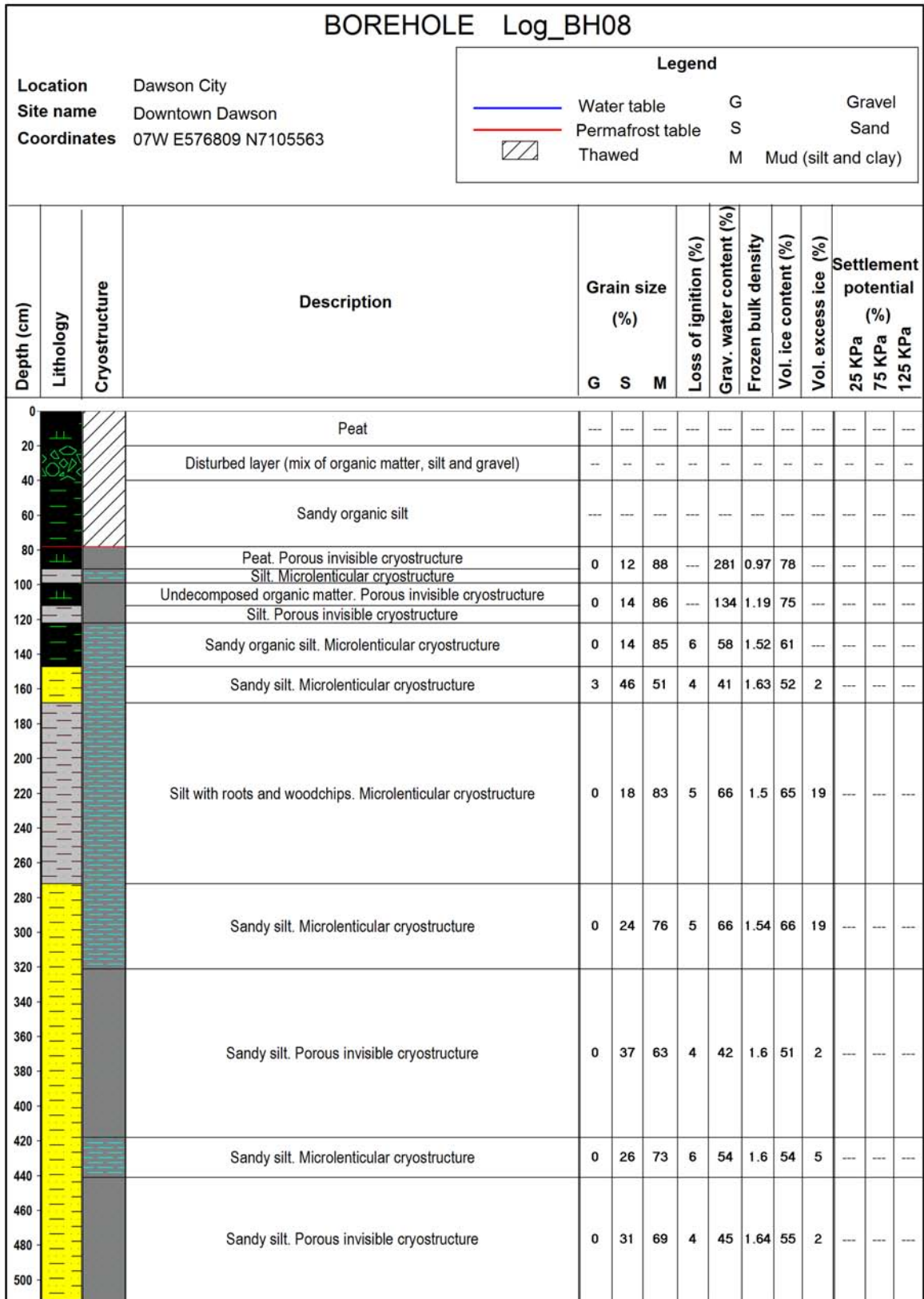
Figure B8. Borehole log for borehole DC_BH08, from the downtown Dawson case study site (see Figure 66 in the main body of this report for location).
