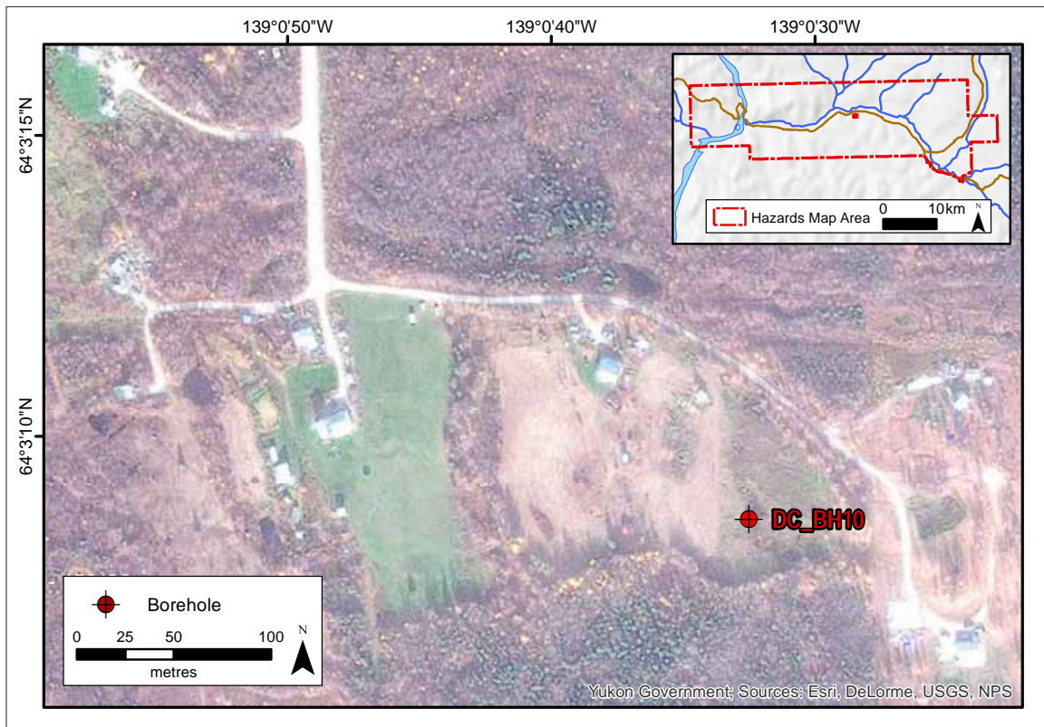
Figure 68. Map illustrating location of detailed site investigation at Henderson's Corner. Refer to Figure 49 for case study location.
