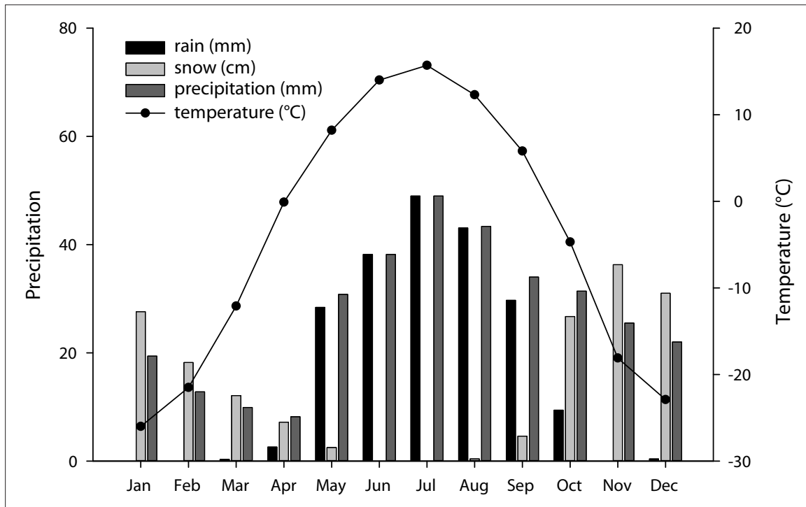
Figure 2. Climate normal (1981-2010) temperature and precipitation data for the Dawson City Airport meteorological monitoring station (Environment Canada, 2014a). To calculate total precipitation in millimetres, snowfall was converted to snow water equivalent and summed with rainfall.
