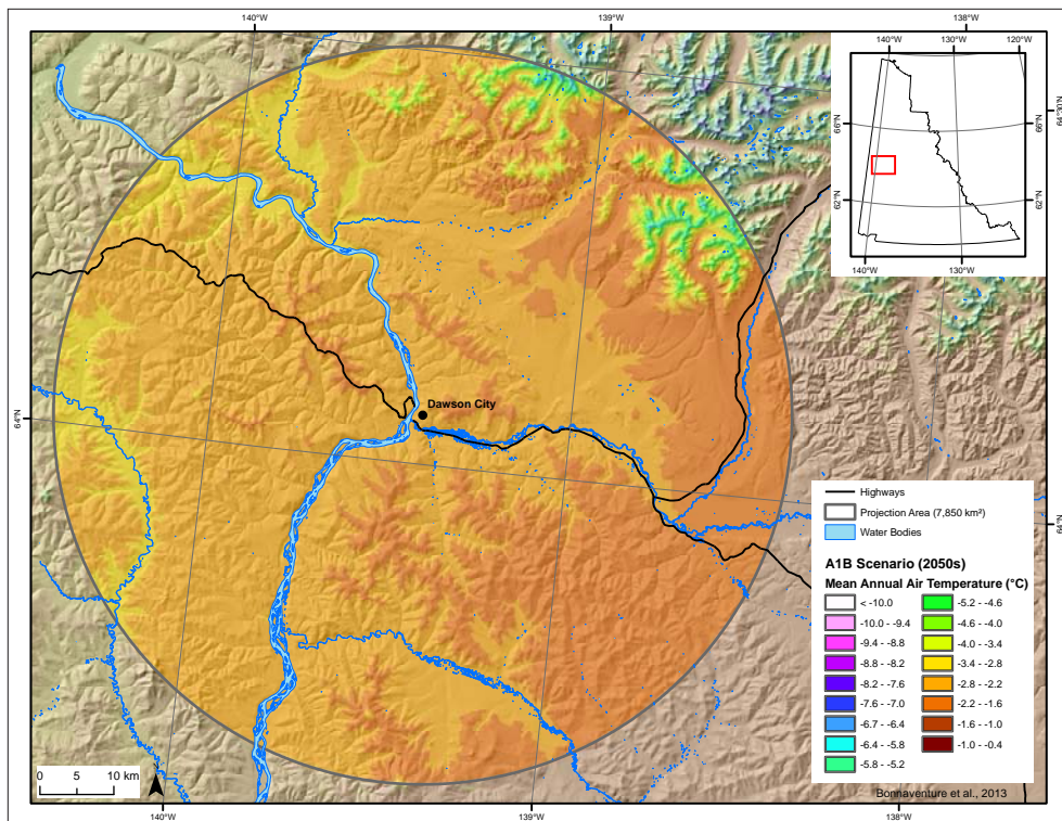
Figure D6. Mean annual air temperature for the Dawson area for 2050, projected using the A1B scenario.
