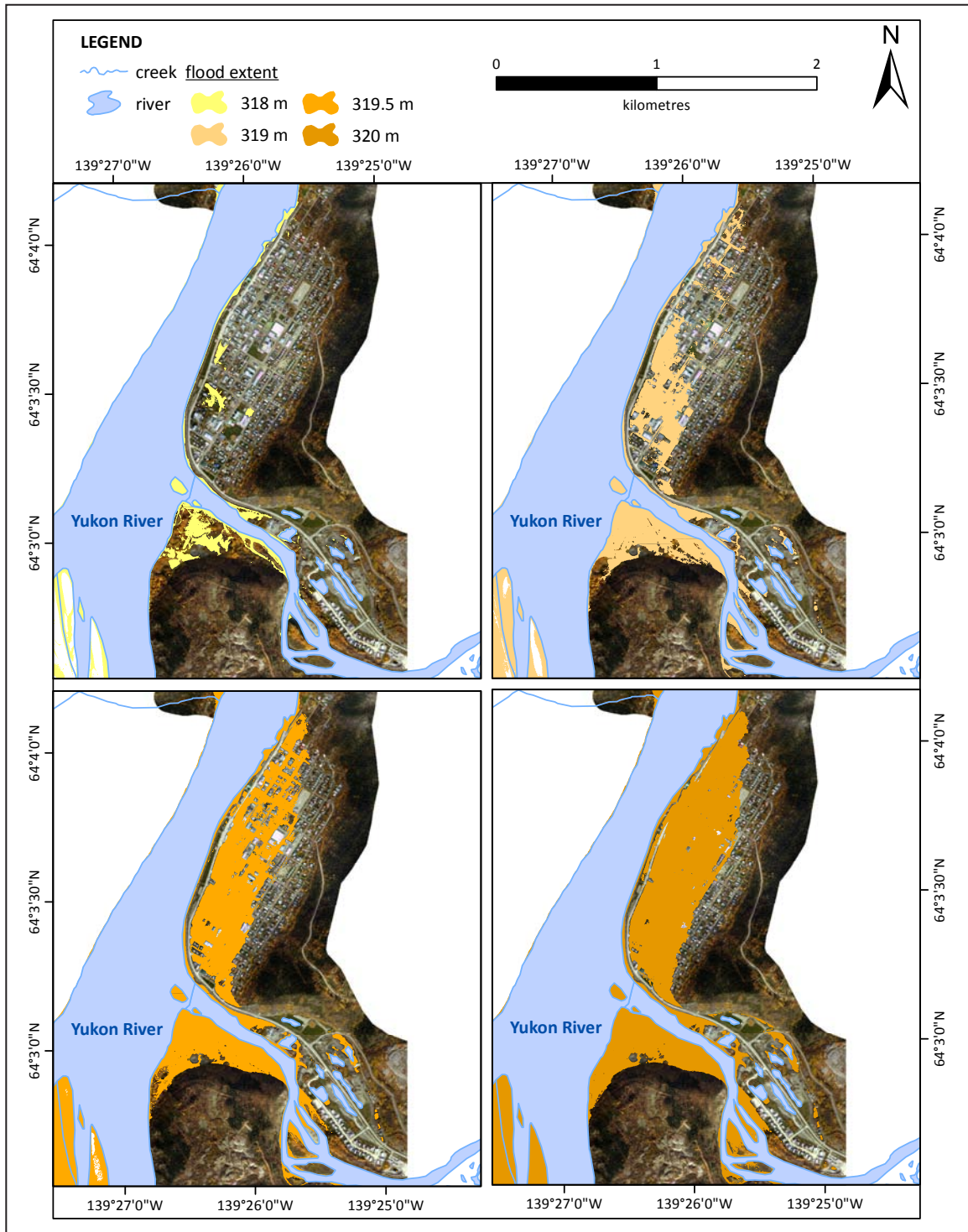
Figure 12a. Modelled flood extents for Dawson City depicting flood extent for individual Yukon River levels (relative to the Canadian Geodetic Datum) including river levels of 318, 319, 319.5 and 320 m. Note that the dike is not integrated as a barrier to flooding. Model results are based on LIDAR imagery provided by the Yukon Government. Background image source: ERSI, DigitalGlobe, GeoEye.
