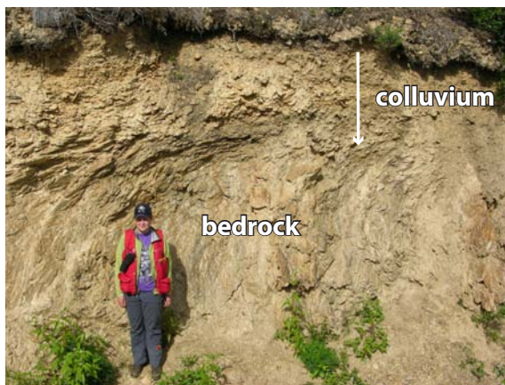
Figure 32. Hillslope colluvium generated from weathered bedrock.
