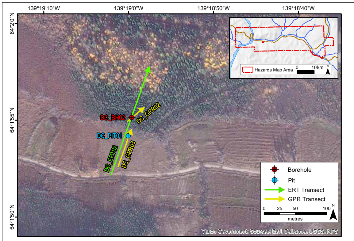
Figure 54. Map illustrating locations of detailed site investigations for the C-3B case study site. Refer to Figure 49 for case study location.
