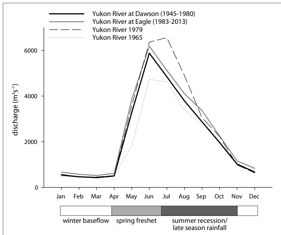
Figure 7. Average monthly discharge hydrograph for the Yukon River at Dawson (heavy solid line) and Eagle (heavy grey line). Also shown are hydrographs for the years 1965 (dotted line) and 1979 (long-dashed line), demonstrating low and high measured peak discharge, respectively (Water Survey of Canada, 2015).
