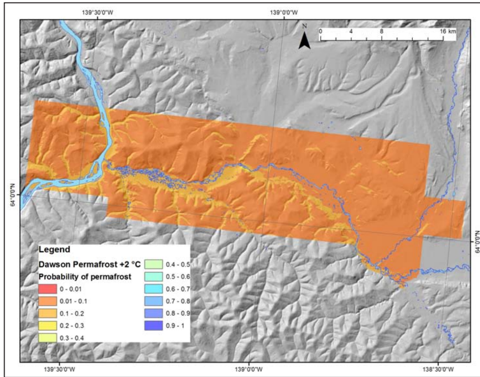
Figure 70. Projected permafrost probability for the Dawson region under an increase in mean annual air temperature of 2°C.
