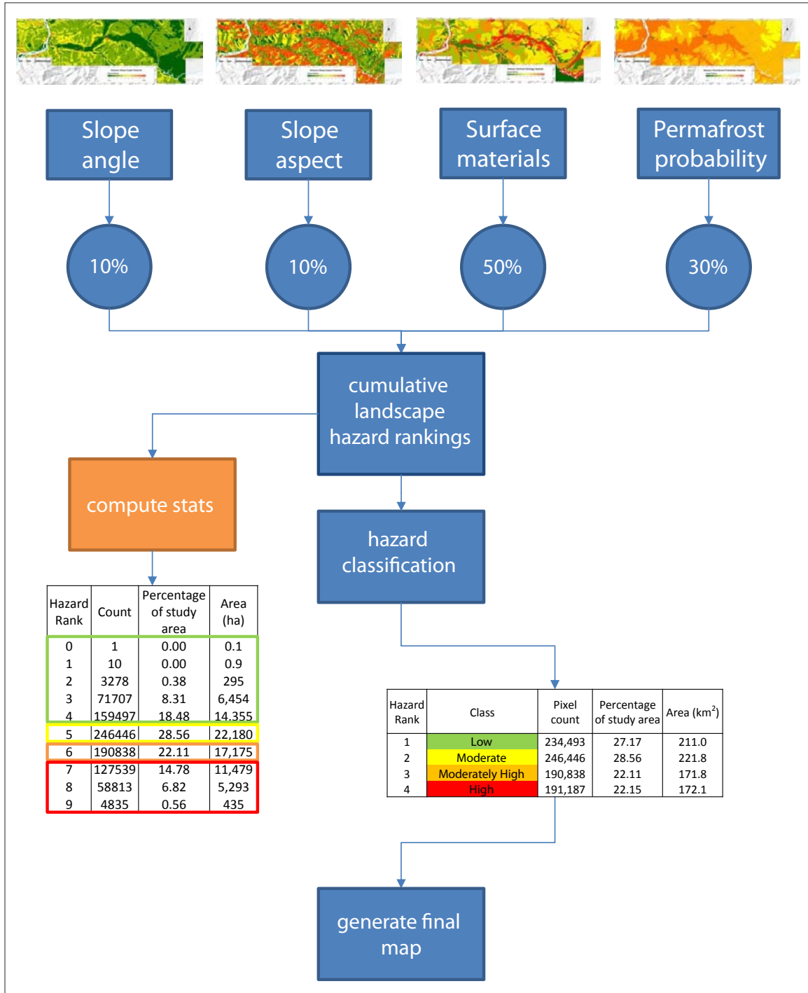
Figure 78. Flowchart illustrating the process used to create the cumulative hazard risk map out of model input parameters for the Dawson region.
