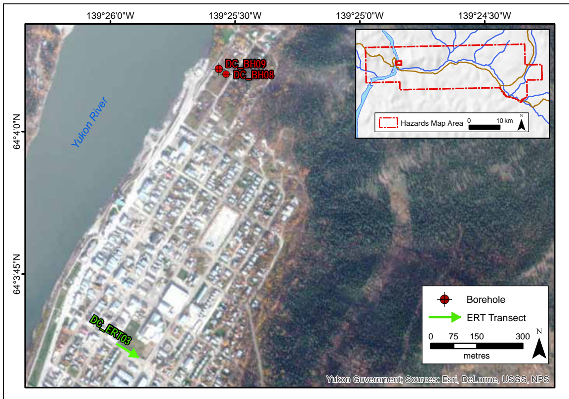
Figure 66. Map illustrating locations of detailed site investigations in downtown Dawson. Refer to Figure 49 for case study location.
