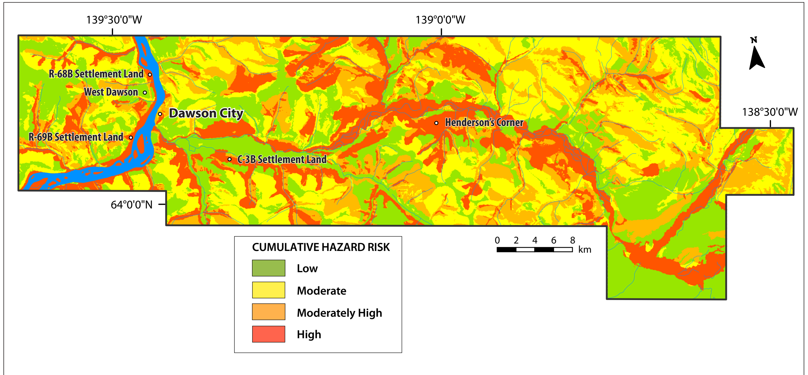
Figure 79. Map depicting hazard risk ranking for the Dawson area (see Figure 1 for location of the map boundary). A larger fold-out version of this map is included in the map pocket in the back of this report.
