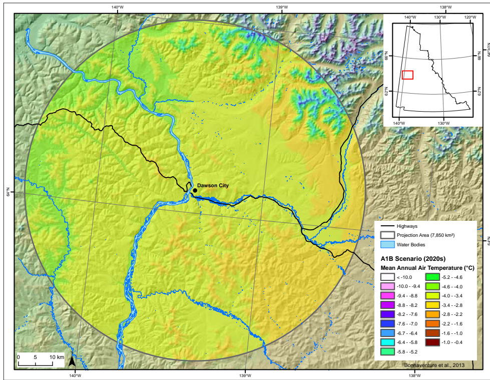
Figure D3. Mean annual air temperature for the Dawson area for 2020, projected using the A1B scenario.
