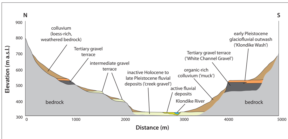
Figure 38. An idealized cross-valley profile for the lower Klondike River valley. View is looking up the Klondike River near its confluence with the Yukon River.
