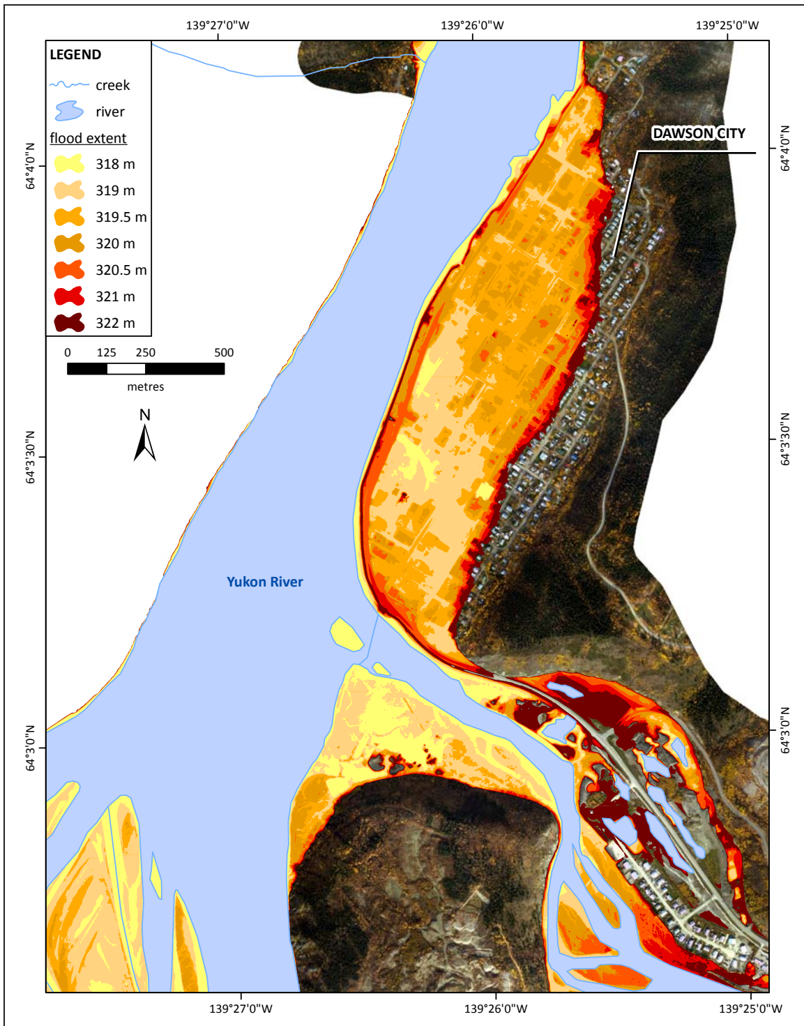
Figure 11. Close-up of amalgamated modelled flood extents for Dawson City illustrating Yukon River levels between 318 m and 322 m (relative to the Canadian Geodetic Datum). Note that the dike is not integrated as a barrier to flooding. Model results are based on LIDAR imagery provided by the Yukon Government. Background image source: ERSI, DigitalGlobe, GeoEye.
