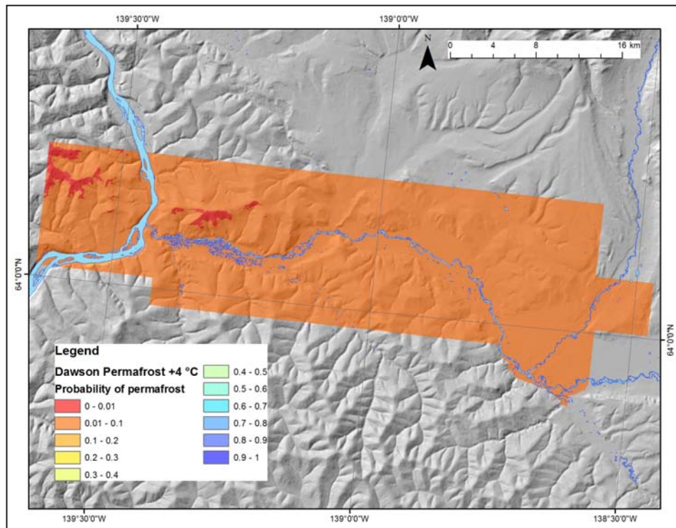
Figure 72. Projected permafrost probability for the Dawson region under an increase in mean annual air temperature of 4°C.
