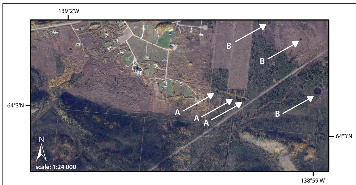
Figure 48. A satellite image of Henderson's Corner shows human-induced thermokarst where vegetation was cleared along a linear path (A), and natural thermokarst ponds in the floodplain of a fluvial fan (B).
