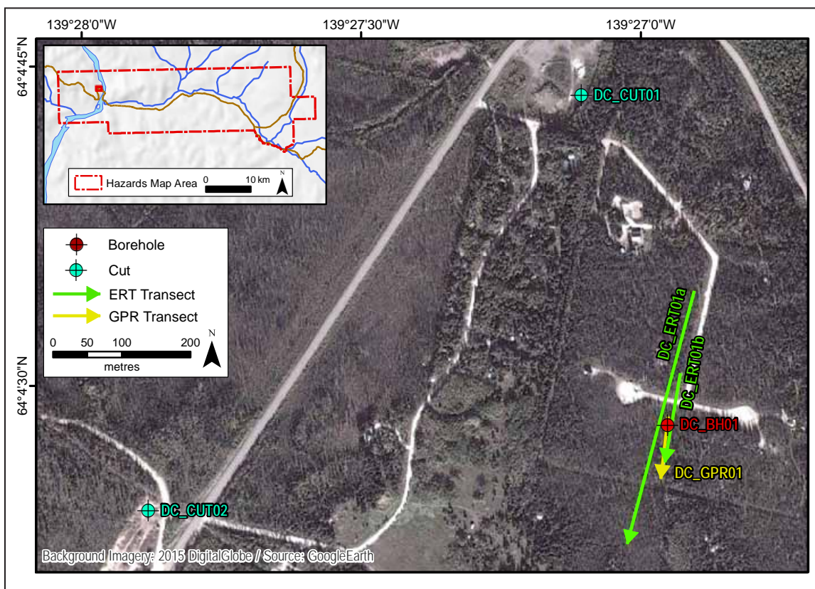
Figure 50. Map illustrating locations of detailed site investigations for the West Dawson case study site. Refer to Figure 49 for case study location.
