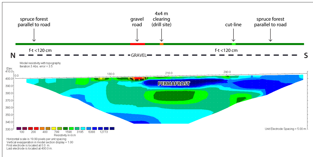
Figure 52. ERT profile DC_ERT01a, is 400 m long and runs parallel to DC_ERT01b (see Figure 50 for location). The profile has a maximum penetration depth of ~60 m. Likely areas of permafrost are outlined by black dashed lines; f-t = frost table.
