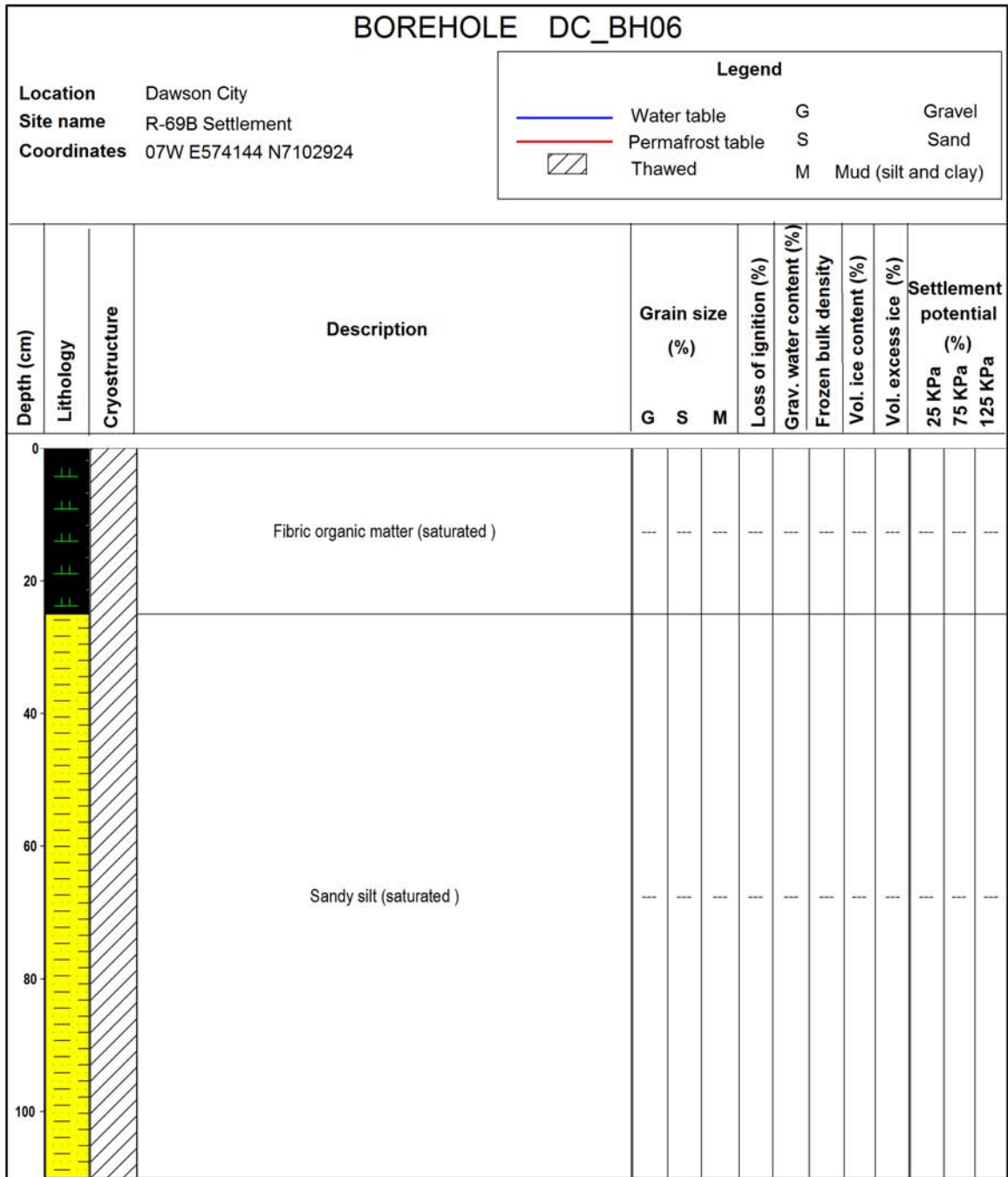
Figure B6. Borehole log for borehole DC_BH06, from the R-69B case study site (see Figure 60 in the main body of this report for location).
