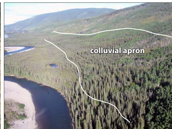
Figure 33. Colluvial aprons (outlined) are commonly comprised of resedimented colluvium and loess near the Klondike River.
