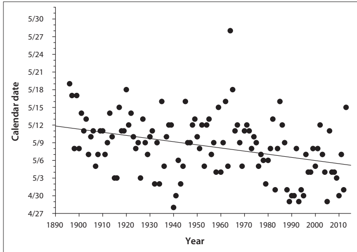
Figure 8. Spring breakup dates for the Yukon River between 1896 and 2013 (from http://www.yukonriverbreakup.com/statistics ). The solid line represents a best-fit regression through the complete dataset.
