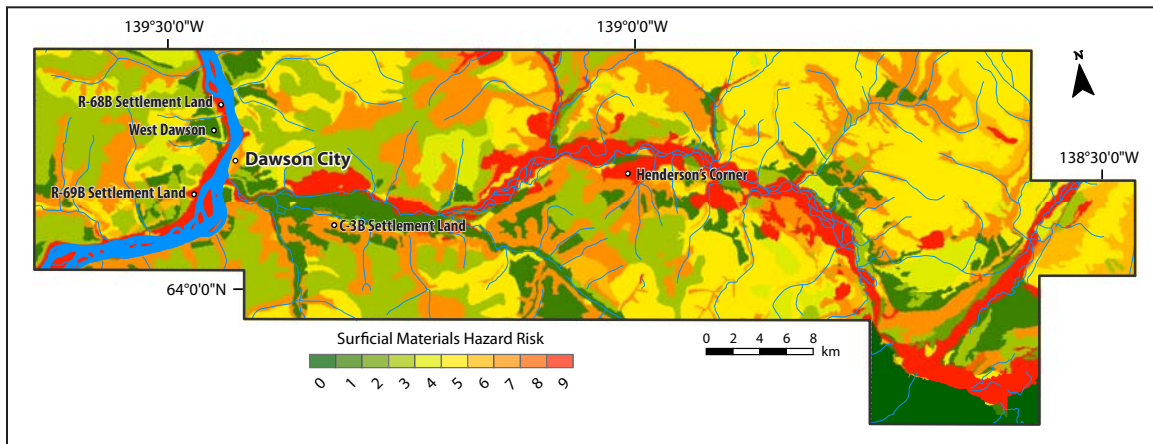
Figure 77. Hazard risk associated with surficial materials in the Dawson region. Stable geological units (e.g., fluvial and glaciofluvial landforms above floodplains, weathered bedrock, coarse-grained colluvium overlying bedrock) are classified as lowest risk (dark green) while geological units affected by landslides, thermokarst, ice-wedge polygons or flooding are classified as highest risk (dark red).
