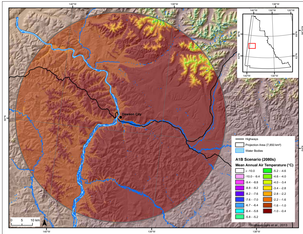
Figure D9. Mean annual air temperature for the Dawson area for 2080, projected using the A1B scenario.
