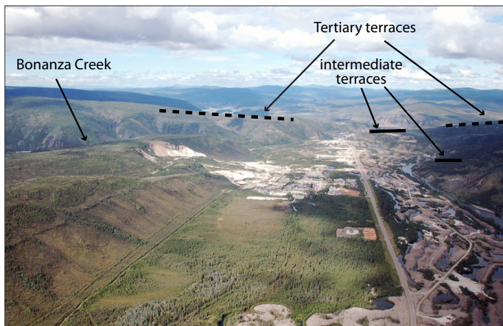
Figure 20. Photo of the lower Klondike River valley (view west toward the Yukon River) with broad Tertiary fluvial surface high on the hillside, intermediate terraces on the north side of the valley, and the narrow Quaternary valley occupied by the modern drainage.
