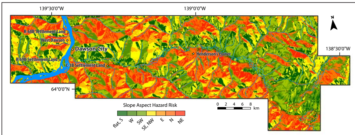
Figure 75. Hazard risk associated with slope aspect in the Dawson region.
