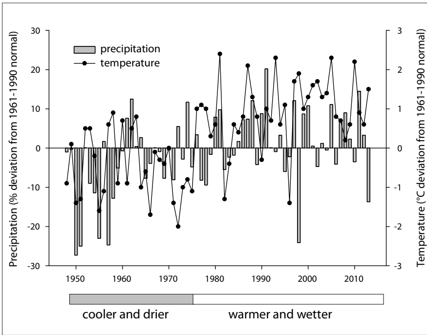
Figure 3. Regional climate trends for northern British Columbia and Yukon, developed using data amalgamated by Environment Canada (2014b). Data has been normalized to indicate deviation from 1961-1990 climate normal conditions. Negative values indicate precipitation amounts and temperatures below normal for the 1961-1990 period, while positive values indicate exceedance of normal conditions.
