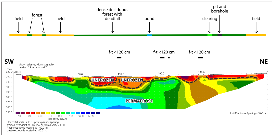
Figure 61. ERT profile DC_ERT05, which is 500 m long and runs southwest to northeast through forest towards the Yukon River (see Figure 60 for location). The profile has a maximum penetration depth of ~60 m. Likely areas of permafrost are outlined by black dashed lines; f-t = frost table.
