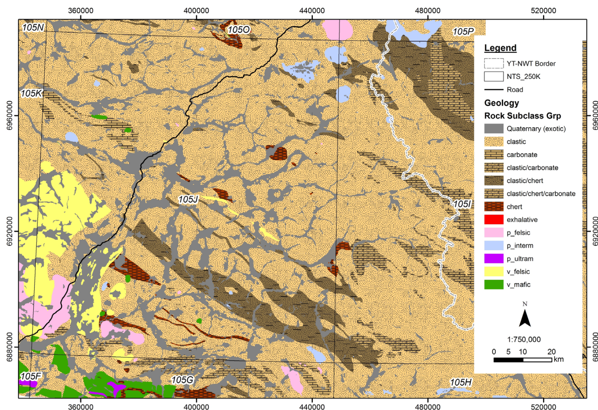
Figure 2. Example of simplified geological units for map sheets 105J and 105I.
