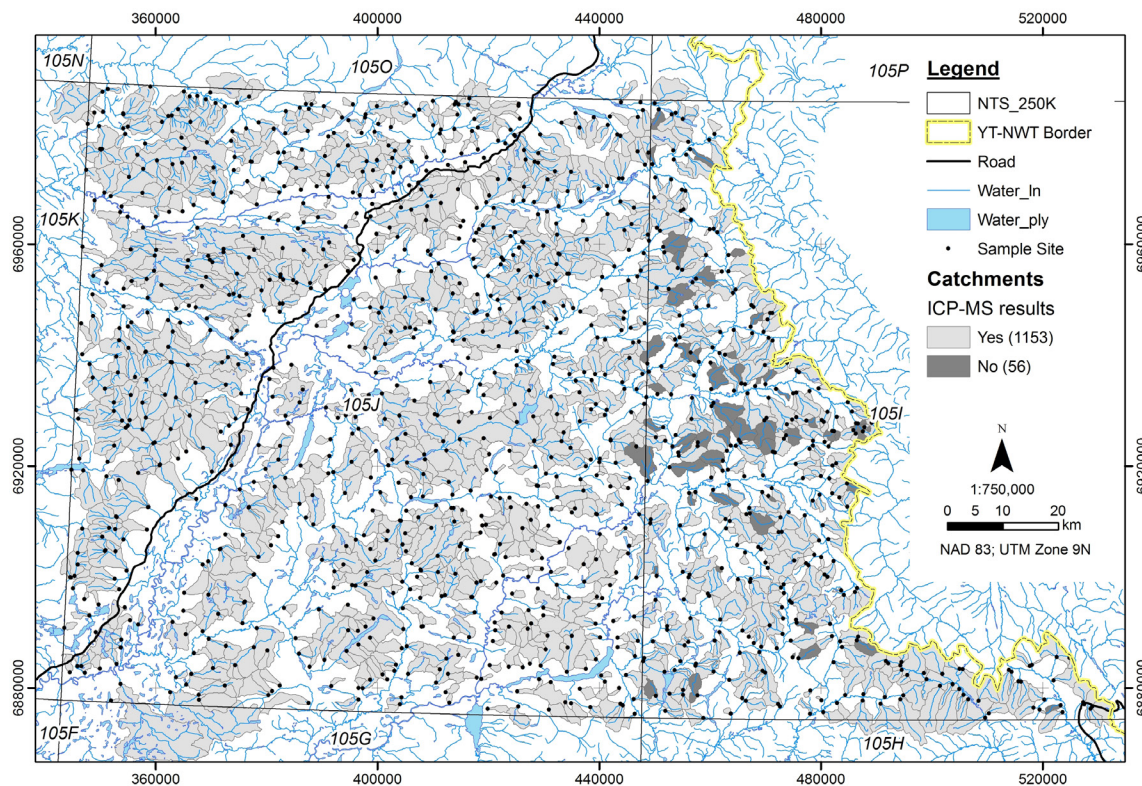
Figure 1. Example of stream sediment sample locations and catchments for map sheets 105J and 105I.
