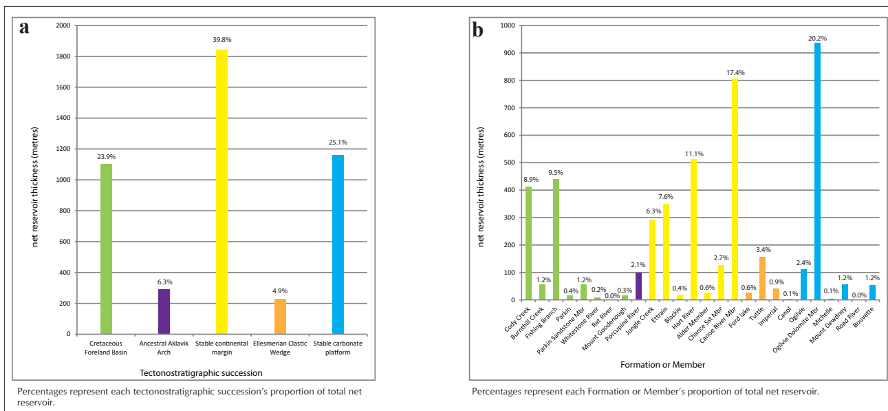
Figure 9. Graph of net reservoir thickness using cutoff parameters #3 (least conservative) per tectonostratigraphic succession (9a) and per Formation/Member (9b).
