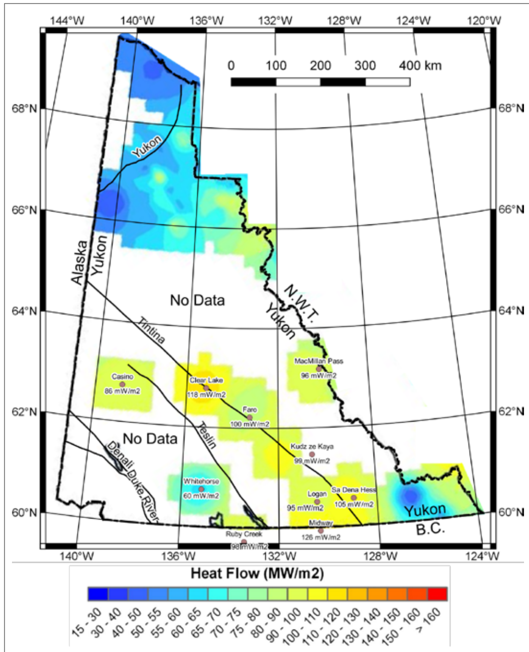
Figure 2. Heat flow map of Yukon from Grasby et al. (2012). Warm colours represent high heat flow and cool colours, low heat flow. Selected heat flow data points from Lewis et al. (2003) are also shown as brown dots labelled with the location and heat flow value. Portions of central and southern Yukon show elevated heat flow compared to other parts of Yukon. Much of the territory lacks heat flow measurements. Black lines depict major faults (Colpron and Nelson, 2011). Map is in Yukon Albers NAD83.
