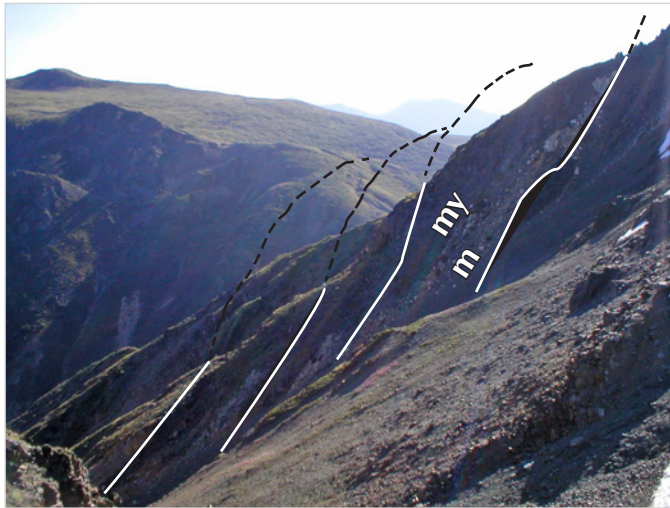
Figure 11. East-vergent duplex structures repeating marble (m) and mylonite (my) on the north face of Tally Ho Mountain.
