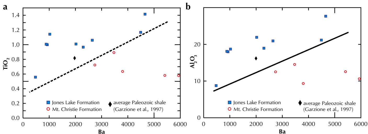
Figure 9. (a) \text{TiO}_2 versus Ba; and (b) \text{Al}_2\text{O}_3 versus Ba. Lines separate Mount Christie Formation samples from Jones Lake Formation samples. Paleozoic shale data from Garzione et al. (1997).
