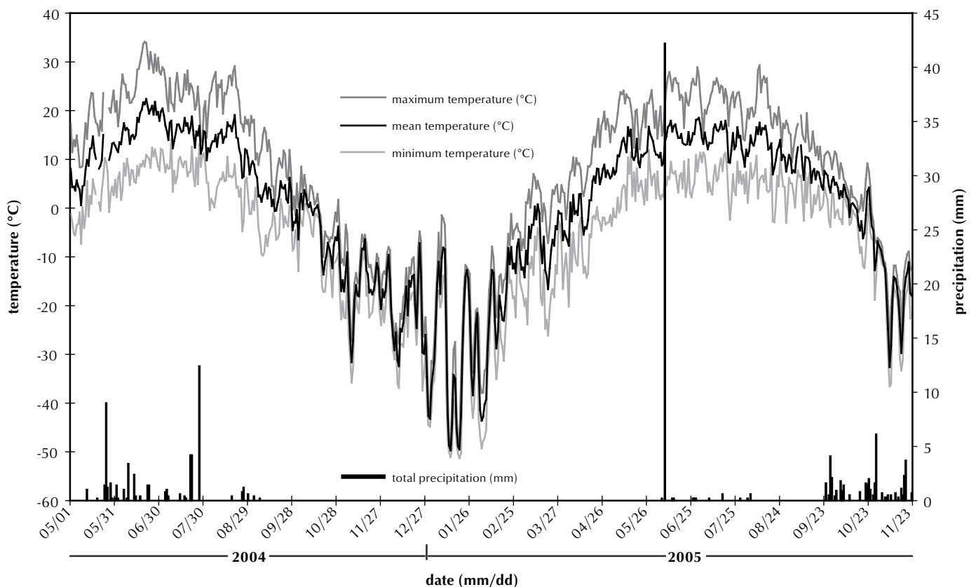
Figure 2. Daily temperatures (mean, maximum and minimum) and total daily precipitation at Dawson weather station ( 64^{\circ}3'\text{N} , 139^{\circ}7'\text{W} , elevation 370 m; data from Environment Canada).
