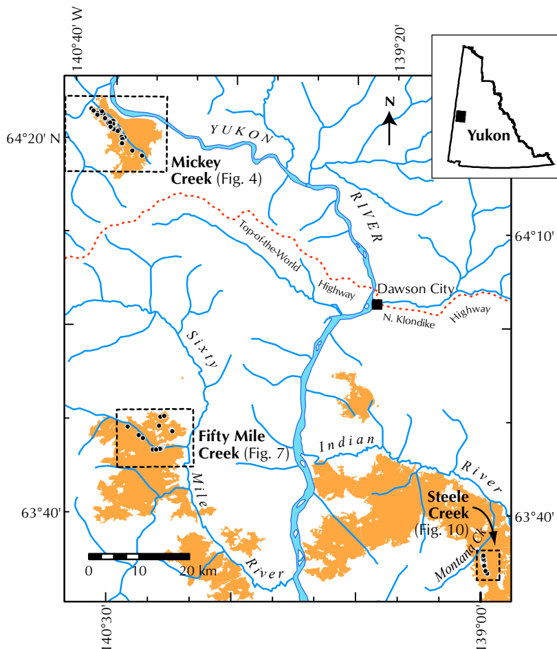
Figure 1. Index map of Dawson area, displaying the locations of Mickey Creek, Fifty Mile Creek and Steele Creek watersheds. Dots represent locations of active-layer detachments. Shaded areas represent those regions burned by forest fires in 2004. Inset map shows location of study area within Yukon.
