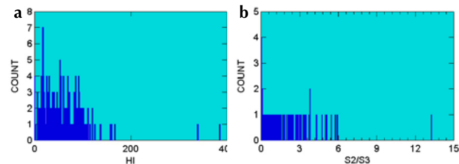
Figure 11. Rock-Eval quality parameters, Tantalus Formation.
