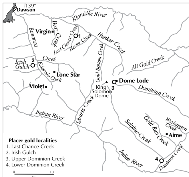
Figure 2. Location map of the Klondike District showing the main placer streams and locations of specific placer gold samples (○) and lode gold (■) occurrences.
