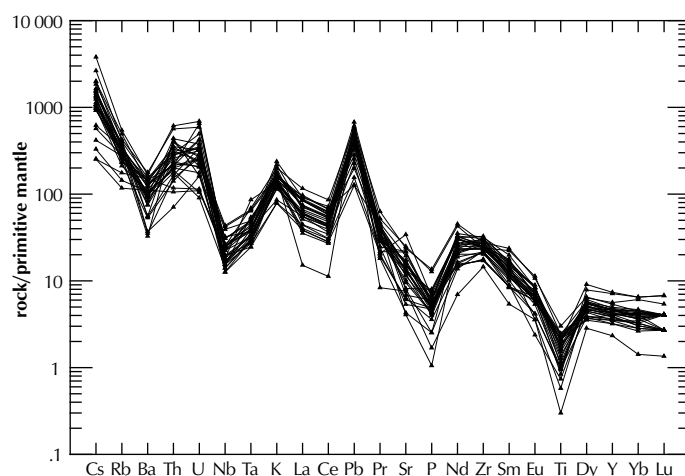
Figure 5. Primitive-mantle-normalized extended trace element diagram of the 2005 plutonic samples; n = 31 . Mantle-normalized values from Sun and McDonough, 1989.
