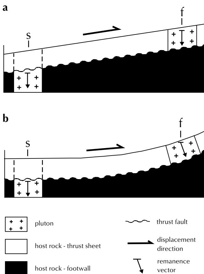
Figure 10. Schematic depiction, not to scale, of the head of a beheaded pluton being pushed up a thrust fault ramp that is: (a) linear; and, (b) curved. Note in a that the ChRM vector in the head and its host rocks in the thrust sheet are unchanged in inclination from the start (s) of displacement to its final (f) position, whereas in b that the vector's inclination shallows as the curved ramp's inclination steepens and the sheet moves towards the paleopole. Deadman pluton likely endured various amounts of both types of displacement before reaching its current location.
