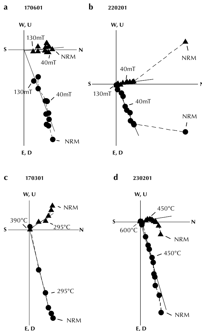
Figure 6. Alternating-field and thermal step demagnetization of example specimens from the host rock skarn of the Deadman pluton from: (a) site 17; (b) site 22; (c) site 17; and (d) site 23. Conventions as in Figure 3 and 4. The J_0 values in 10^{-1} A/m are: (a) 0.591; (b) 0.253; (c) 4.01; and (d) 5.50.
