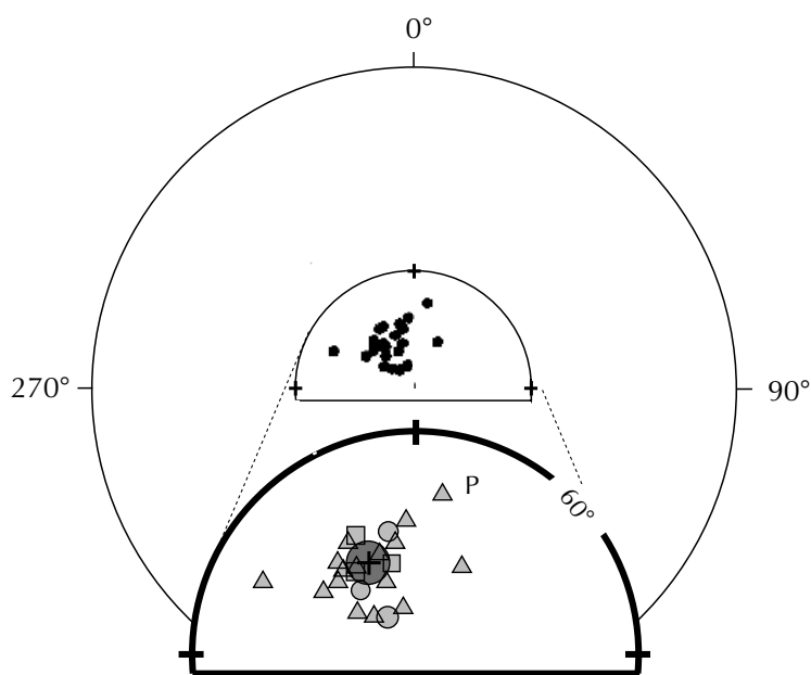
Figure 8. Equal-area stereonet showing the site mean directions for the Deadman pluton collection. Site symbols: ▲ pluton, ■ dykes, ● host rock skarn. The inset shows the central portion of the stereonet at inclinations of >60^\circ for added clarity, along with the population mean (+) and its cone of 95% ( 2\sigma ) confidence. The present Earth's magnetic field direction is shown by a "P".
