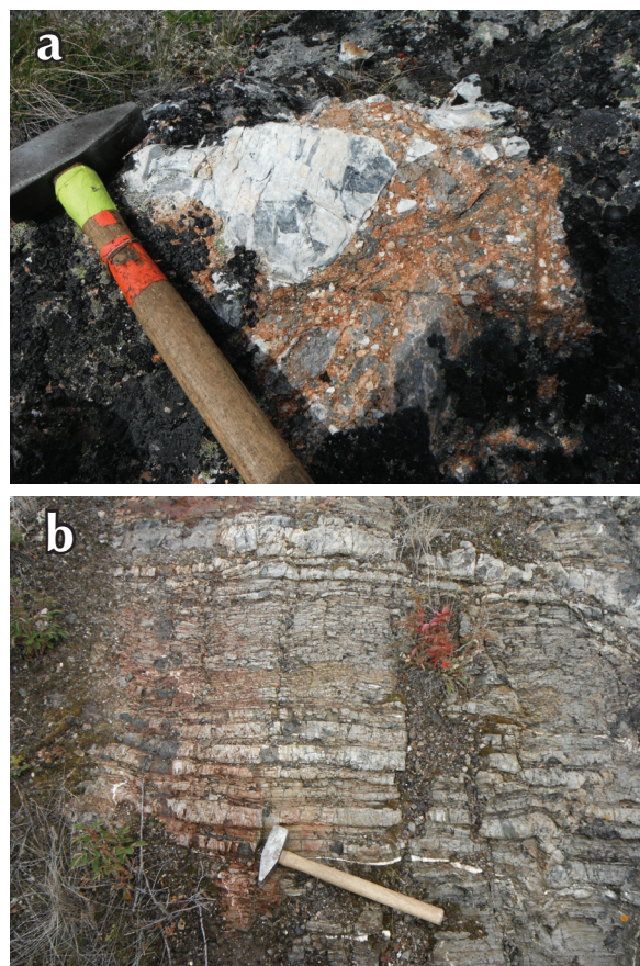
Figure 4. Outcrop photos of Cache Creek terrane rocks; a) chert clasts within a volcanoclastic matrix, east of Mount Michie; and b) ribbon-banded chert in the Marsh Lake area.
