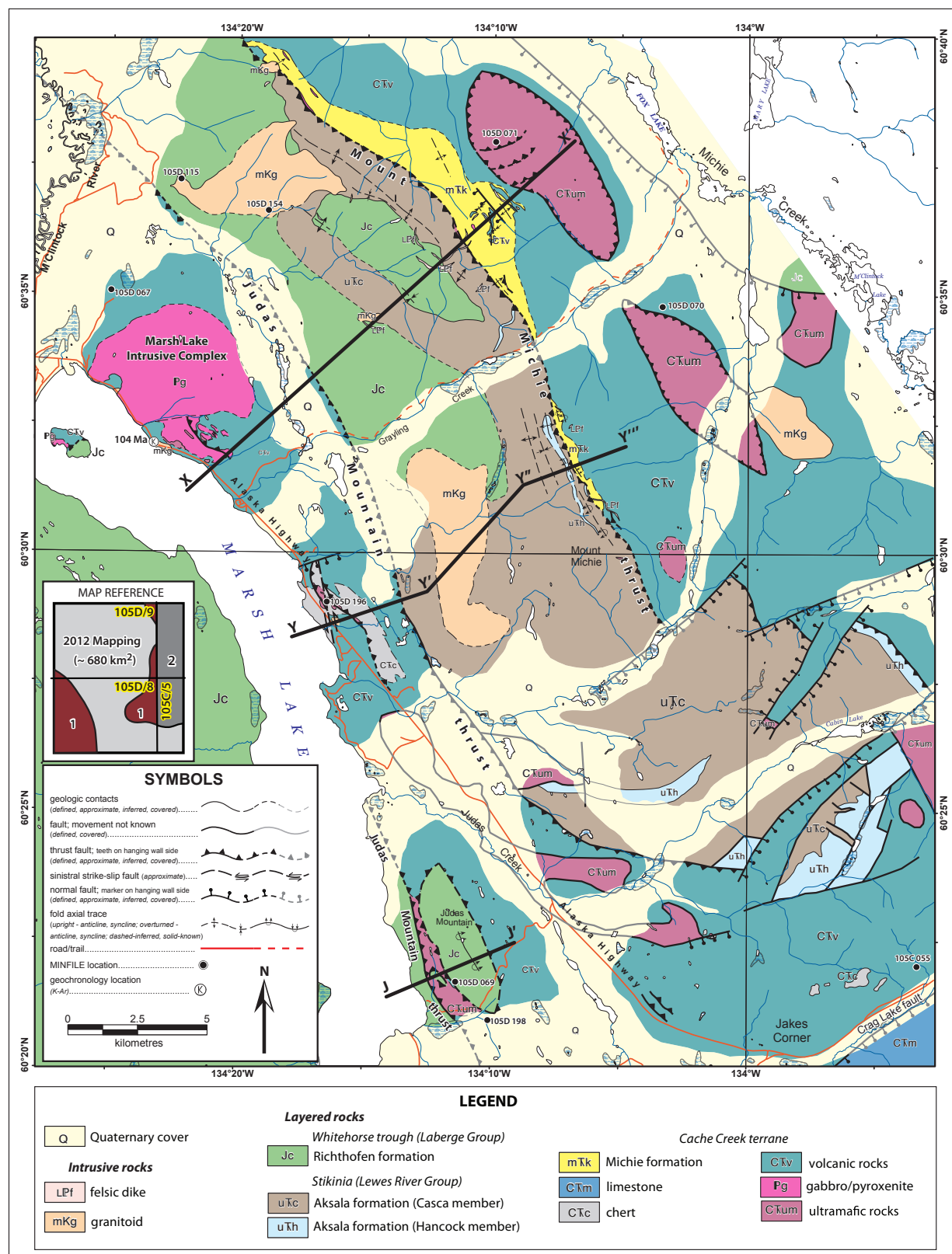
Figure 3. Simplified bedrock geology map of the study area. Map reference inset shows parts of the map area compiled from 1) Wheeler (1961); and 2) Gordey and Stevens (1994); the author's detailed mapping of an area ~680 km 2 , straddling the Michie Creek (105D/9), Tagish (105D/8), and Squanga Lake (105C/5) map areas is also indicated.
