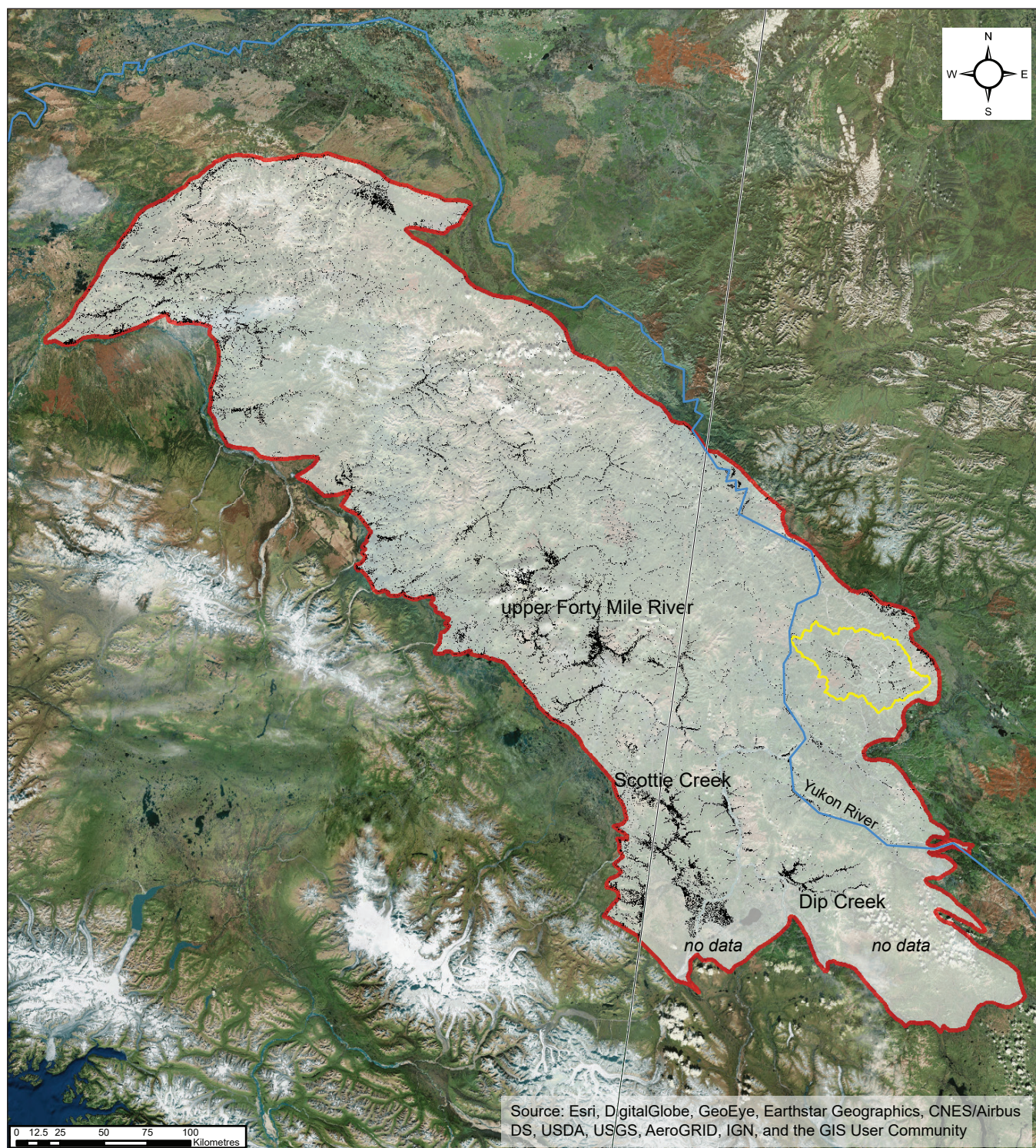
Figure 12. Distribution of wetlands across the Klondike Plateau ecoregion (white shade) that spans the border between Yukon and Alaska. Black-coloured pixels correspond to wetlands modeled by Grods, et al., 2012 and Homer, et al., 2015. The majority of the wetlands are concentrated in drainage reaches that are distal to the Yukon River such as the upper Fortymile River and Scottie Creek wetlands.
