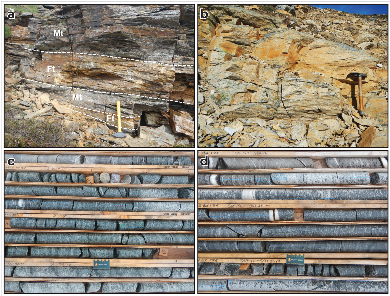
Figure 3. Field photographs of 2017 sampling locations in the Finlayson Lake region. Sample location coordinates reported as UTM Zone 9N and NAD 83. (a) 17MM-001: Wind Lake formation, felsic tuff (Ft) interbedded with mafic tuff (Mt) ~300 m above the contact with Kudz Ze Kayah formation (413749 E, 6815933 N); (b) 17MM-055: Kudz Ze Kayah formation, massive aphyric rhyolite (413086 E, 6813844 N); (c) 17MM-060: Wind Lake formation (?), biotite-chlorite altered mafic dike that crosscuts KZK stratigraphy (415122 E, 6814798 N); (d) 17MM-062: Grass Lakes plutonic suite, quartz-feldspar porphyry immediately below the deepest known KZK volcanic rocks (~580 m depth; 415122 E, 6814798 N); (e) and (f) on next page.
