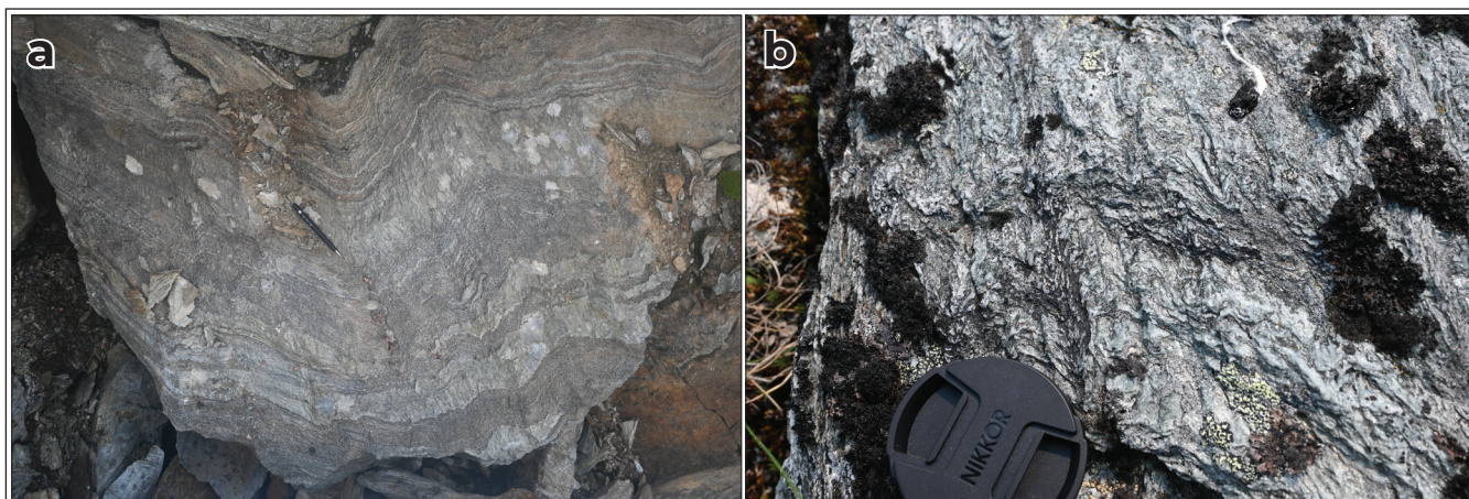
Figure 5. Evelyn Creek succession, middle division. (a) Chlorite and muscovite-rich schist interlayered with layers of quartzite and quartz-rich schist. Pencil for scale. (b) Crenulated chlorite-muscovite schist, composed of streaky quartz-rich layers separated by chlorite and muscovite-rich folia. 46 mm lens cap for scale.
