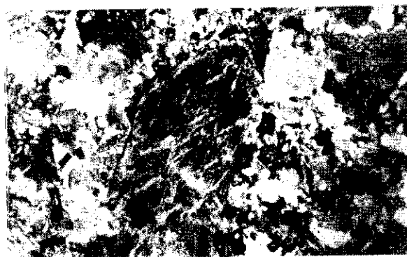
l. Photomicrograph showing propylitic alteration - epidote, chlorite and sericite; Folle plug.
