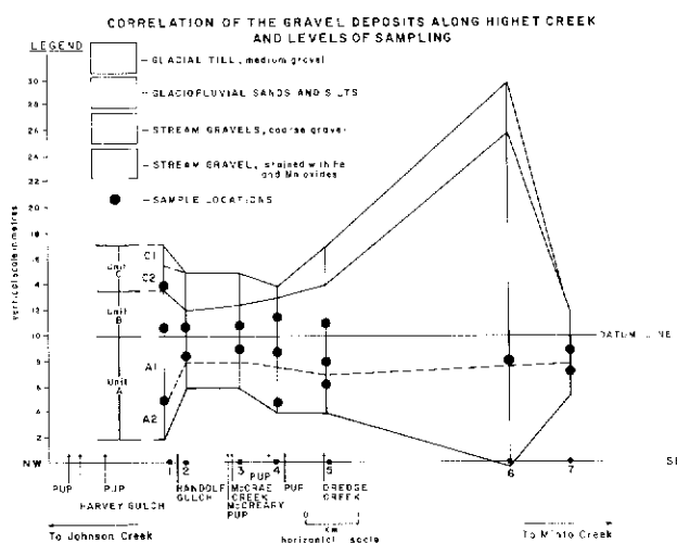
Figure 4 Correlation diagram.
