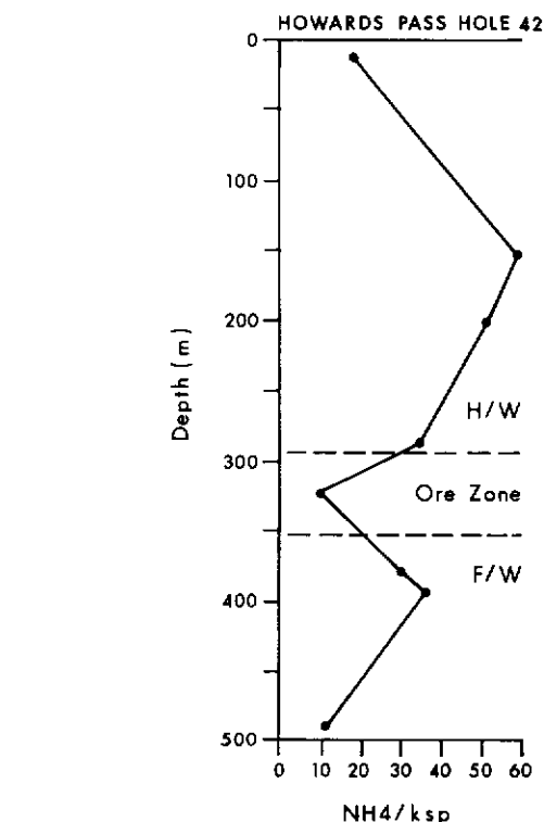
Fig. 11 Depth profile of NH 4 /feldspar, Howards Pass. NH 4 in K feldspar increases in the hanging wall.
