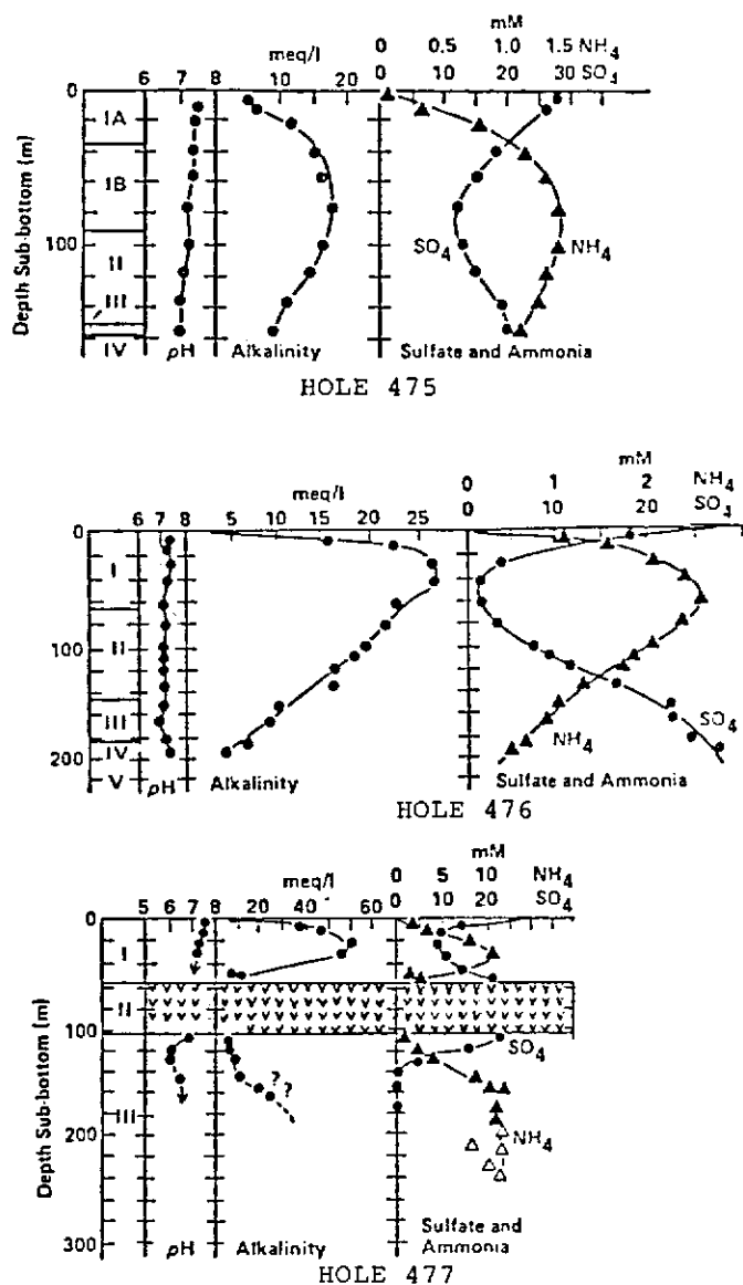
Fig. 6 NH 4 geochemistry, Guayamas Basin (from Gieskes, 1982).
