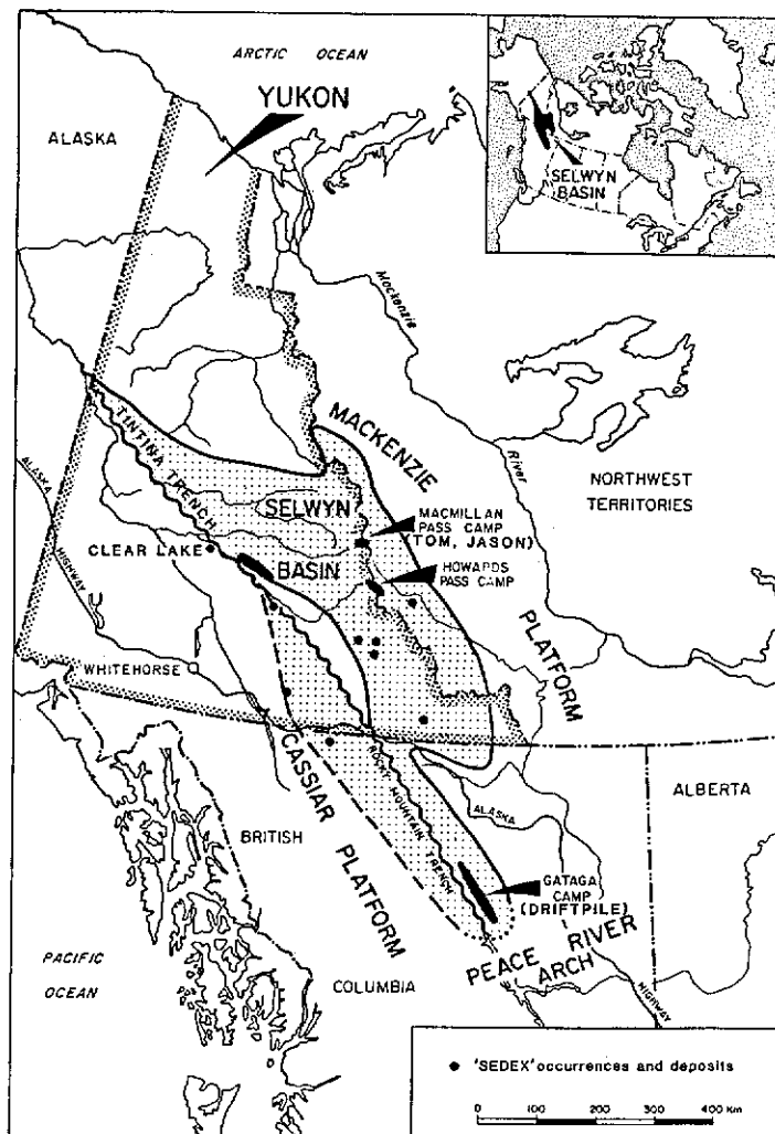
Fig. 1 Location of the Selwyn Basin and the main sedex zinc-lead-silver camps (modified from Carne and Cathro, 1981).
