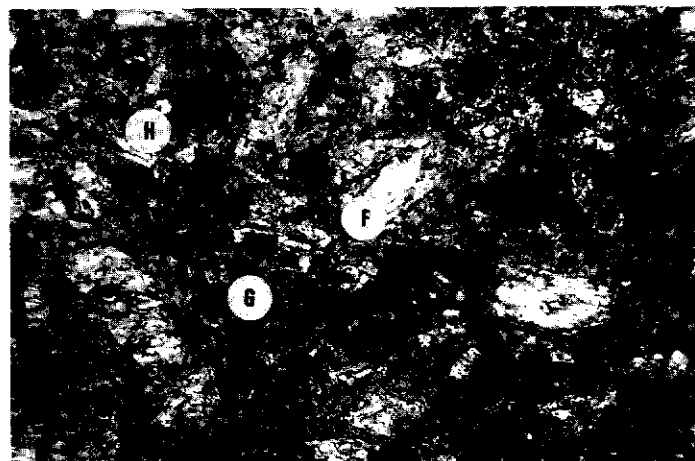
Figure 4. Photomicrograph of andesite, crossed polarizers; length of view 10 mm. F = feldspar (plagioclase), H = hornblende and G = groundmass.
