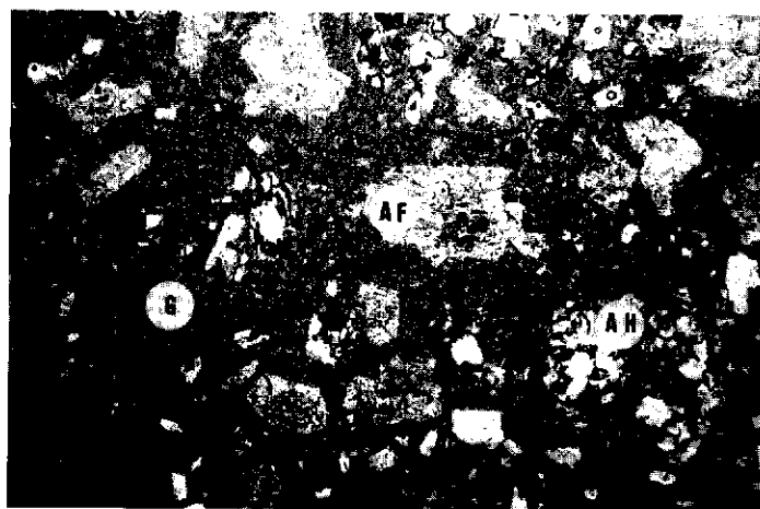
Figure 8. Photomicrograph of altered andesite, crossed polarizers; length of view 5 mm. AF = altered feldspar, replaced by clays, AH = altered and leached hornblende, and G = groundmass. Sample is from andesite opposite the Britannia adit.
