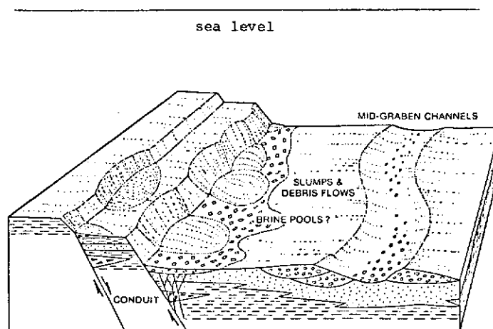
Fig. 4 Schematic diagram of the depositional environment of sulphides at MacMillan Pass, Tom and Jason deposits. Detrital influx may have diluted or washed out \text{NH}_4 in the brine pools (after Winn et al, 1981).
