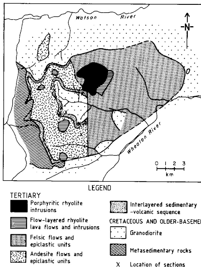
Fig. 1 Geology and major subdivisions of the Skukum volcanic complex.
