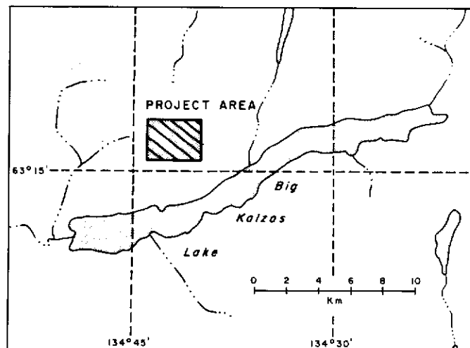
Figure 1. Index map showing location of Kalzas area.
