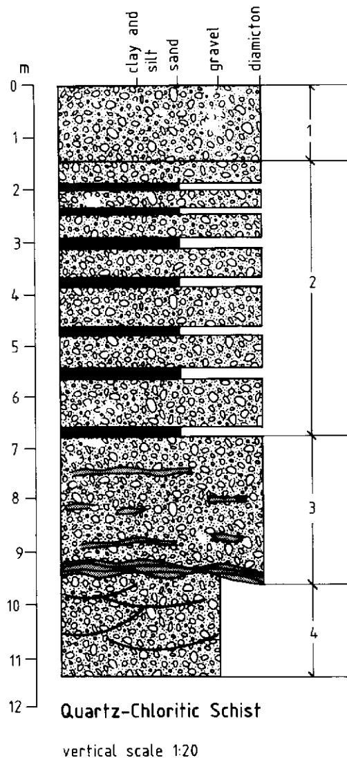
Figure 3. Stratigraphy and sedimentology of a buried placer deposit at the mouth of Left Clear Creek.
