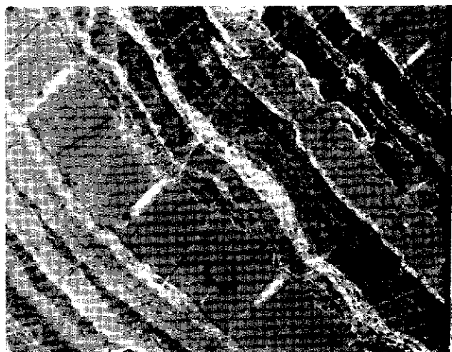
Figure 7c Laminated barite-sulphides-silica facies, lower deposit. Silicified siltstone turbidite (light grey) is interbedded with packets of laminae of barite +/- galena (medium grey) and sphalerite-quartz (white). Quartz filled tensional fractures in silicified siltstone are interpreted to relate to Mesozoic deformation. Centimeter scale. Arrow indicates stratigraphic tops.
