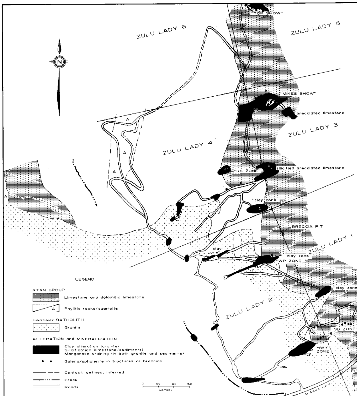
Figure 1. Geology of the STERLING property
