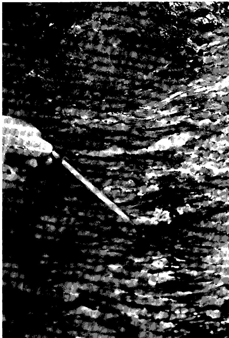
Figure 1. Tourmalinite near the LUGDUSH skarn tungsten occurrence. Note alternating black tourmaline-rich and white quartz layers.
