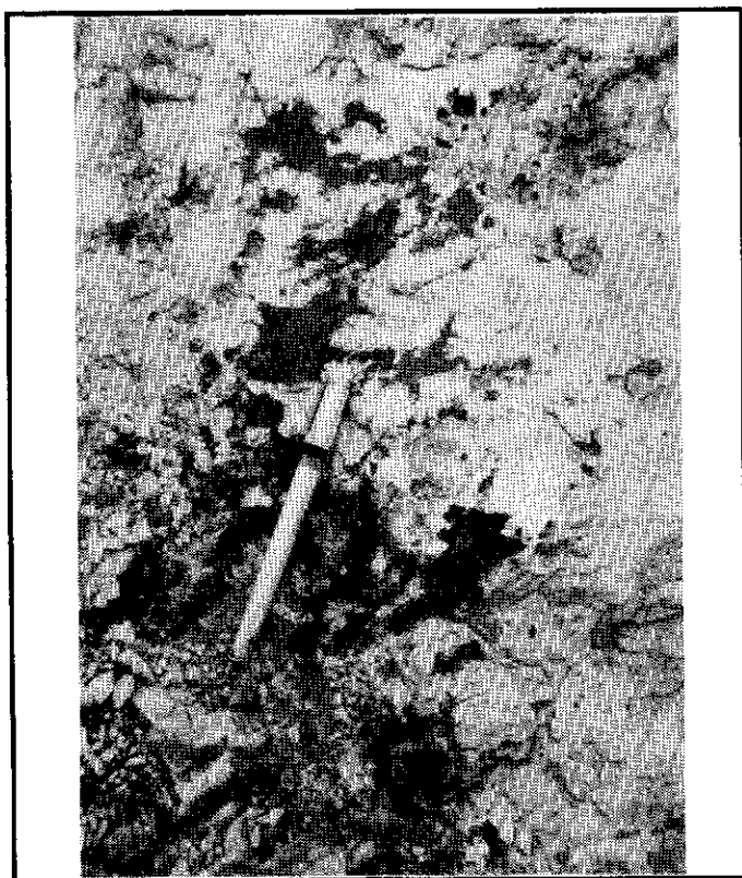
Figure 1. Irregular patches of coarse grained galena and red sphalerite in massive barite.
