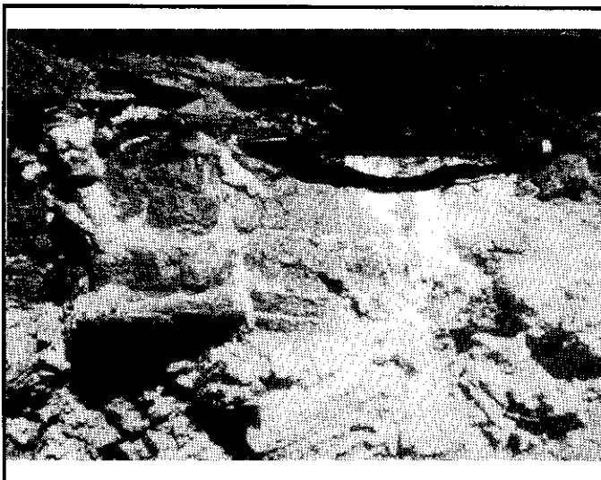
Figure 3. Quartz-filled tension fractures cutting massive sulphide at contact between rusty, brecciated limestone (above) and bleached phyllite (below). Note angular discordance between foliations above and below the sulphides.
