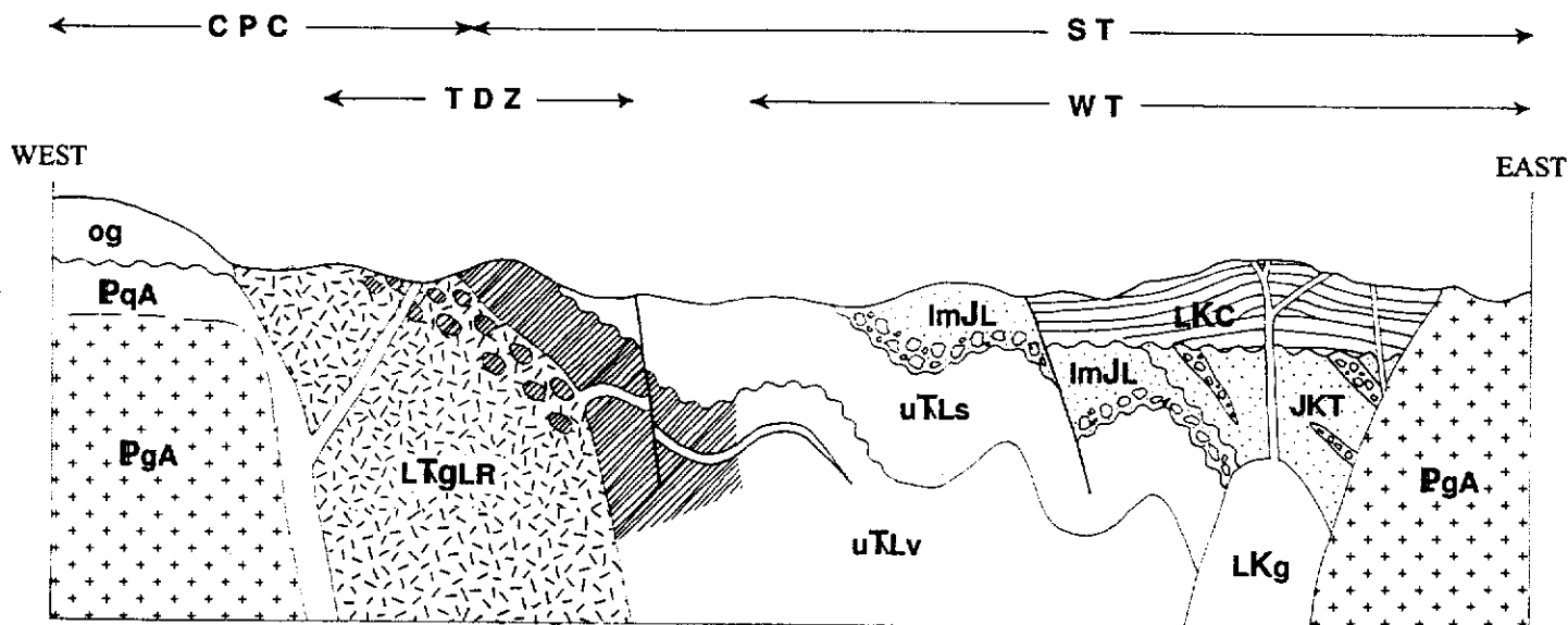
Figure 4. Schematic cross-section looking north, through the Thirty-seven Mile Creek map area (105D/13). Rock unit symbols are those used in Fig. 3. CPC = Coast Plutonic Complex, ST = Stikine terrane, WT = Whitehorse Trough, TDZ = Takhini deformation zone.
