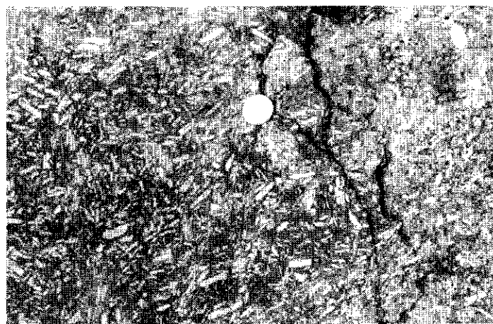
Figure 7. Large bladed plagioclase phenocryst, trachytic andesite porphyry flow. This unit is typical in the lower part of Late Cretaceous Carmack Group stratigraphy in southern Yukon Territory. Exploration and Geology 1992
