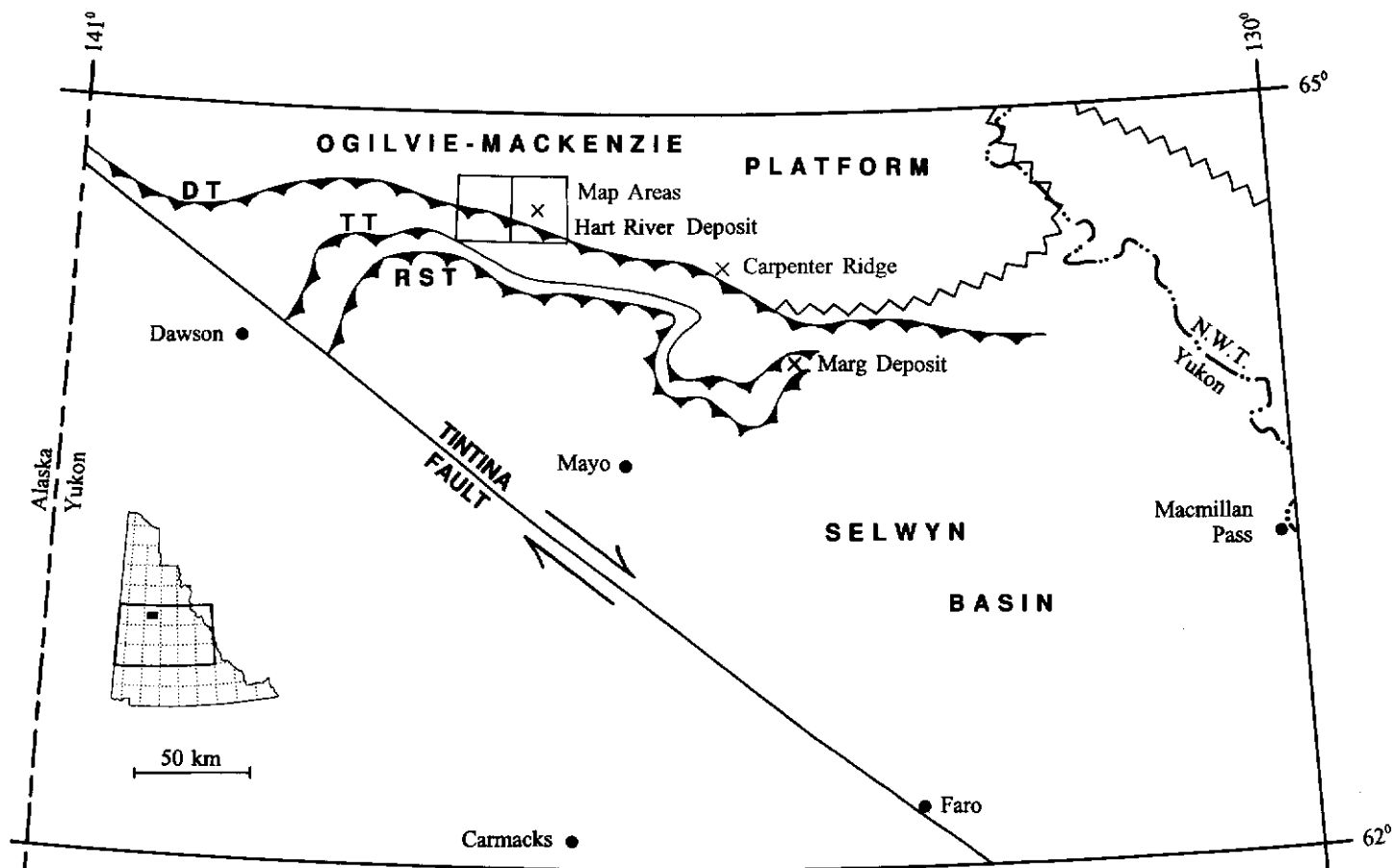
Figure 1. Tectonic setting and location of the study area. DT-Dawson thrust; TT-Tombstone thrust; RST-Robert Service thrust.
