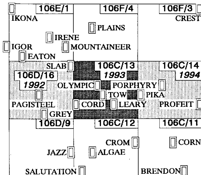
Figure 1: Wernecke Mountains Project—Location of study area and selected mineral occurrences in the Wernecke Mountains of northeastern Yukon. Darkly shaded area in centre is present study area, NTS map area 106C/13. Lightly shaded areas are former (1992) and proposed (1994) study areas. Occurrence names are from Yukon Minfile (INAC, 1993).
