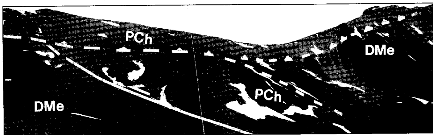
Figure 7: View south at Plata Thrust. Foreground Earn siltstone (DMe) is overthrust by folded Hyland limestone and maroon argillite (PCh). UTM 64635E, 705500N, 200 m SW of Plata #6 vein.
