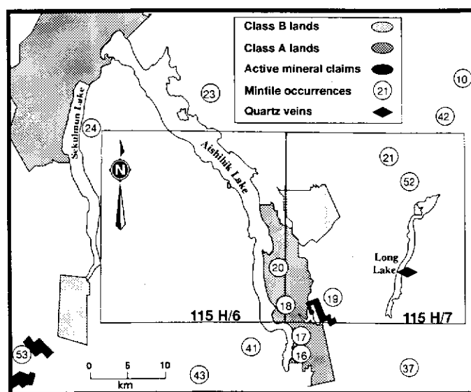
Figure 2: The location of Class A and B lands in the Aishihik Lake area. Also indicated are: Yukon Minfile occurrences (INAC, 1992); active claims as of June, 1993; the study area (map sheets 115 H/6 and 7); and the location of mineralized quartz veins mapped during this study. The quartz veins are described in the text. Assay results for these and other veins sampled during this study are included in Appendix 1.
