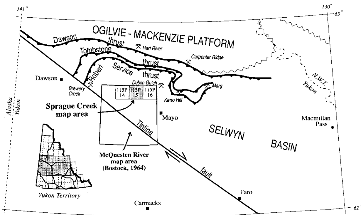
Figure 1: Location of Sprague Creek map area with respect to regional geographic and geological features and important mineral occurrences.
