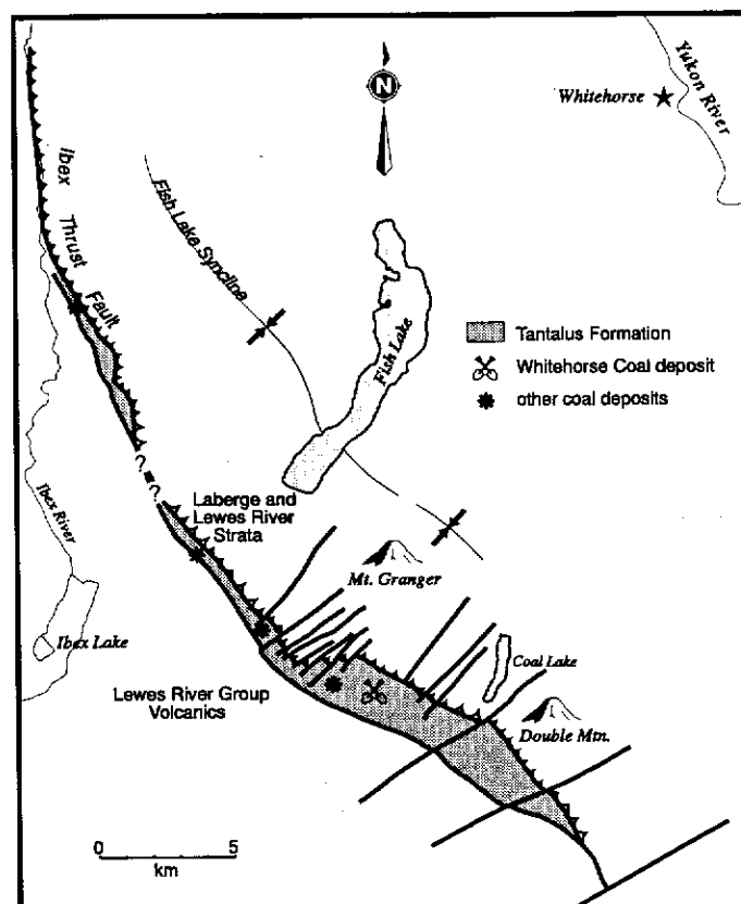
Figure 2. Location of the Whitehorse Coal Deposit.
