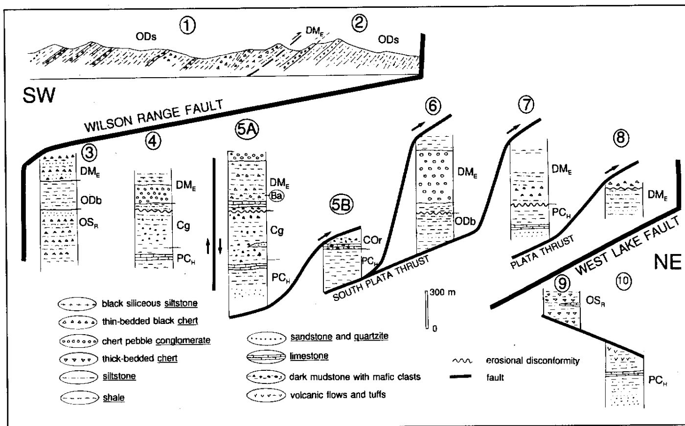
Figure 3: Generalized stratigraphic columns showing the main stratigraphic relationships in West lake map area.
