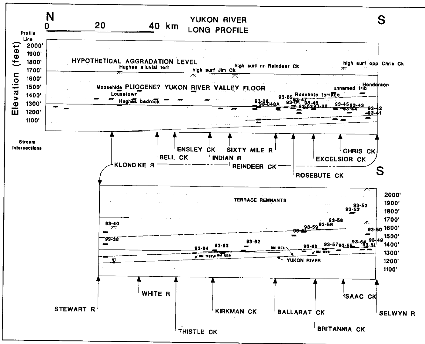
Figure 7: Long profile of Yukon River reach with terrace levels derived from field measurement, topographic maps, and data from Hughes and others (1972). A postulated aggradation level for the highest alluvial surface and a Pliocene? Yukon River valley floor are indicated as sloping opposite to the present drainage. A lower alluvial surface parallel to the present Yukon River slope is shown. A higher alluvial surface may have existed but data is scarce.
