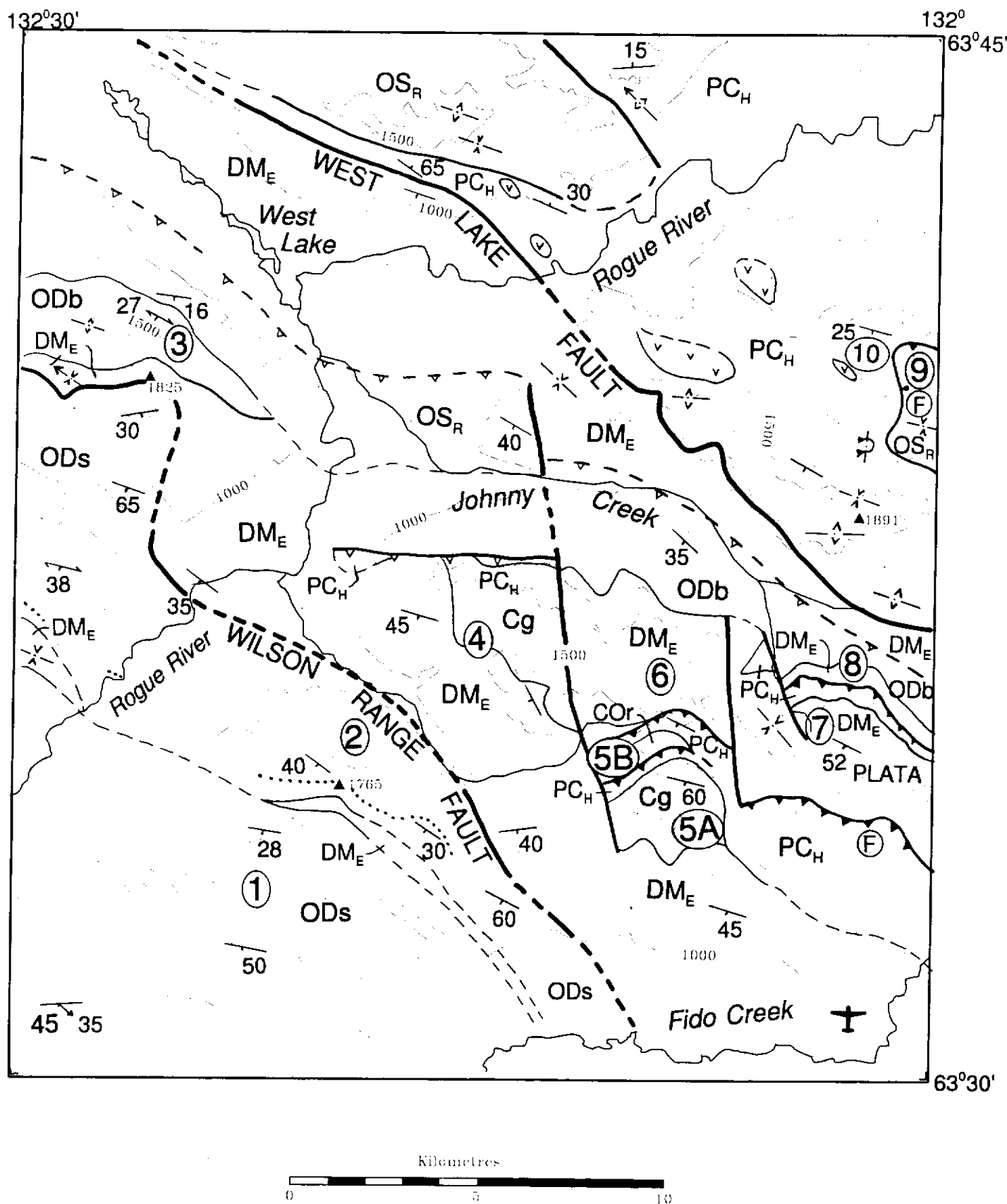
Figure 2: Simplified geological map of West Lake map area (105N/9). Numbers show the location of stratigraphic columns in Figure 3.
