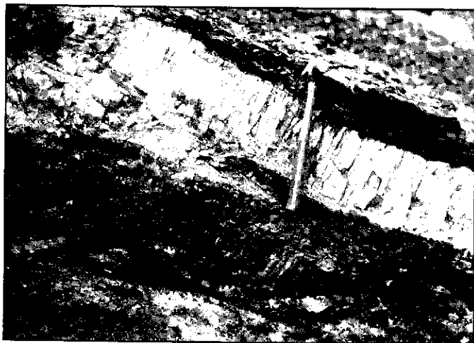
Figure 4a: A rhyolite sill cutting coal measures at the main pit of the Whitehorse coal deposit has resulted in adjacent columnar jointed coal and an increase in maturation due to metamorphism. See Figure 4b.
