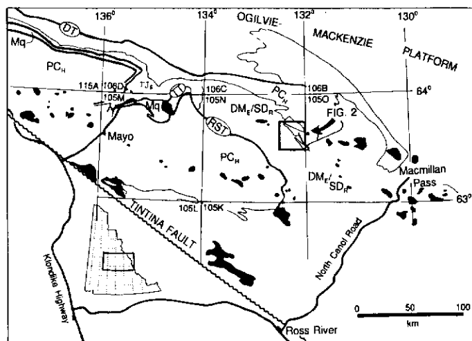
Figure 1: Tectonic setting and location of West Lake map area. DT-Dawson Thrust, TT-Tombstone Thrust, RST-Robert Service Thrust; Mq-Keno Hill quartzite, TJs-Lower schist and related rocks; DM_E/OS_R -Earn and Road River strata, PC_H -Hyland Group. Solid areas are Cretaceous granitic intrusions. Letters denote map areas, as follows: 1051: Nahanni (Gordey and Anderson, 1993); 105J: Sheldon Lake, and 105K: Tay River (Gordey and Irwin, 1987); 105M: Mayo (Roots and Murphy, 1992); 105N: Lansing (Blusson, 1974); 105O: Niddery Lake (Cecile and Abbott, 1992); 106C: Nadaleen River (Blusson, 1974); 106D: Nash Creek and 115A: Larsen Creek (Green, 1972).
