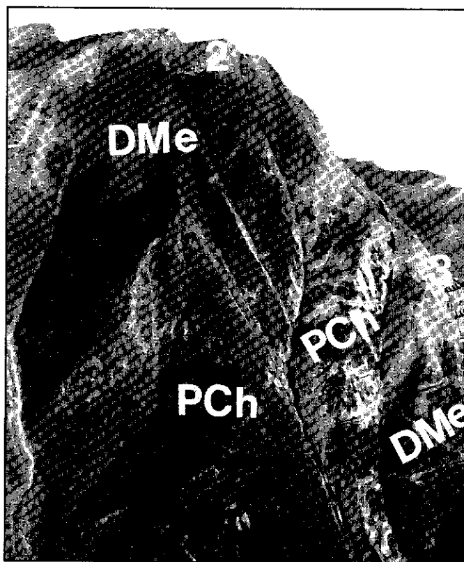
Figure 9: Aerial view looking northwest at the PLATA property. Numbers denote silver-lead veins that were mined between 1976 and 1985. Hyland Group (PCh) sandstone (foreground), limestone (near adit) and maroon argillite (middle right) are thrust over Earn Group (DMe) on right, and unconformably overlain by DMe (left). The normal fault in centre has about 100m south-side down displacement.
