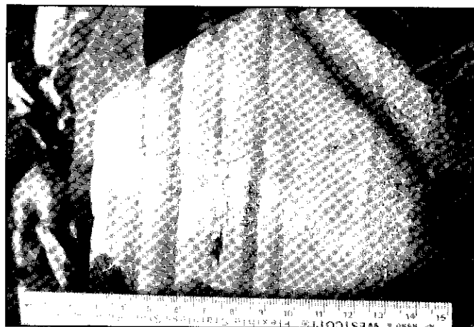
Figure 7: Thin-bedded turbiditic greywacke at top of mafic metavolcanic unit. Photo of boulder in southern tributary of Hobo Creek.
