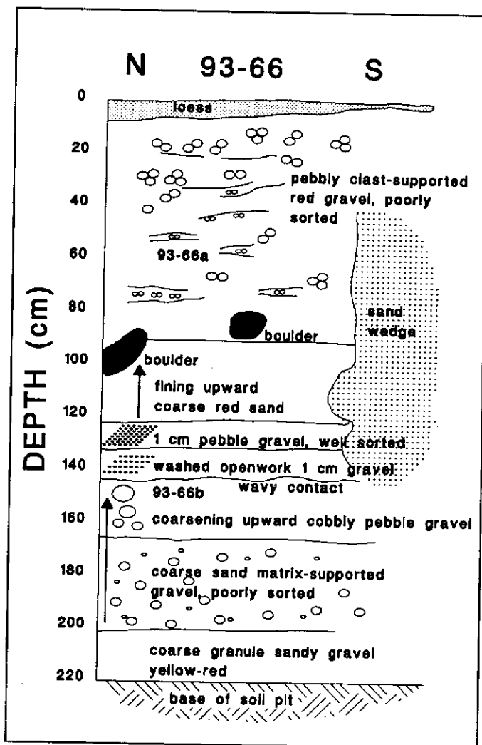
Figure 10: Schematic profile of soil pit with Wounded Moose paleosol from station 93-66, a 460 ft terrace opposite Lake Creek valley. Samples for gold grain counts are indicated (93-66a and 93-66b). This section is interpreted to be an outwash deposit related to the latest pre-Reid glaciation. The cross-cutting sand wedge is a cryogenic feature common in Wounded Moose paleosols.
