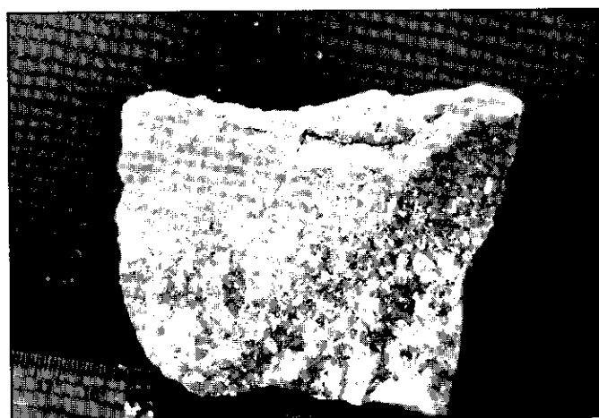
Figure 12: Cut surface of rock sample 93CH 11-2. This rock is a silicified and sulphidized granite from the northern margin of the Cap Creek Granodiorite. The grey patches and veins in this otherwise leucocratic rock is fine-grained accumulations of pyrite and chalcopryrite.
