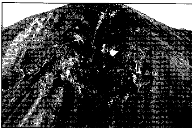
Figure 10: West (and east)-facing, steep rock faces such as this are common manifestations of the north-trending fault series. Although the mountain is composed of south-dipping Lewes River Group sediments, most of the resistant outcrops are composed of the numerous, north-trending felsite dykes which cut this face.
