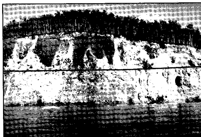
Figure 5: A rock cut terrace overlain by gravel and sand occurs five km downstream of Valley Creek on the right limit (stn 93-18). Black line marks the top of weathered bedrock at a height of 23 m (75 ft) above river level.
