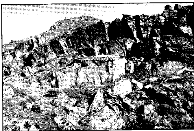
Figure 4: Medium-to thick-bedded meta-sandstone and pebbly meta-sandstone and interbedded phyllite of Narchilla Formation. View is to the west along the ridge east of summit of Red Mountain.
