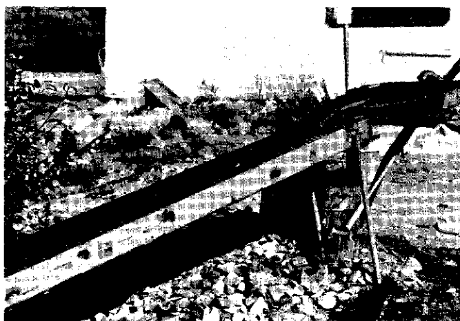
Figure 38: Small sluice box, or "long tom" used to upgrade sluice box concentrates. Expanded metal and astroturf cover the floor of this unit.
