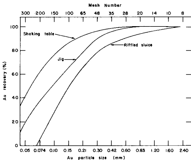
Figure 6: Recovery rates of fine-grained gold for sluice box, jig, and shaking table (after Wang, 1979).
