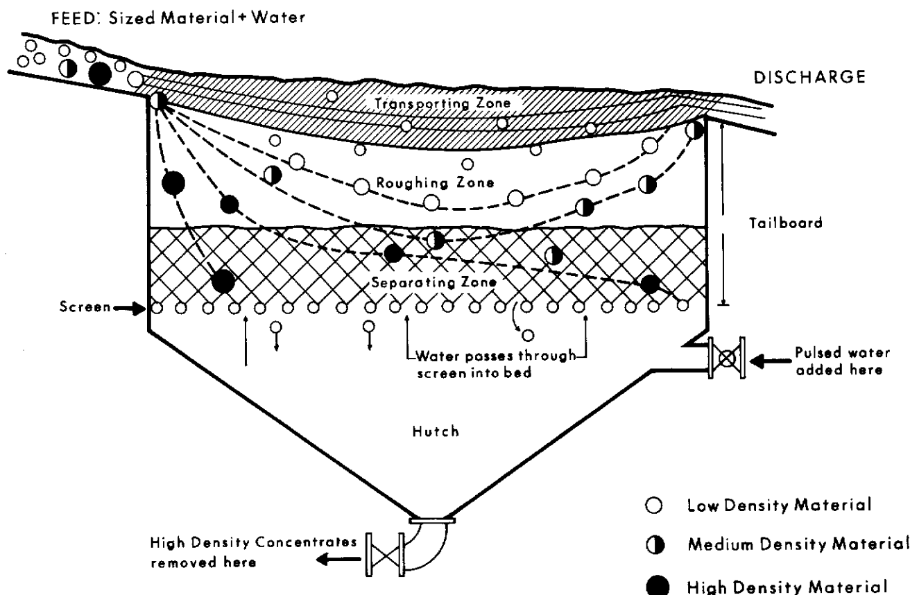
Figure 4: Cross-sectional diagram of a jig, showing the paths of particles of various densities.
