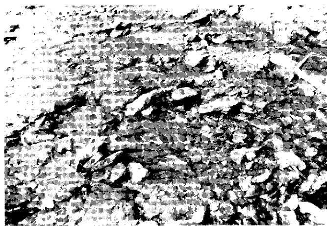
Figure 10: View of imbricated clasts in a shallow stream.
