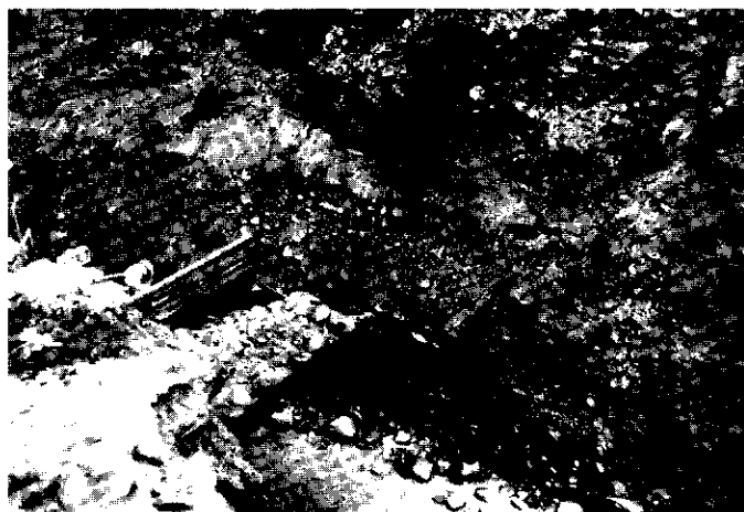
Deposits at the Russell Creek property of Noranda Exploration Ltd. Glaciofluvial gravel, massive clay and a second horizon of glaciofluvial gravel are visible in the wall of this test pit. The loader bucket at the left of the photograph provides a scale.
