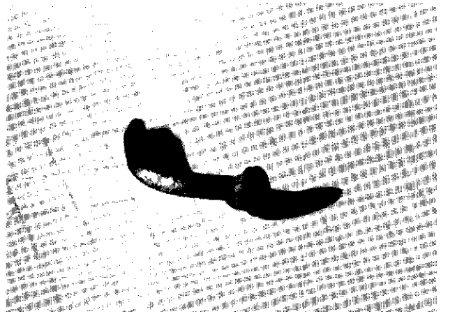
Figure 28: Copper nail recovered from old underground workings on Miller Creek. A thin plating of gold covers the convex side of the bent nail. The spaces on the grid paper are 5 mm (.2 inches) apart.
