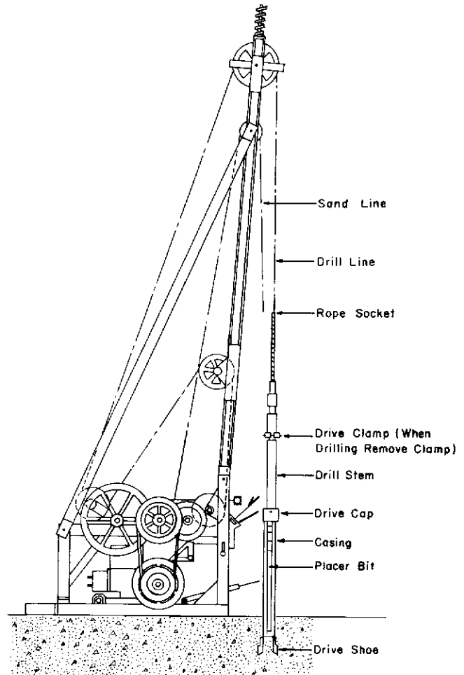
Figure 1: Basic equipment used in churn drilling (after Wells, J.H., 1973).
