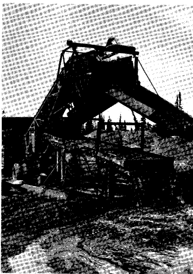
Figure 15: "Over-and-under" sluicing plant used along the right limit of Indian River by Alcar Construction Ltd. (R.W. '84)
