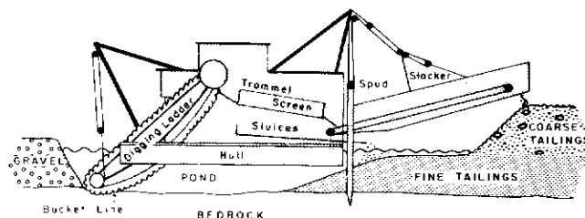
Figure 1: Diagram showing the parts of the Queenstake Resources Ltd. dredge.
