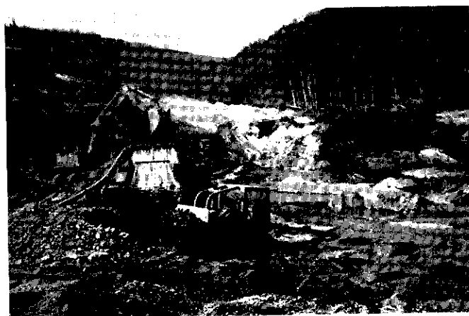
Figure 21: Sluicing plant at LRL Mining being fed by the Cat 235 hoe. Tailings are being removed from the foot of the "Derocker" screening unit by the Traxcavator. (L.O. '83)
