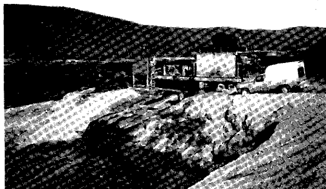
Figure 12: Sluicing plant being fed by loader at Teck Corp. mining operation on Sulphur Creek. (R.W. '84)
