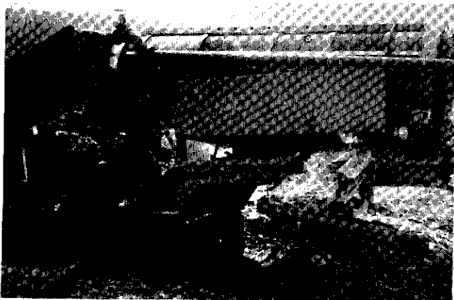
Figure 4: Sluicing plant used by D. Sandberg at the base of Paradise Hill. (L.O. '83)
