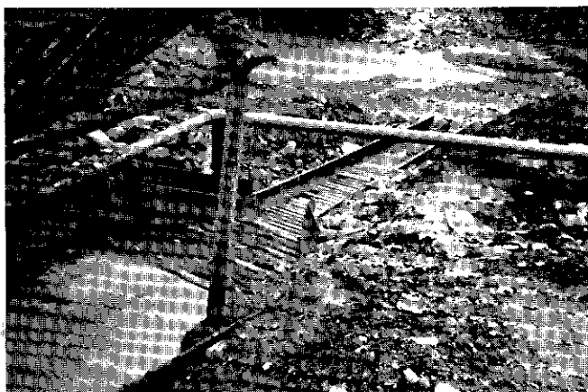
Figure 1: Sluicing plant at A. Ritter and F. Schomig operation on Fifteen Pup. Grizzly is visible at upper left above dump box. (R.W. '83)
