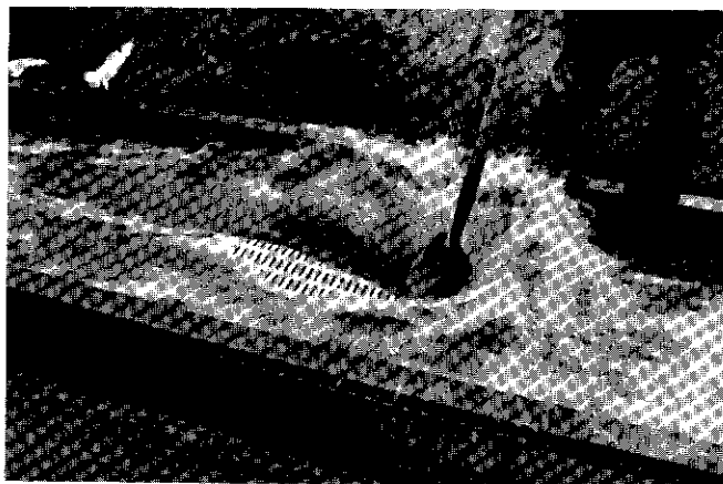
Figure 1: Slotted punch plate over riffles in a single run sluice box. (J.H. '84)
