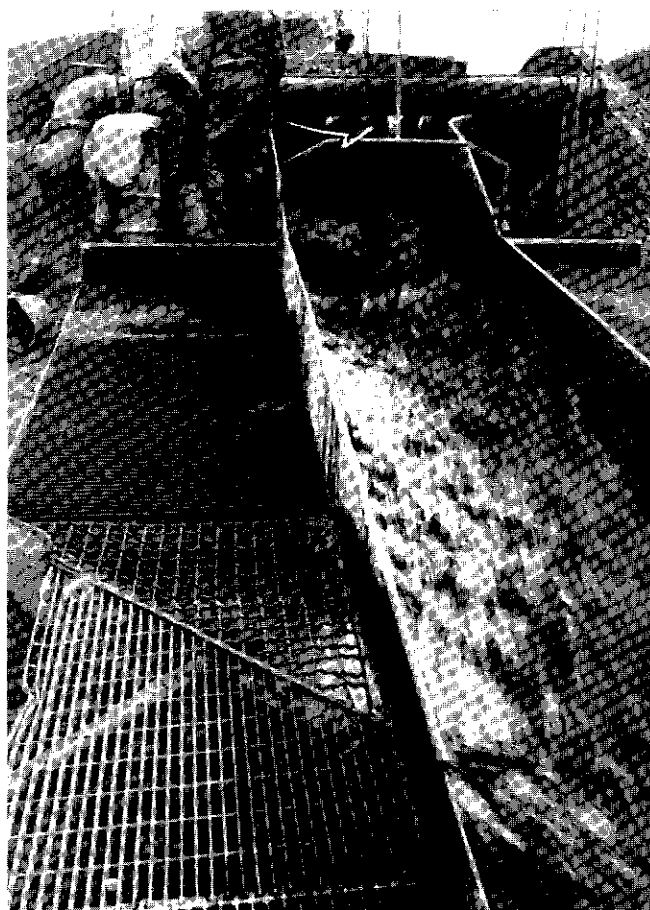
Figure 14: Sluicing using a sluice box with main run and two short side runs. Water is being sprayed from a manifold onto the gravel in the dump box. (J.H. '84)
