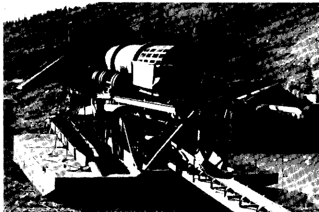
Figure 2: View of "Hall Dredge" sluicing plant used by Burwash-Cooper Mining Co. Ltd. on Burwash Creek. The pontoon hull of the unit is visible. (L.O. '84)
