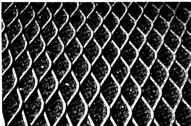
Figure 4: Thick gauge expanded metal overlying indoor-outdoor carpet. Heavy minerals trapped by the riffles can be seen.
