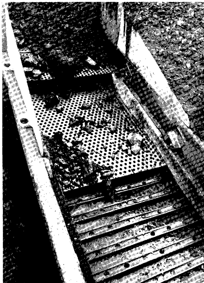
Figure 5: Punch plate over angle iron riffles with holes along the top. (J.H. '84)
