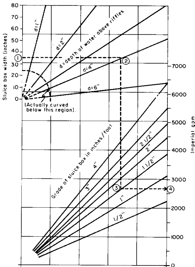
Figure 6: General guide to the amount of water used per minute in a sluice box.
