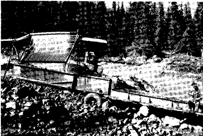
Figure 2: Single run sluice box with grizzly typical of those used in glaciated areas. (J.H. '84)
