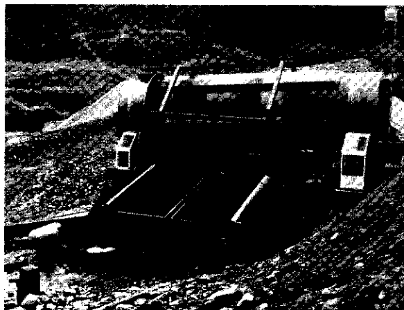
Sixty Mile Enterprise's trommel with double side runs, located on Miller Creek.
