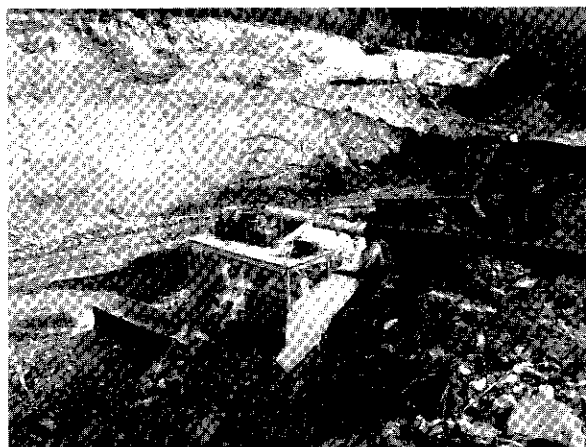
Homemade derocker at Johnson Creek mining operation of R. Barchen being fed by a loader.
