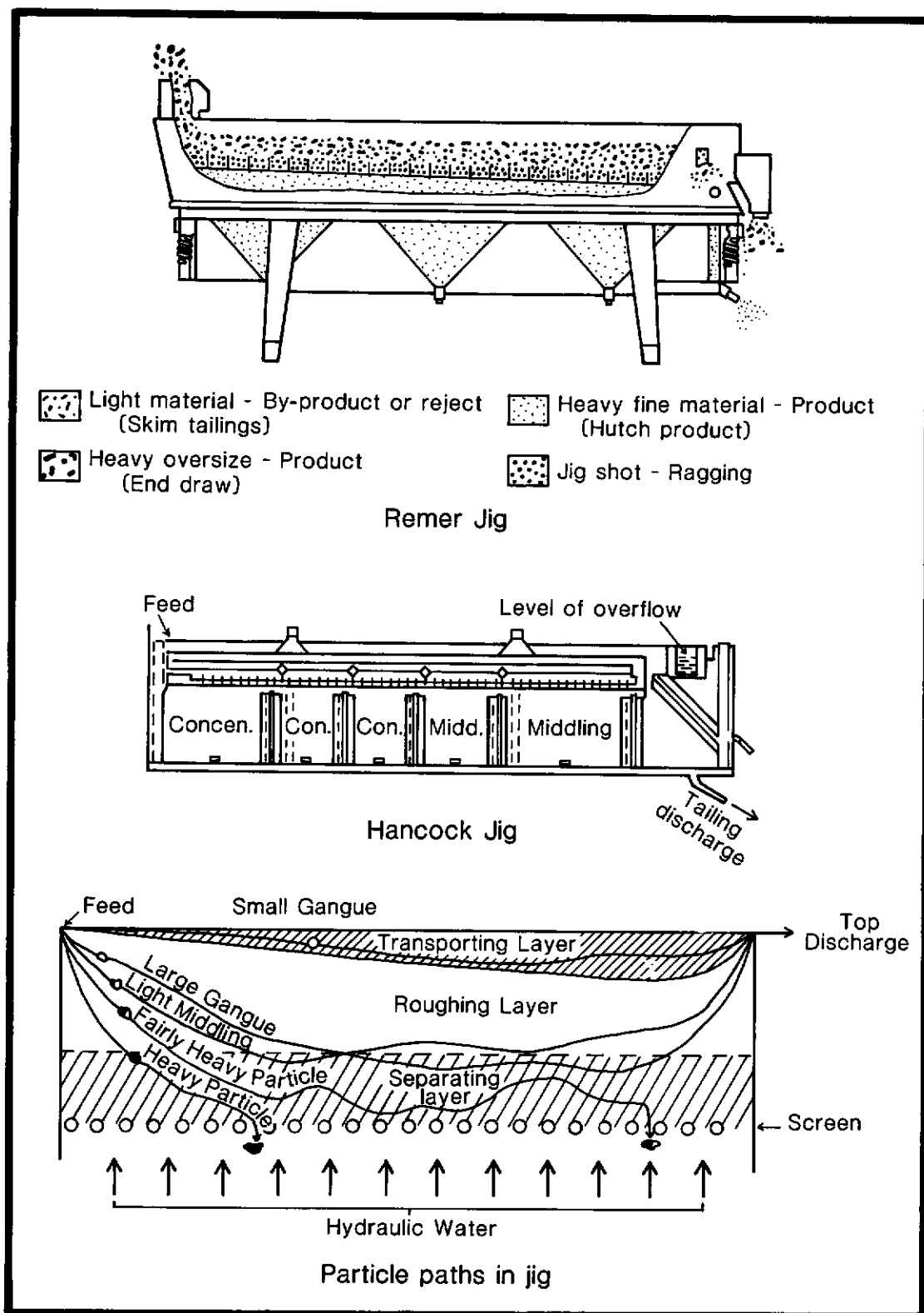
Figure 4: Jig operation (Pryor, 1965).
