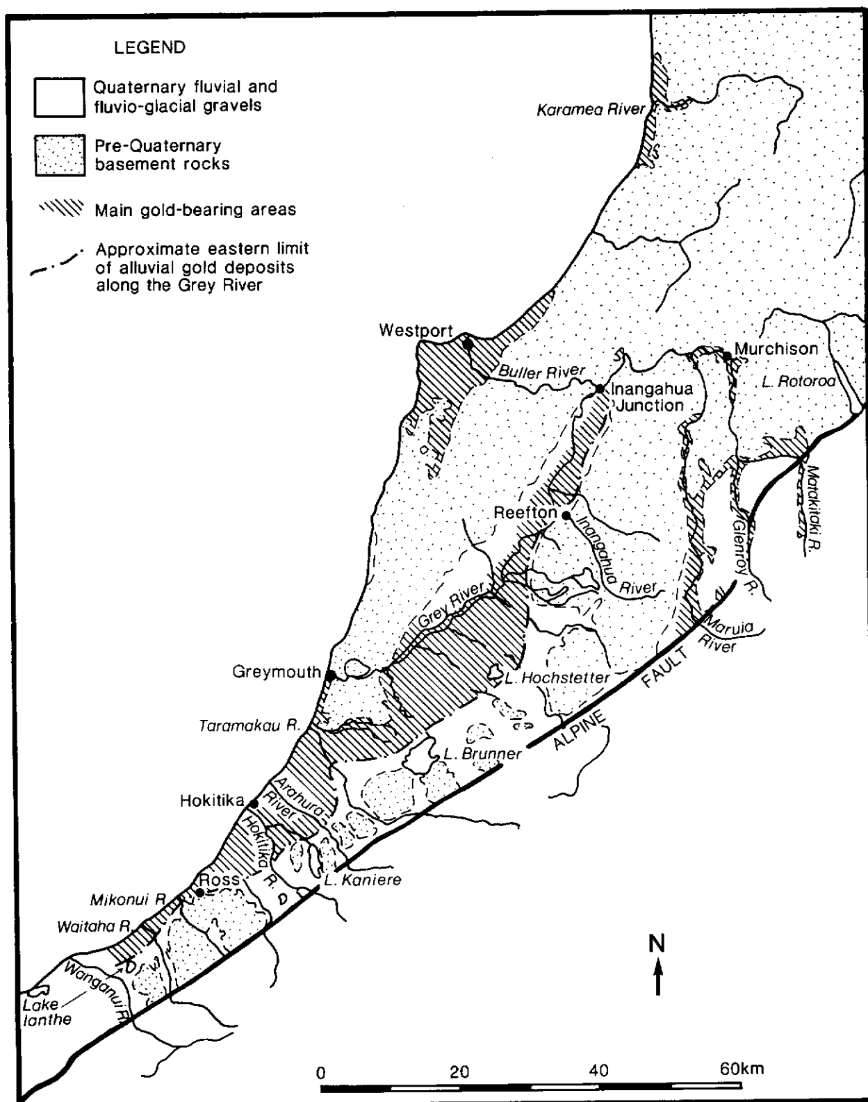
Figure 1: Distribution of West Coast alluvial gold deposits.
