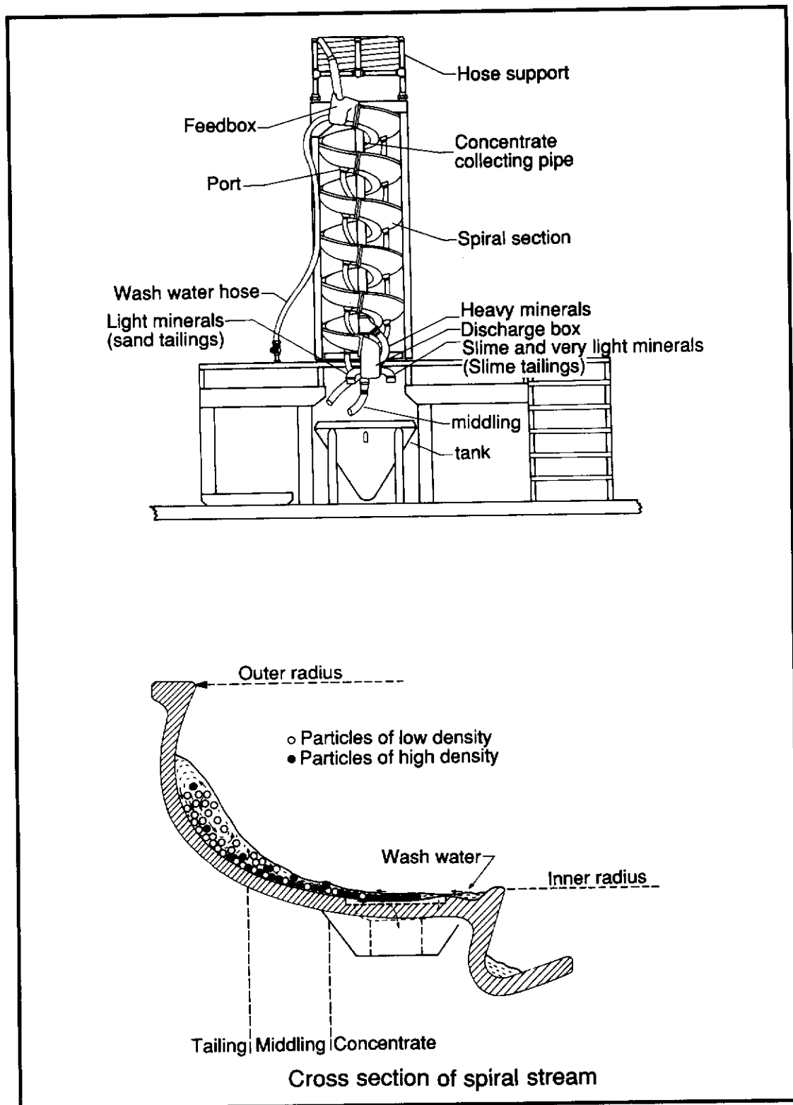
Figure 5: Spiral operation (Pryor, 1965).
