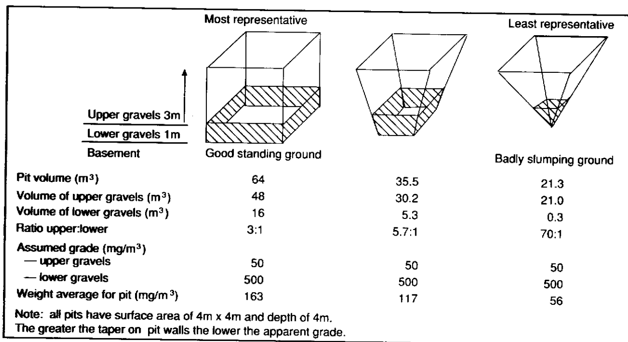
Figure 3: Effect of pit shape on sample volume and calculated gold grade.
