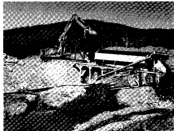
A 225 Cat hoe is feeding a hopper at the head of the trommel, at Queenstake's placer operation on Blackhills Creek.
