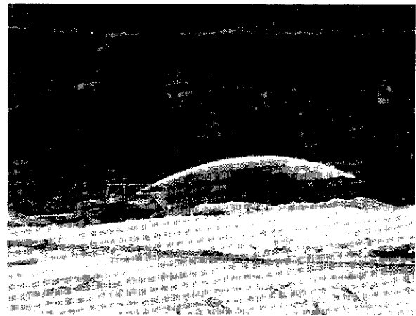
Hydraulic at J & C Holding's property on Hunker Creek. Water was used to strip a thick section of black muck.
