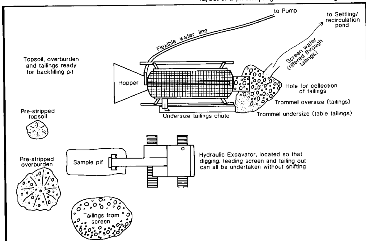
Figure 2: Sample pit optimum ground plan layout.
