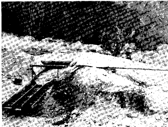
View of a typical 3 run sluice box, at Hans Algotson operation on Trail Hill.
