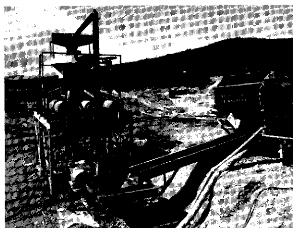
View of trommel wash plant operated by Nechako Contracting, with side sluice run feeding material to Cyclones on Clear Creek.
