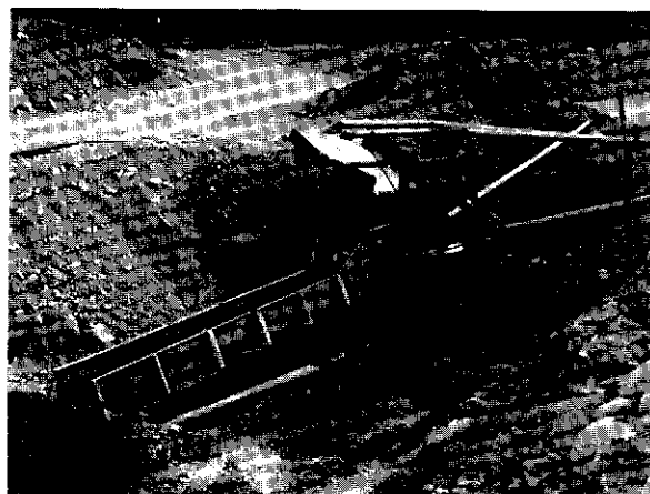
Sluice plant with side dump hopper grizzly at Larry Tremblay's property on Reed Creek.
