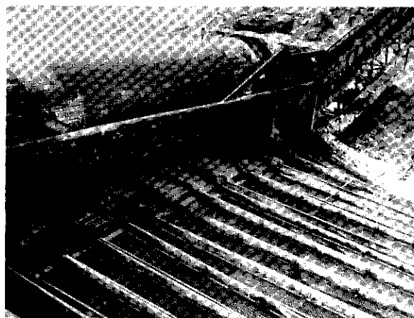
M. Orbanski's 8 foot diameter trommel with 12 sluice runs which was located at the mouth of Bonanza Creek right limit.
