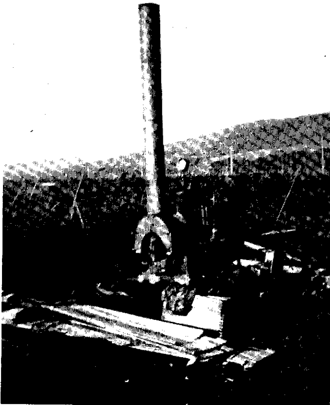
The steamer on the left, used to thaw ground on Granville in 1935, is not much different from the steamer on the right, which found service on Revenue Creek in 1992.
