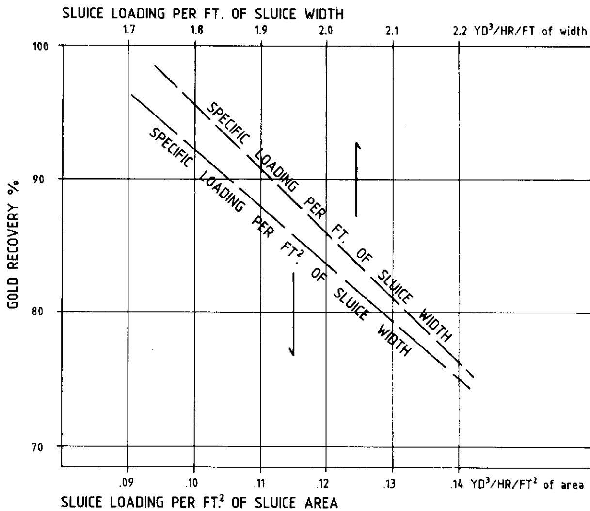
TYPICAL DETERIORATION IN SLUICE PERFORMANCE WITH INCREASED LOADING
