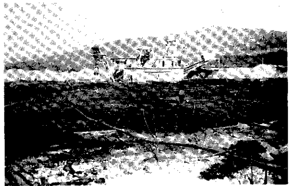
View of steam pipes and points used in thawing the ground in preparation for the dredge in the background (circa 1935).
