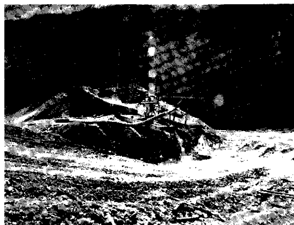
A triple run sluice box with monitor at J&C Holding's mine on Hunker Creek.
